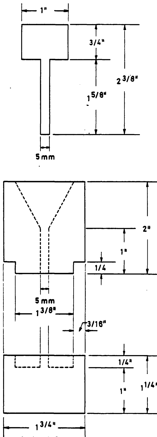
Figure 15. Press design B for preparing graphite powder compacts.
