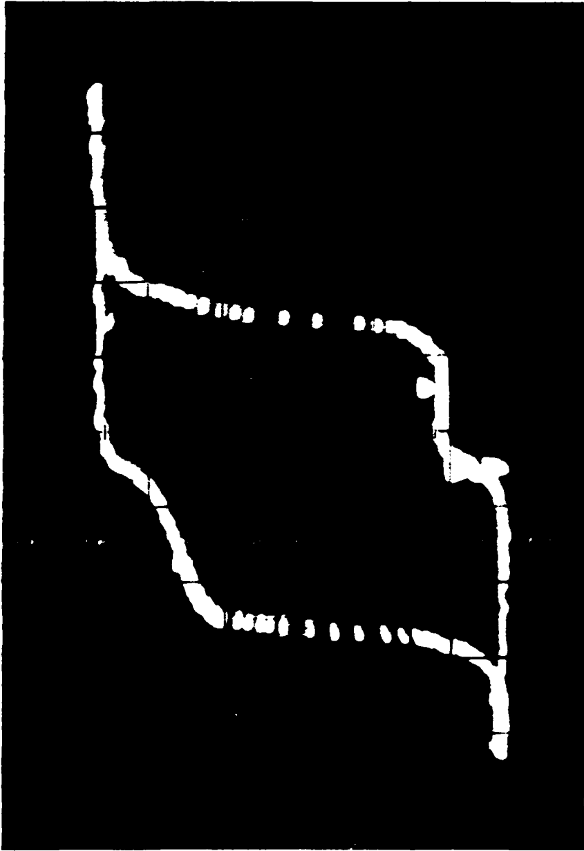
Fig.17: M(H) of "Neomax" at T = 77K
