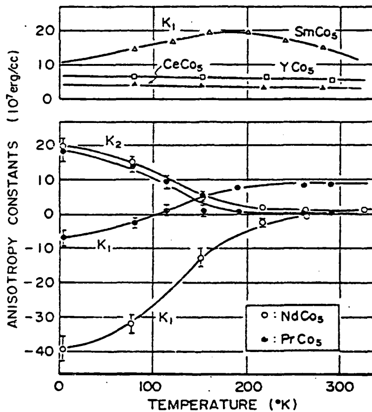
Fig.14: K_1(T) and K_2(T) for \text{YCo}_5 , \text{SmCo}_5 , \text{NdCo}_5 and \text{PrCo}_5 according to (21)
