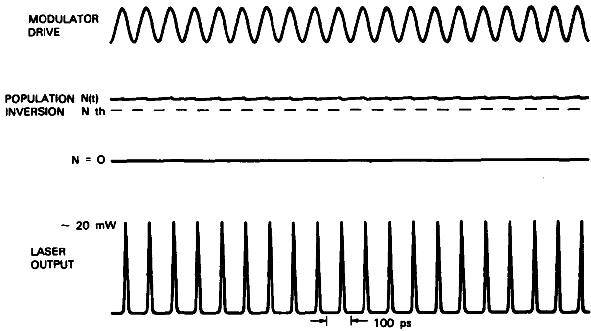
Figure 3. Continuous-inversion Q-switching at 10 GHz for I = 1.65 I_{th} , \tau^{SP} = 1.5 ns, \alpha^L = 50 cm -1 , \alpha^H = 350 cm -1 , C = 10^{-5} , a 180- \mu m amplifier, and a 70- \mu m modulator.
