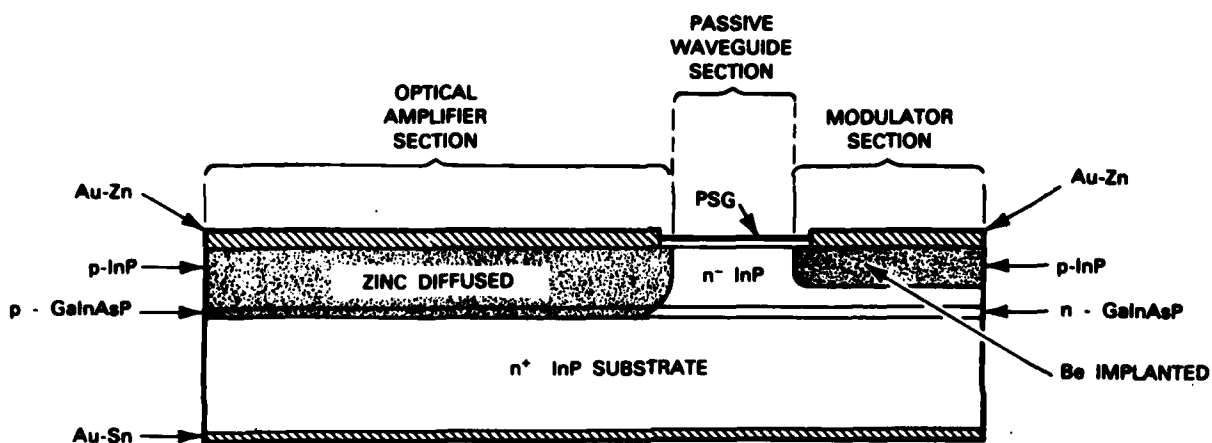
Figure 1. Schematic drawing of the laser cross section. The optical amplifier and modulator range in length from 150 to 200 \mu\text{m} and 50 to 75 \mu\text{m} , respectively. The waveguide is 25 \mu\text{m} long. A mesa (not pictured) is etched to provide lateral optical confinement. The endface mirrors are formed by cleaving.
