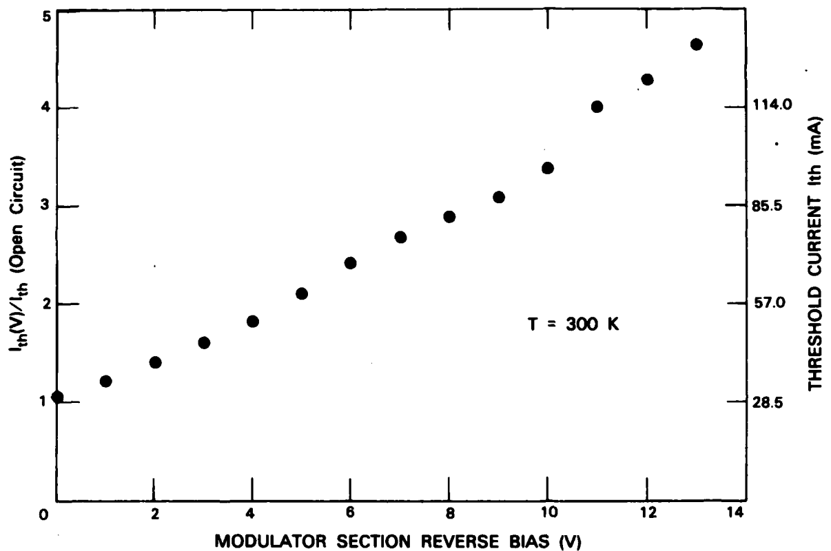
Figure 13. Pulsed threshold, normalized to the threshold of the laser with the modulator open, as a function of modulator reverse bias.
