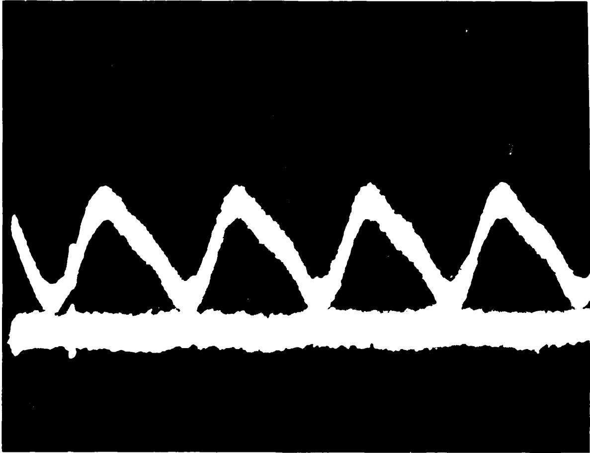
Figure 10. Q-switched output at 3 GHz from the laser with proton-isolated modulator. Modulator is forward-biased and operates by both gain and loss switching.
