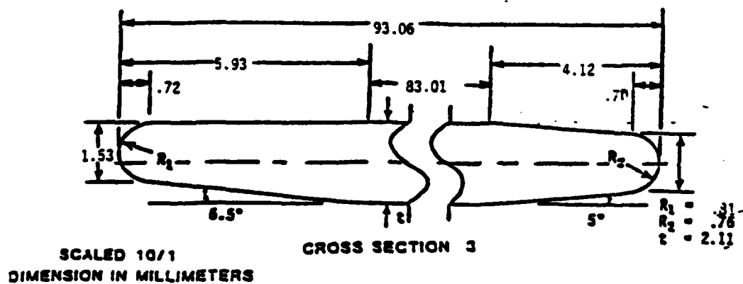
Figure 1c. Cross Sectional Drawings of the Steel Fin
