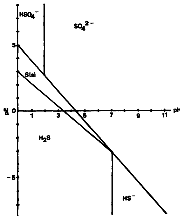
Figure 9. pE-pH Diagram for the \text{SO}_4^{2-} - \text{S(s)} - \text{HS}^- System (Reference 18)
