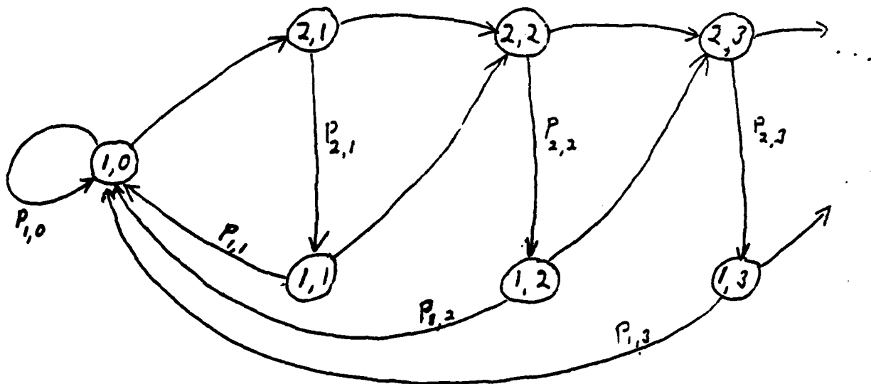
MARKOV CHAIN FOR COLLISION RESOLUTION PERIOD
