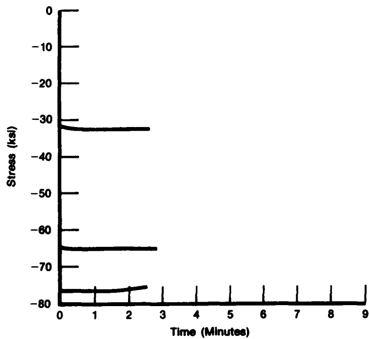
Figure 2-16. Relaxation Curves Starting from Points on Compression Unloading Branch in Figure 2-4
