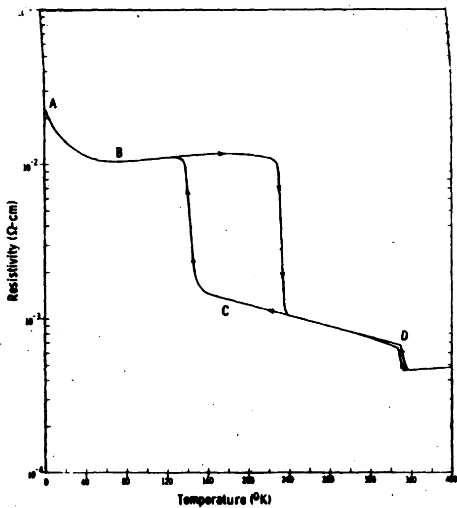
Figure 1. The logarithm of the resistivity of 1T TaS 2 versus the temperature.
