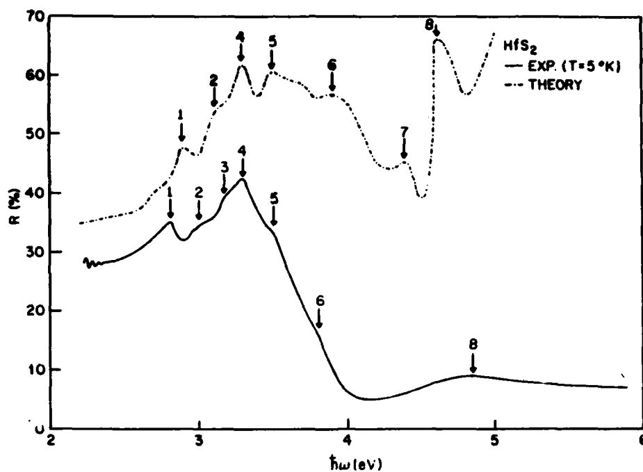
Figure 6. Experimental and theoretical spectra of \text{HfS}_2 .
