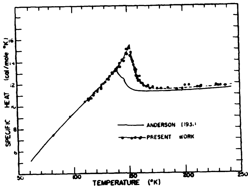
Figure 1. Specific heat of \alpha -MnS in the vicinity of the Neel temperature.
