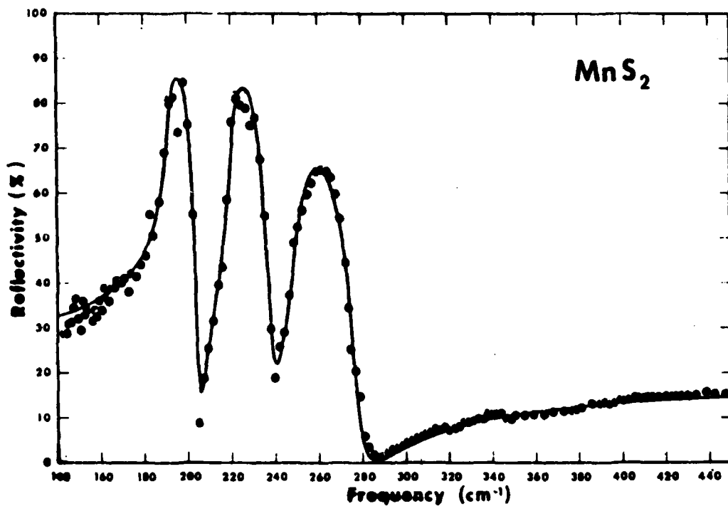
Figure 3. Three oscillator fit to the infrared reflectivity of \text{MnS}_2 . The points are the experimental data and the curve is the theoretical fit.
