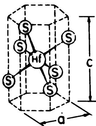
1T-HfS 2
