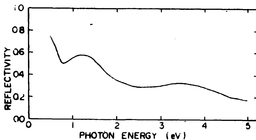
Figure 1. Reflectivity spectrum of a \text{CoS}_2 single crystal at room temperature.
