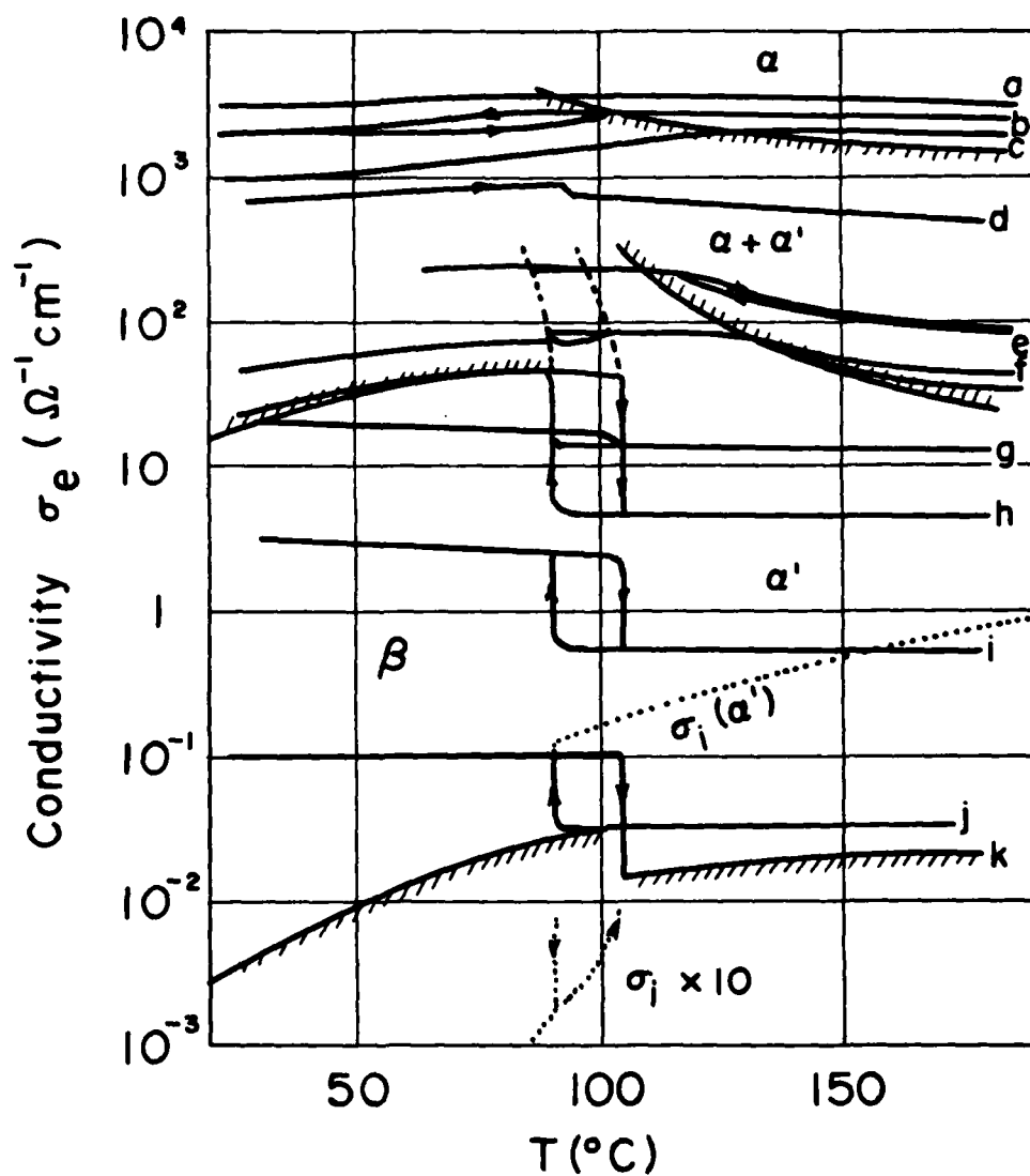
Fig. 1 \sigma_e vs. T FOR \text{Cu}_{2-\delta}\text{S} CORRESPONDING TO FIGURE 2.
