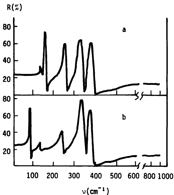
Figure 4. Infrared reflection spectra of \text{CdGa}_2\text{S}_4 : (a) \vec{E} \parallel \vec{c} ; (b) \vec{E} \perp \vec{c} .
