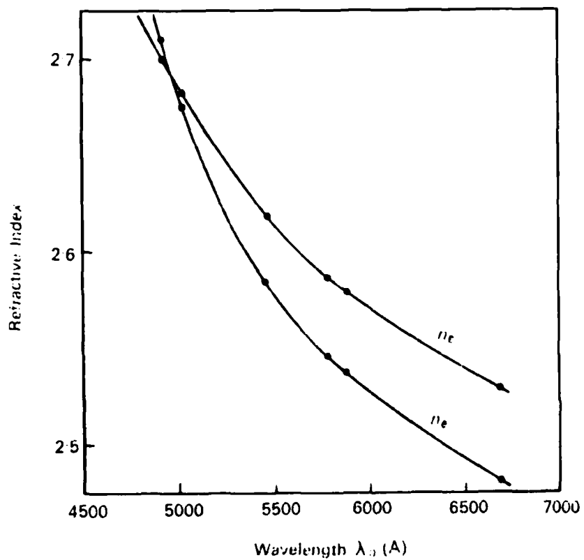
Figure 1. The refractive indices of AgGaS 2 at 20°C.
