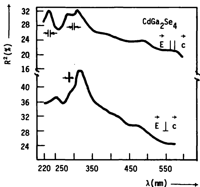
Figure 3. Spectrum of twofold reflection of \text{CdGa}_2\text{Se}_4 in polarized light.
