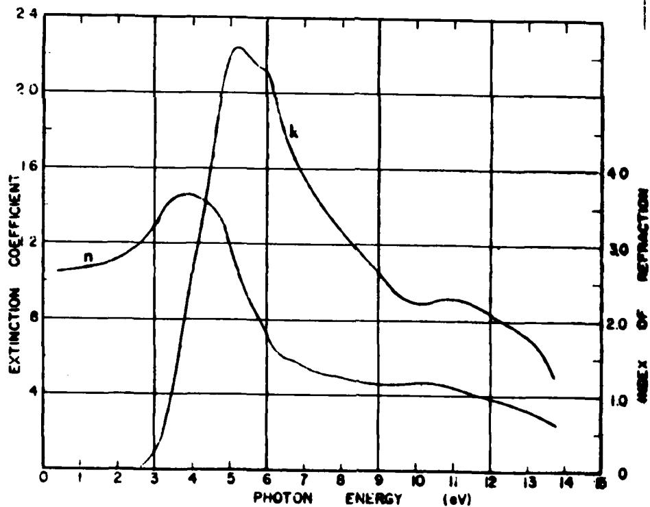
Figure 14. Spectral dependence of the real and imaginary parts of the refractive index calculated from reflectance data.
