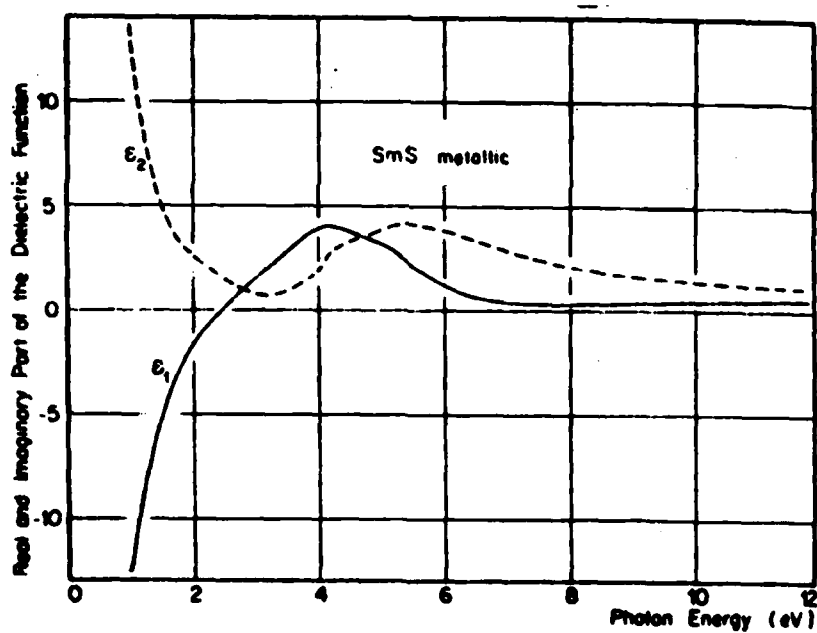
Figure 5. Dielectric function of metallic SmS.
