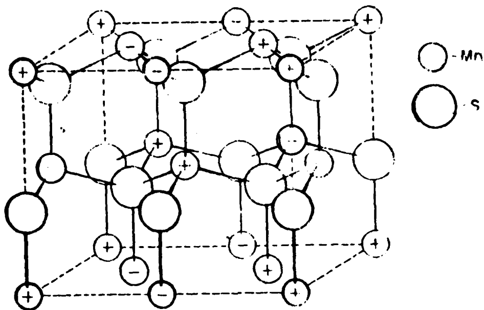
Figure 4. Magnetic structure of \beta -MnS (wurtzite form). The orthorhombic unit cell is shown.
