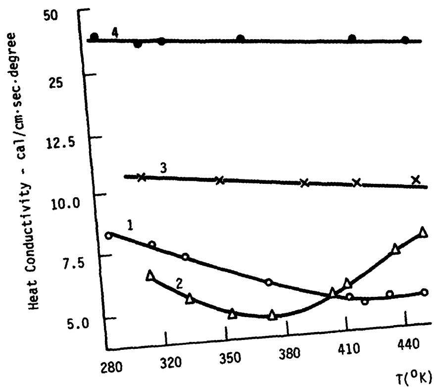
Figure 2. Effect of temperature on the heat conductivity of Ag 2 Te (1), Ag 2 Se (2), SnTe (3), and CdTe (4).
