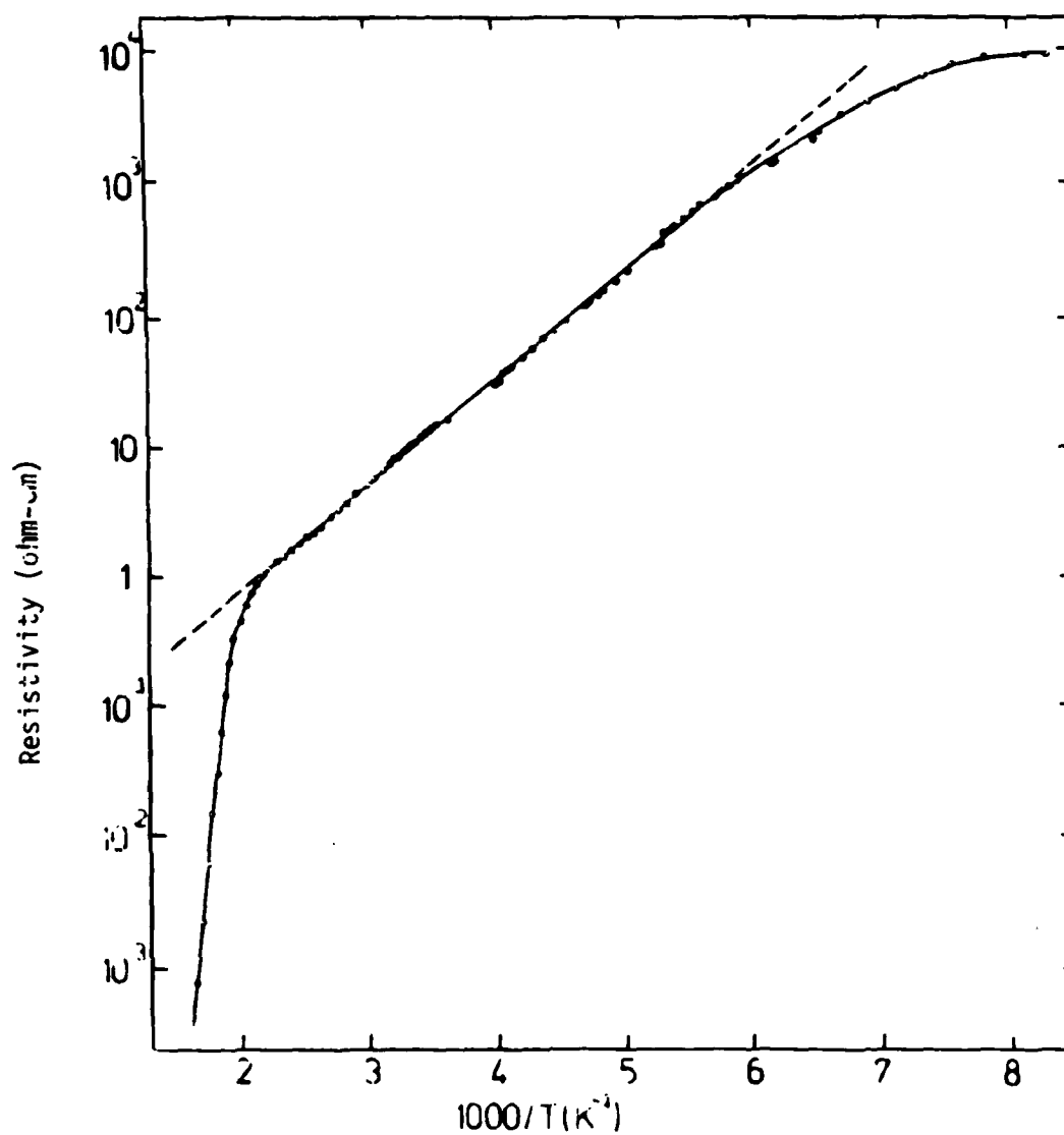
Figure 6. Temperature dependence of the resistivity \rho of a single crystal of \alpha -MnS, grown by iodine-vapor transport and quenched from 600K.
