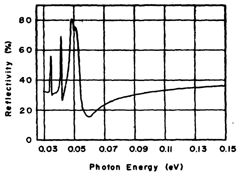
Figure 4. Spectral reflectivity of FeS 2 at 300 0 K in the infrared region.
