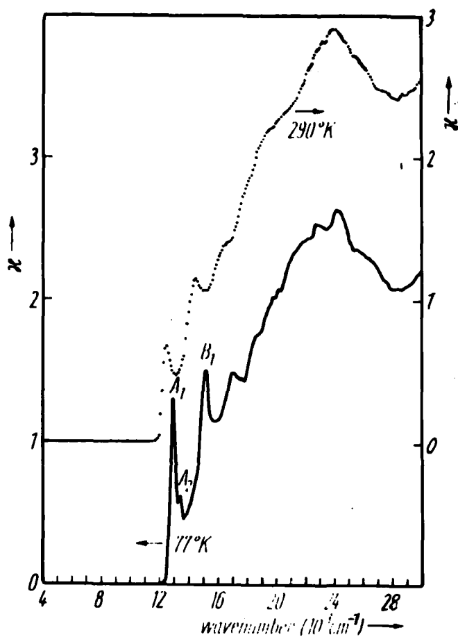
Figure 5. Spectral variation of n ( \vec{E} \perp \vec{c} ) for \alpha\text{-MoSe}_2 at 290^\circ (dotted) and 77^\circ\text{K} (full line).
