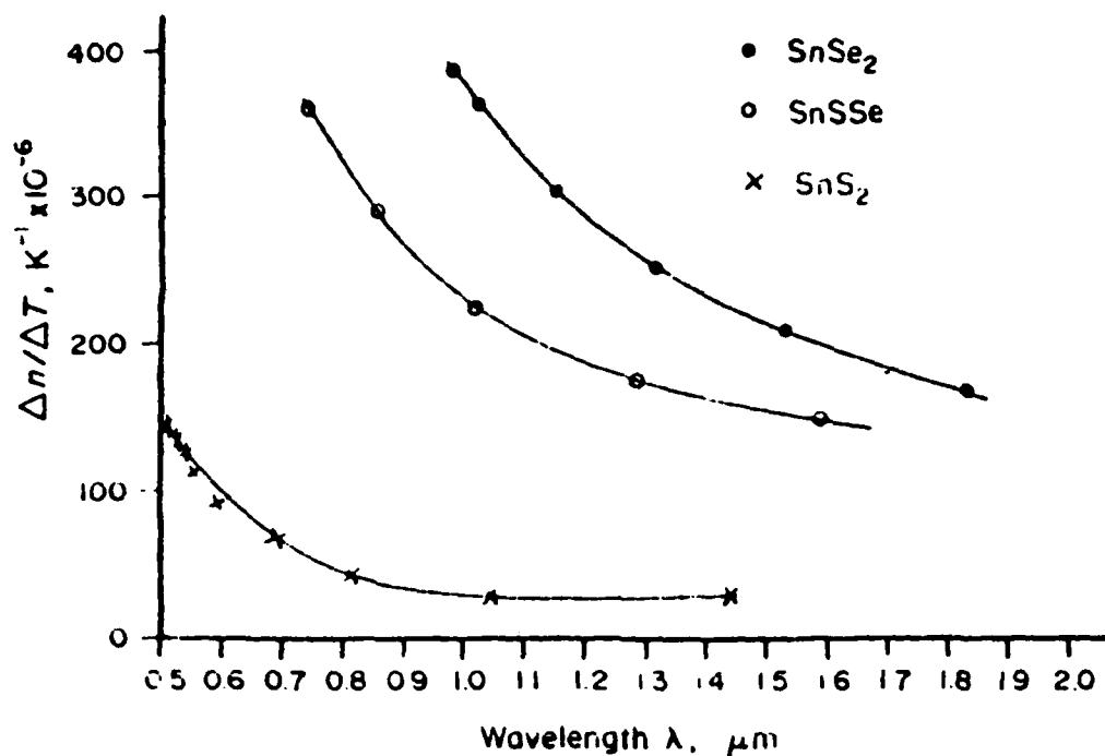
Figure 3 - The temperature coefficient of the refractive index as a function of the wavelength for SnS_xSe_{2-x} ( x = 0, 1, 2 ).
