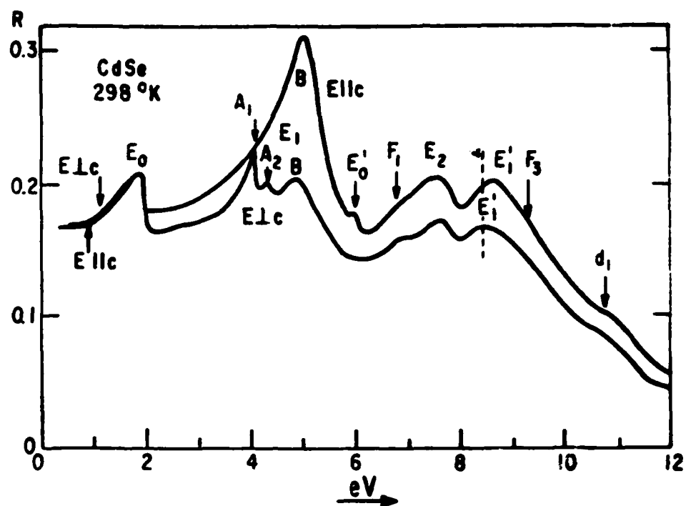
Figure 1. Reflectance of CdSe at room temperature.
