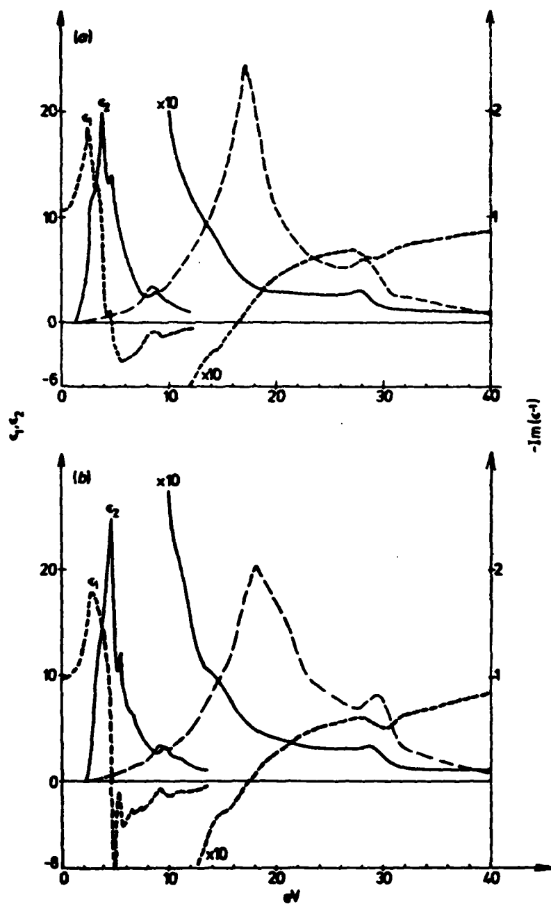
Figure 7. Dielectric constants ( \epsilon_1, \epsilon_2 ) and energy-loss function (unlabelled broken curve) of (a) \text{SnSe}_2 and (b) \text{SnS}_2 .
