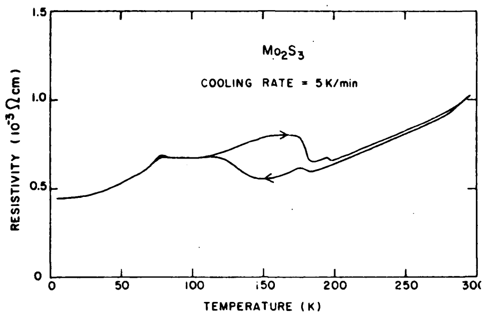
Figure 2. Resistivity of \text{Mo}_2\text{S}_3 as a function of temperature. The cooling rate was approximately 5^\circ\text{K/min} .
