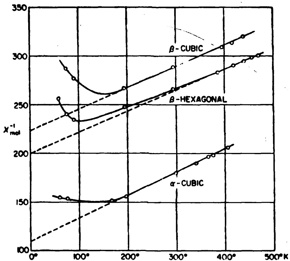
Figure 2. Magnetic susceptibility of MnS as a function of temperature.
