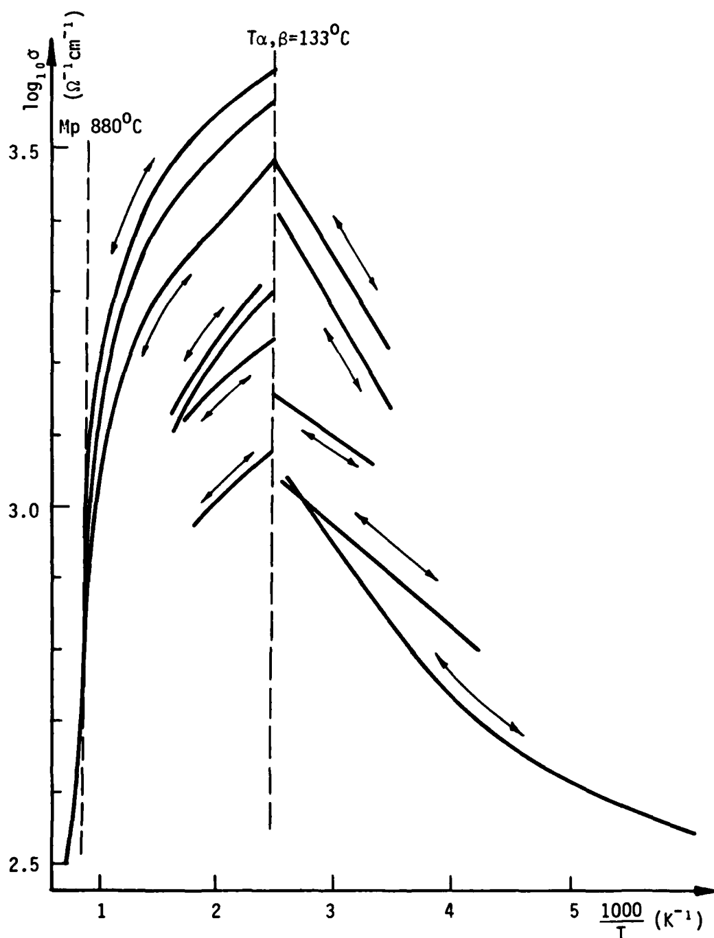
Figure 1. Electrical conductivity of \text{Ag}_2\text{Se} . For T < T_{\alpha,\beta} = 133^\circ\text{C} , all the measured samples demonstrate semiconducting properties. For T > T_{\alpha,\beta} , the coefficient d\sigma/dT is always < 0 . The different curves, corresponding all to nominally pure and stoichiometric samples, demonstrate the influence of thermal history on the electrical conductivity of \text{Ag}_2\text{Se} .
