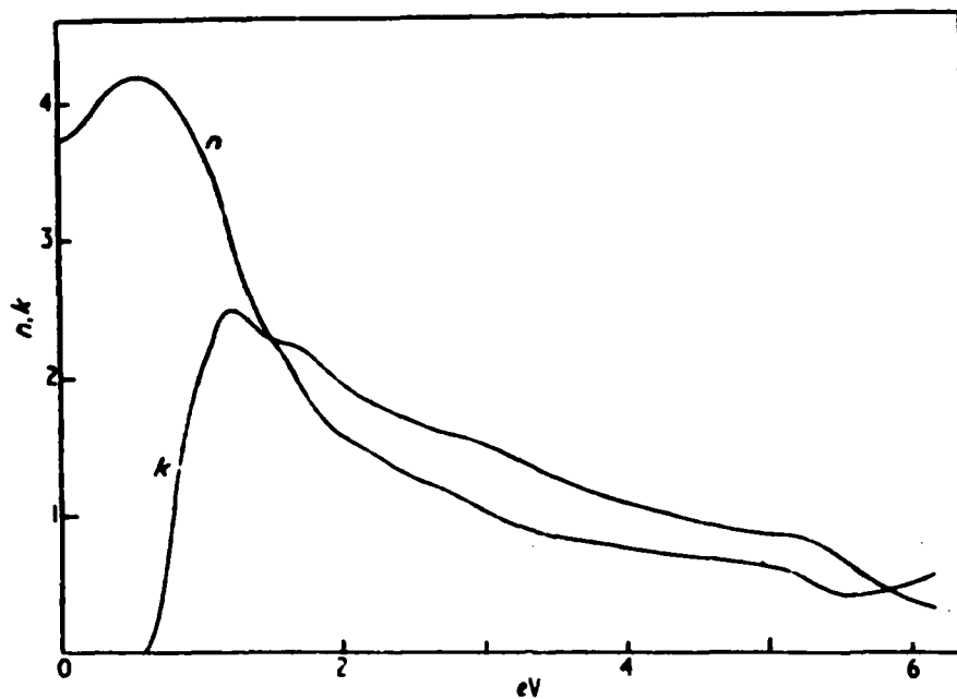
Figure 5. Real and imaginary parts of the refractive index n and k of \text{MoTe}_2 from Kramers-Kronig analysis.
