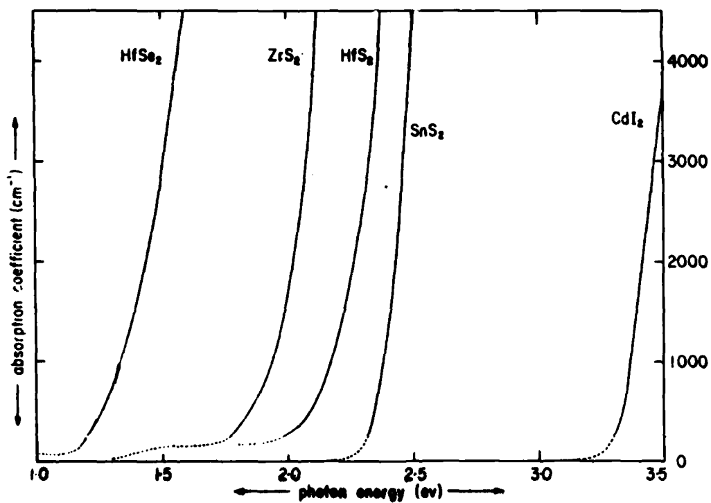
Figure 7. Room temperature optical absorption edge data for \text{ZrS}_2 , \text{HfS}_2 , \text{HfSe}_2 , \text{SnS}_2 and \text{CdI}_2 .
