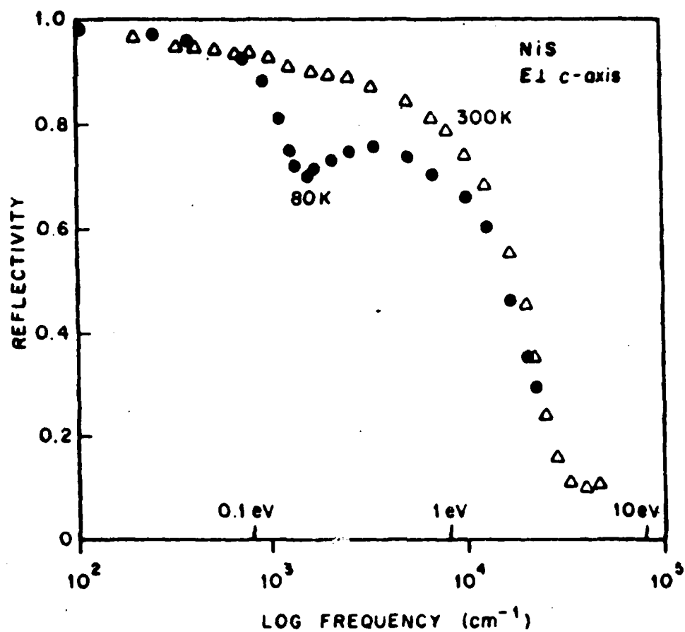
Figure 5 - Polarized reflectivity spectra for a sample of NiS taken above and below the transition temperature of 230 0 K.
