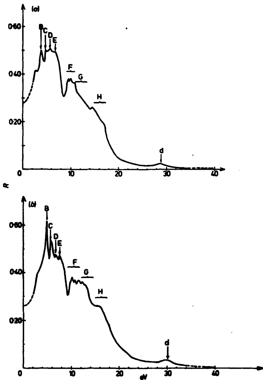
Figure 6. Reflectivity curve of (a) \text{SnSe}_2 and (b) \text{SnS}_2 for \vec{E} \perp \vec{c} ; our experimental curves as full curves, extrapolations as broken curves.
