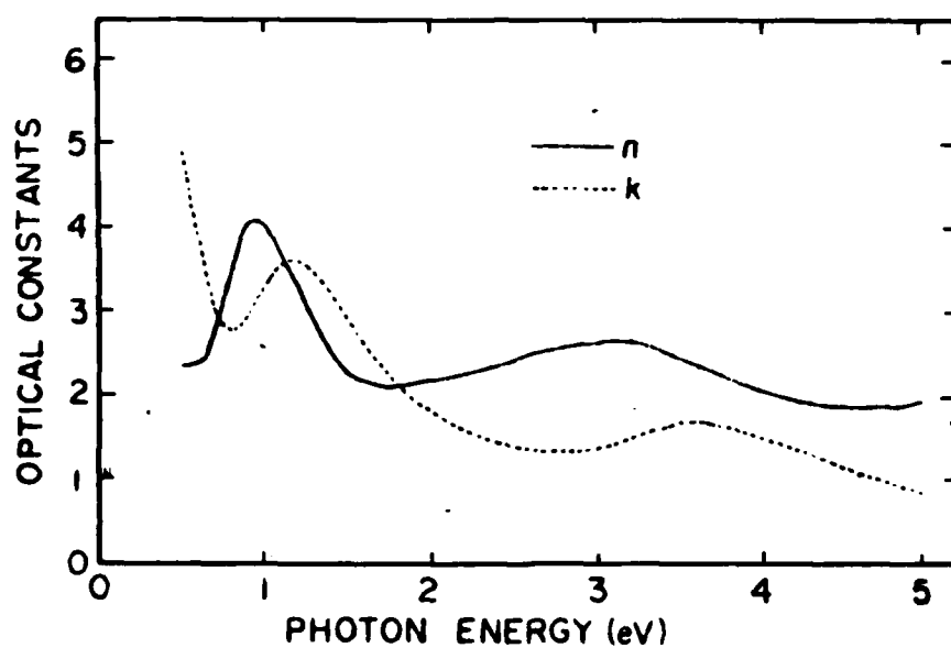
Figure 2. Spectra of optical constants n and k of \text{CoS}_2 deduced from the reflectivity spectrum. Solid curve:— n . Dotted curve: ..... k .
