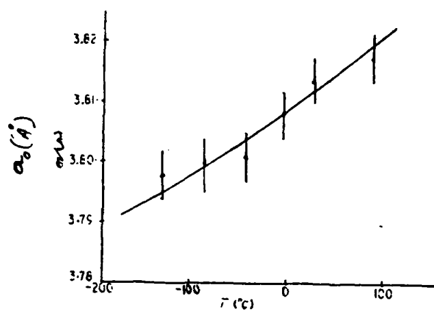
Figure 1. Variation with temperature of lattice parameter a_0 of single \text{SnSe}_2 crystals.
