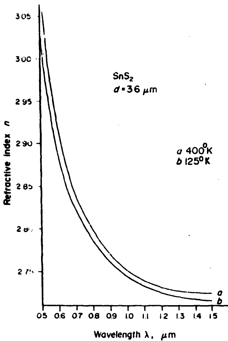
Figure 2(c) - Dispersion Curve for the Compound \text{SnS}_2 .
