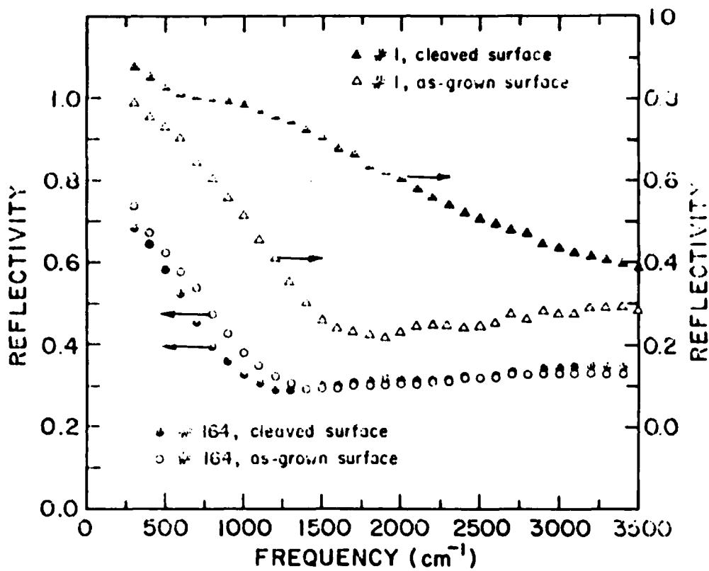
Figure 7. Infrared reflectivity of freshly cleaved and as-grown surfaces of titanium disulfide.
