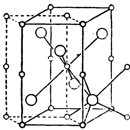
(a) NiAs
