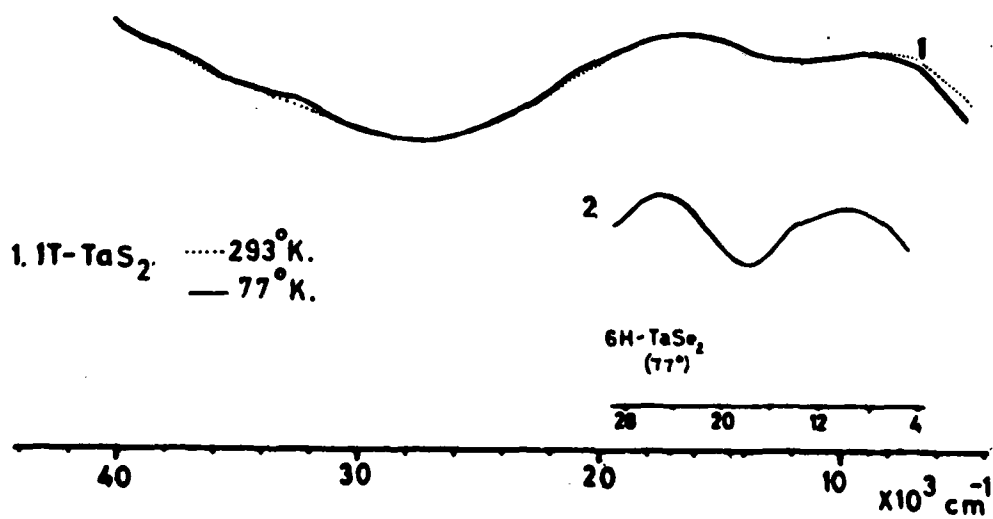
Figure 7. Variation of transmittance of \text{TaS}_2 at two temperatures.
