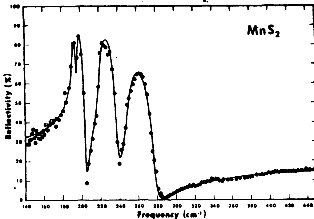
Figure 4. Four oscillator fit to the infrared reflectivity of \text{MnS}_2 . The points are the experimental data and the curve is the theoretical fit.
