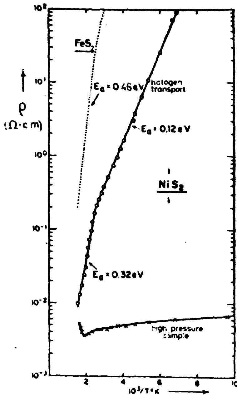
Figure 2. Resistivity vs. Temperature plot for the pyrite semiconductors FeS 2 and NiS 2 .
