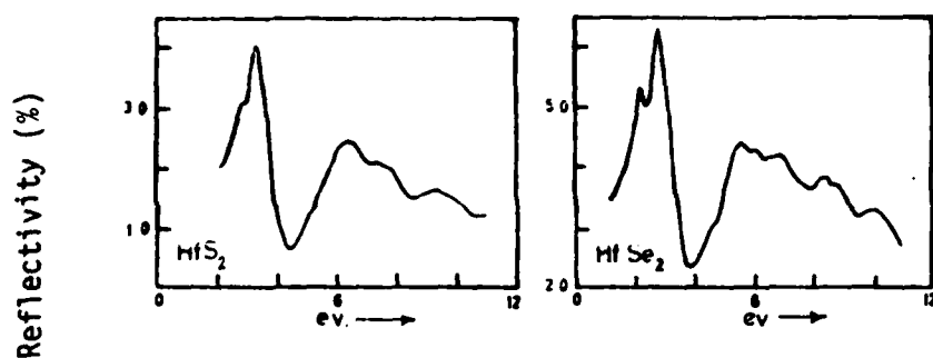
Figure 4. Reflectivity for \text{HfS}_2 and \text{HfSe}_2 .
