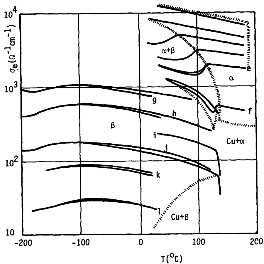
Figure 3. Electronic conductivity \sigma_e vs T for \text{Cu}_{2-\delta}\text{Se} with various \delta -values. The roman letters a,b,...,l correspond to the same ones in Figs. 2 and 4.
