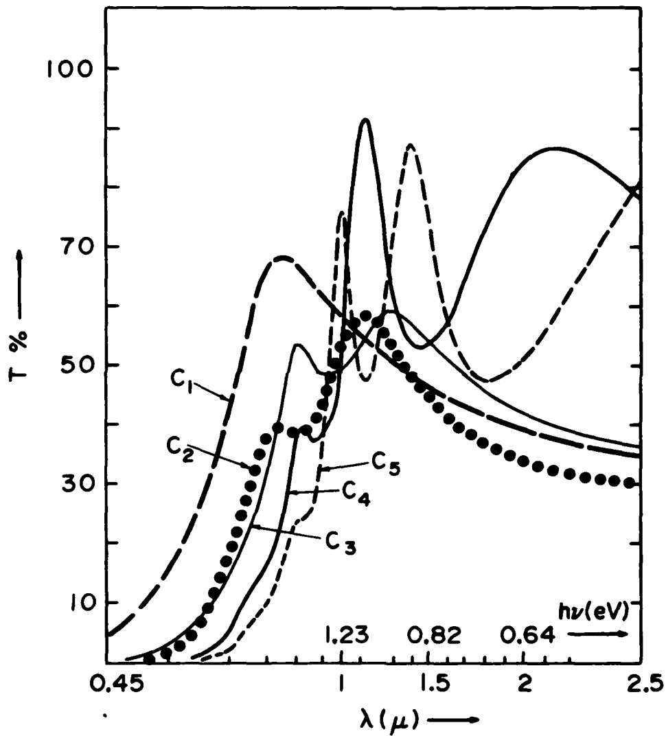
Fig. 2 TRANSMISSION VARIATION VS. WAVELENGTH FOR EVAPORATED \text{Cu}_x\text{S} LAYER OF DIFFERENT THICKNESSES AS TABULATED ABOVE
