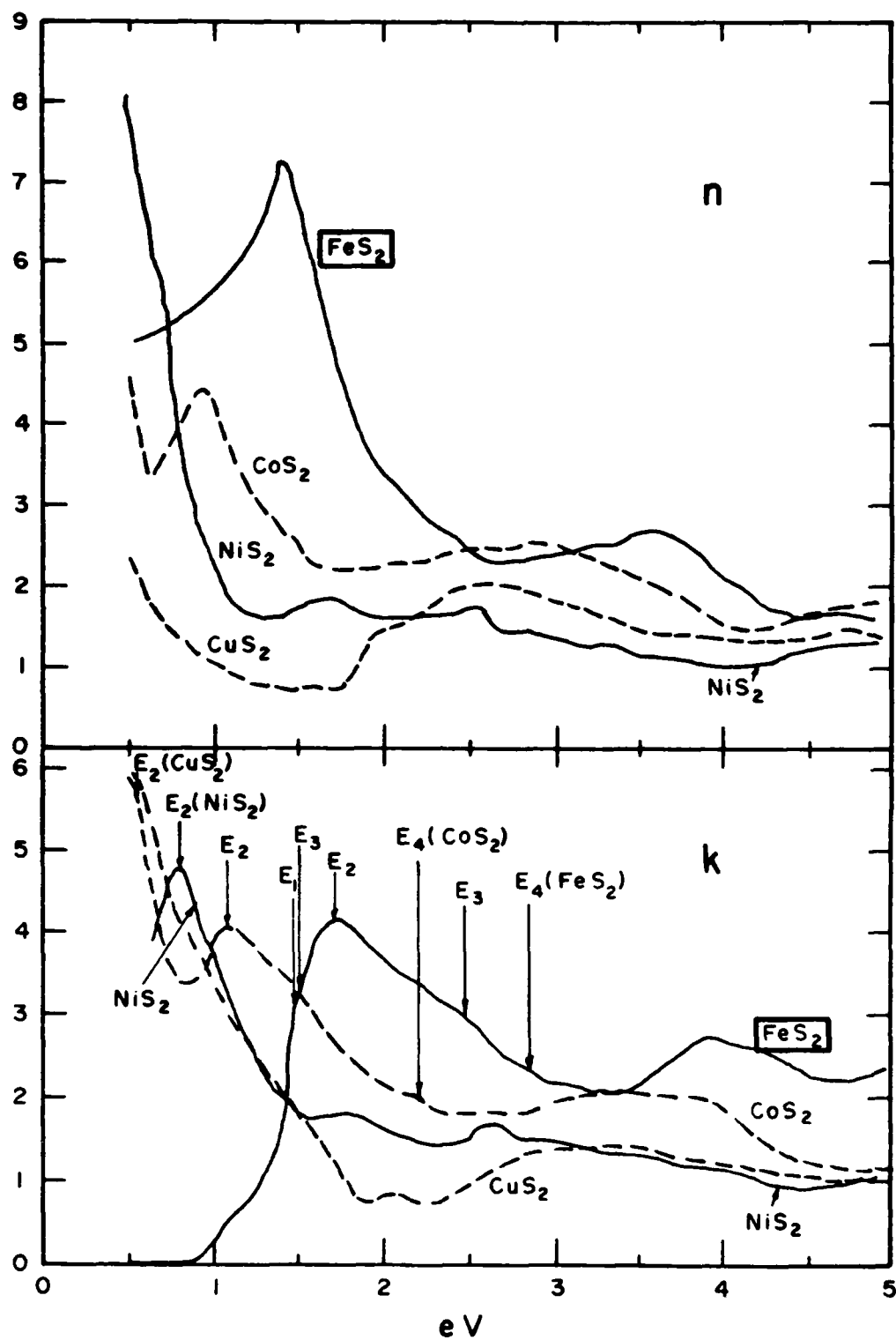
Figure 11. Real and imaginary parts of the complex refractive index for FeS 2 , CoS 2 , NiS 2 and CuS 2 .
