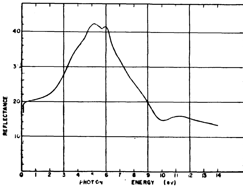
Figure 12. High energy reflectance spectrum of single-crystal MnS.
