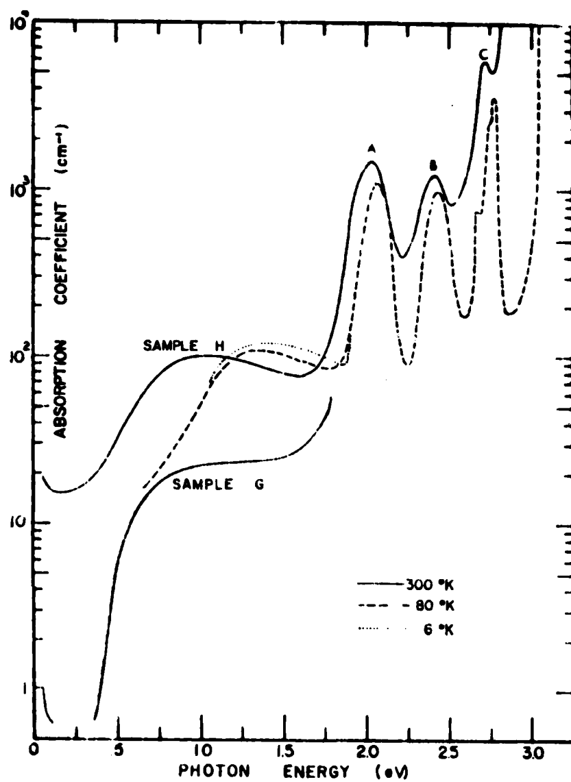
Figure 8. Optical absorption spectra of MnS crystals.
