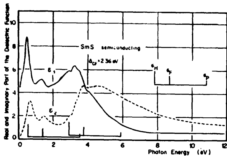
Figure 4. Dielectric function of semiconducting SmS.
