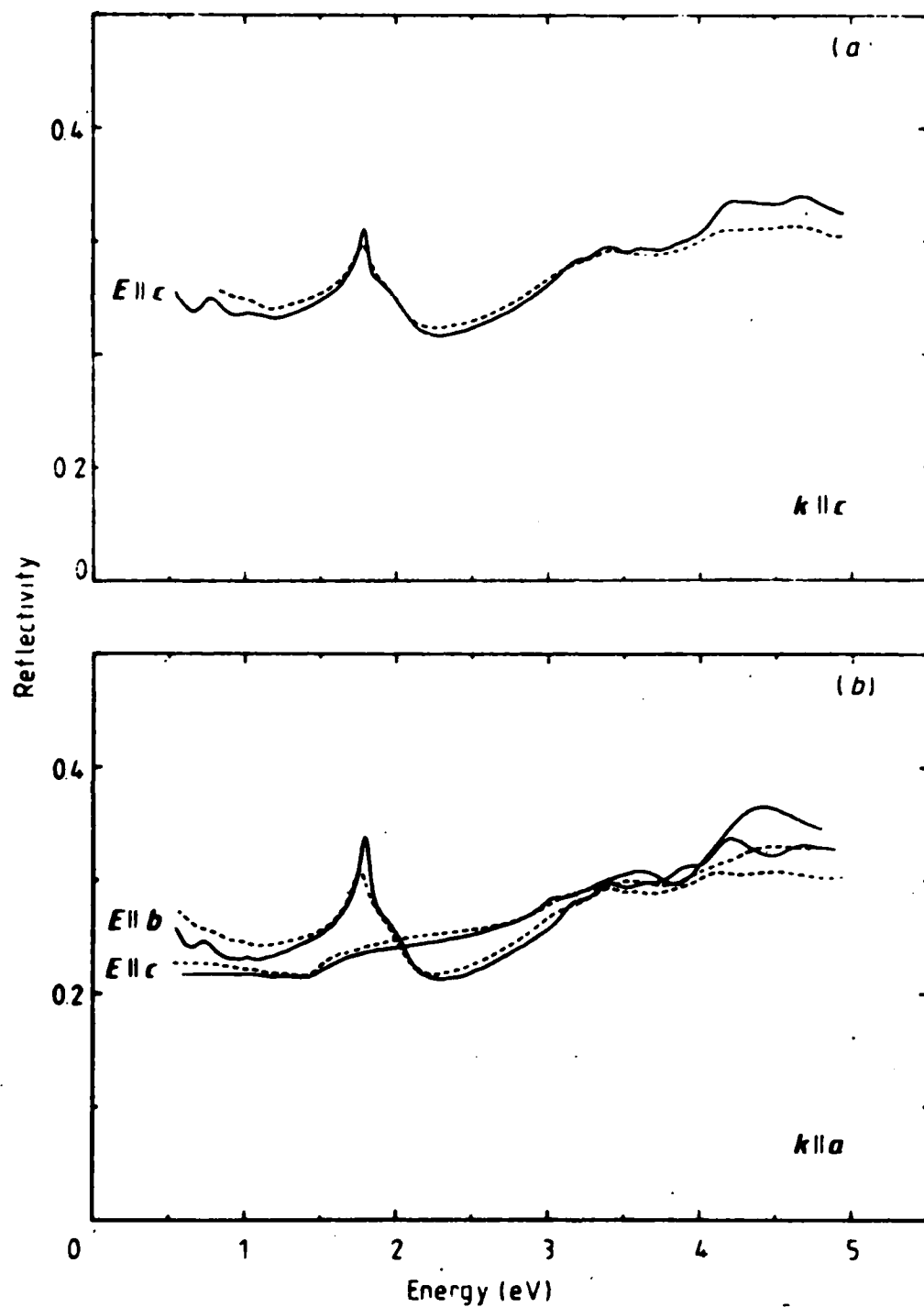
Figure 2 - Reflectivity of \text{ZrSe}_3 . Full curves, 77K; broken curves, room temperature.
