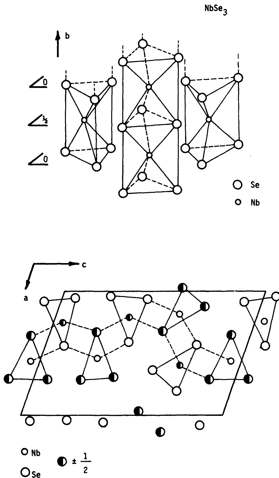
Figure 1. Structure of \text{NbSe}_3 . Upper part: stacking along the b -axis of trigonal prisms \text{NbSe}_6 . Lower part: projection of the structure on the ac plane.
