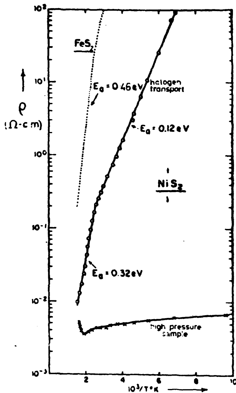
Figure 2. Resistivity vs. Temperature plot for the pyrite semiconductors \text{FeS}_2 and \text{NiS}_2 .
