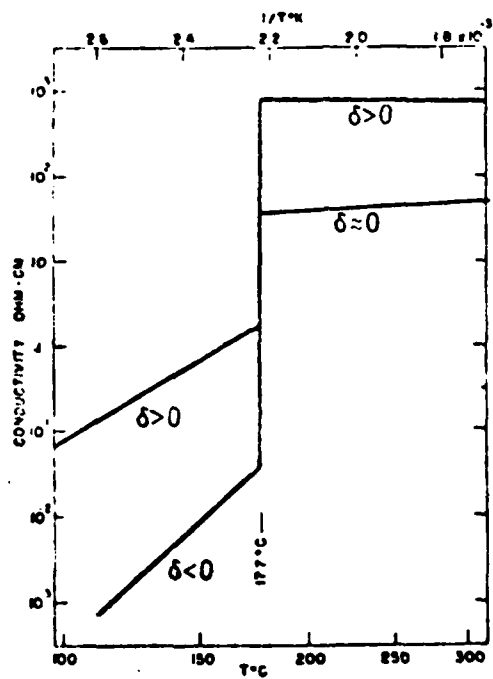
Figure 1. Electrical Conductivity of \text{Ag}_{2+\delta}\text{S} vs. T
