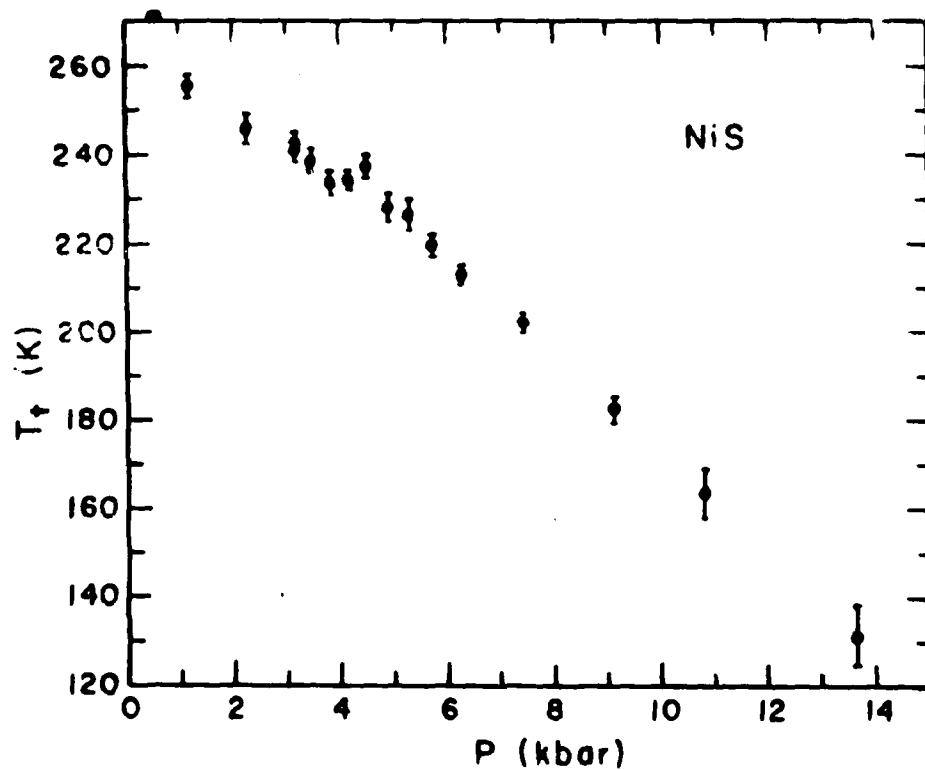
Figure 3. Pressure dependence of the metal - nonmetal transition temperature in hexagonal NiS. There is a local increase in T_t near 4.5 kbar and a 30 percent difference in the magnitude of dT_t/dP measured above and below this region.
