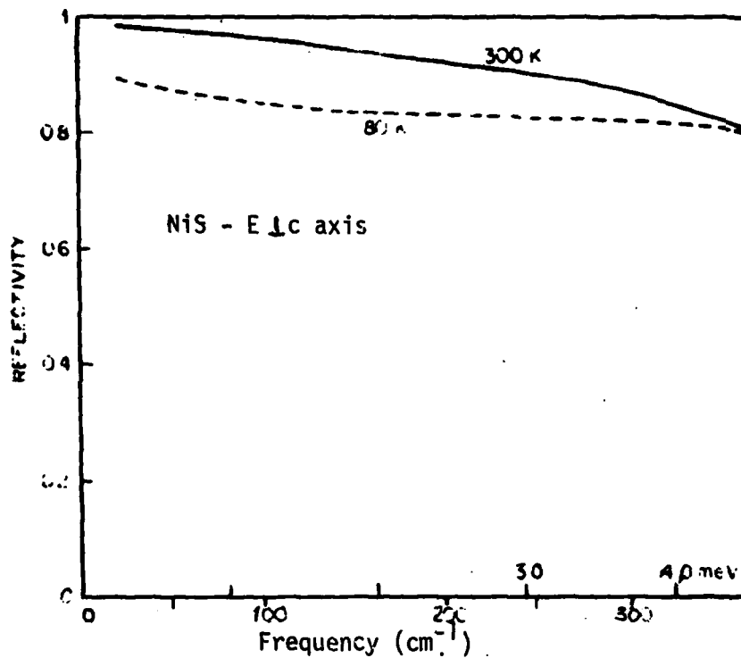
Figure 7. Far-infrared reflectivity of NiS. The 80-K data have a rather large uncertainty in their normalization; they have been chosen to equal the 300-K reflectivity near the 350 cm -1 .
