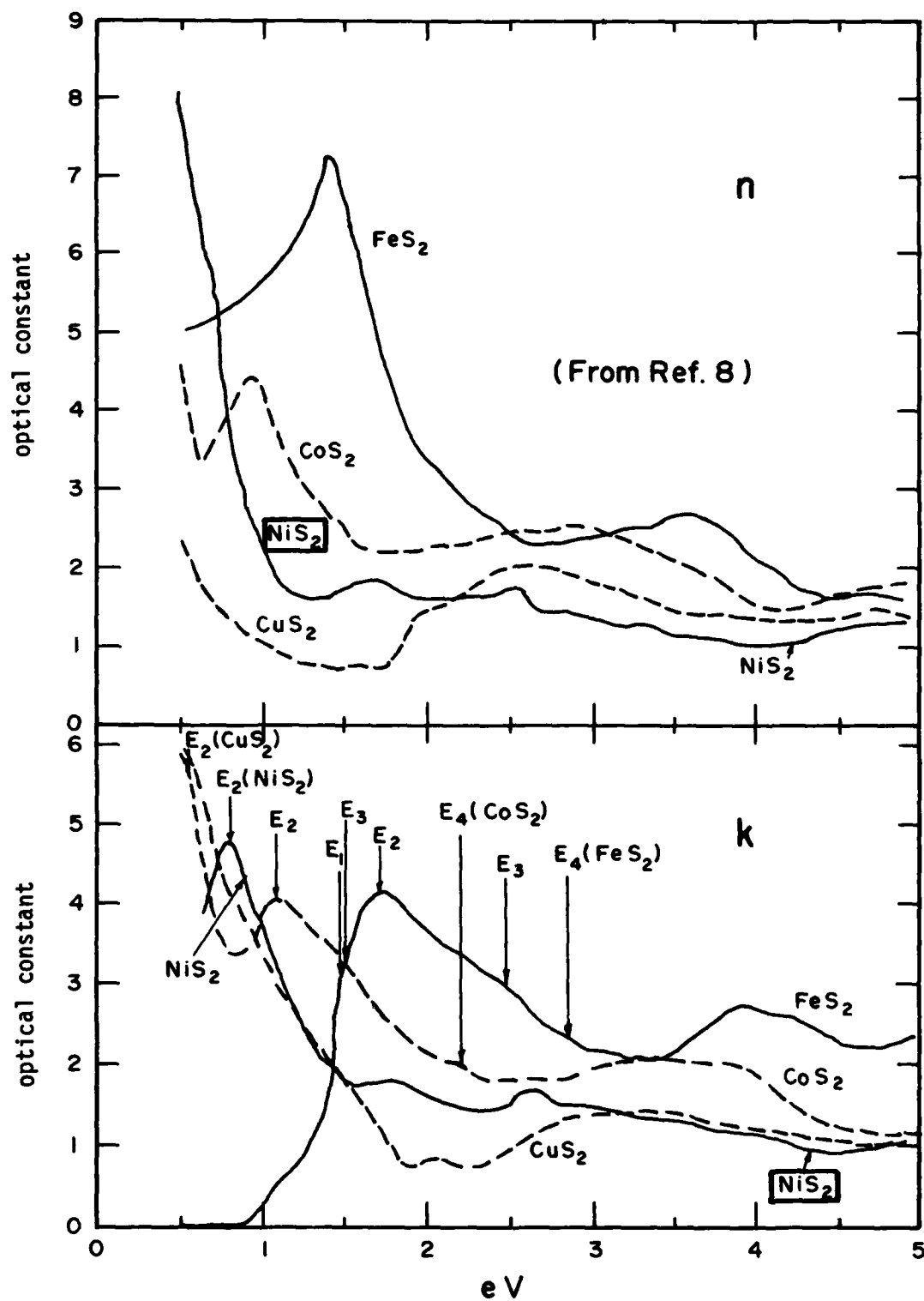
Figure 3. Real and imaginary parts of the complex refractive index for FeS 2 , CoS, NiS and CuS 2 .
