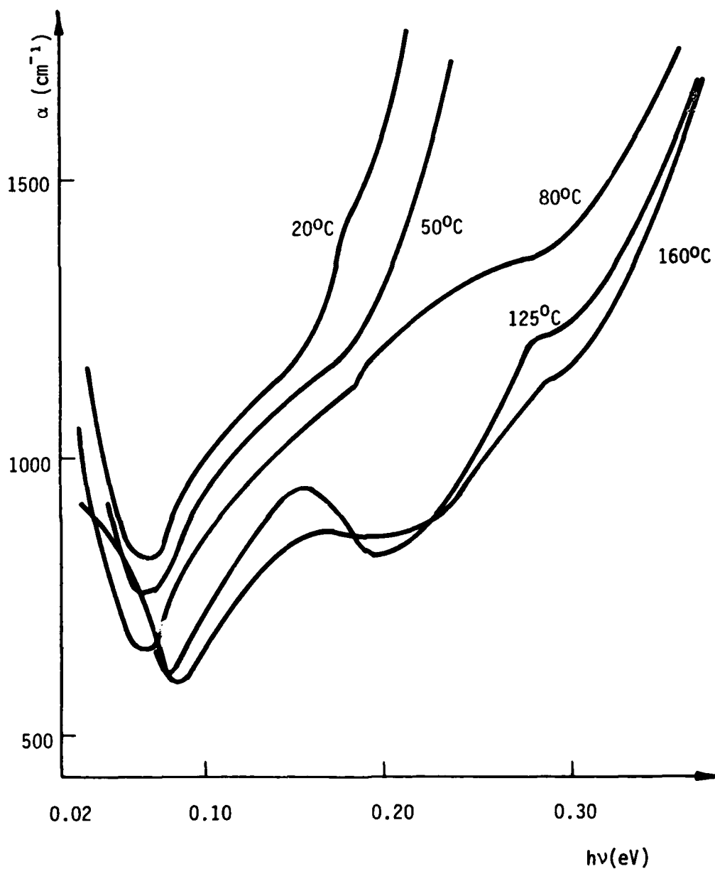
Figure 2. Optical absorption of \text{Ag}_2\text{Se} at various temperatures. This figure demonstrates the presence of two different absorption mechanisms: (a) For photon energies lower than about 0.05 eV, free-carrier absorption is predominant; (b) for photon energies larger than about 0.1 eV, absorption is due to interband transitions.
