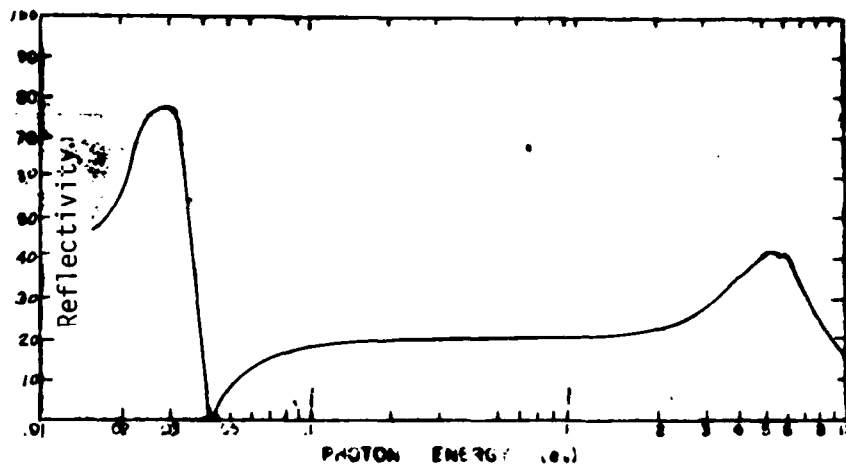
Figure 11. Reflectance spectrum of MnS
