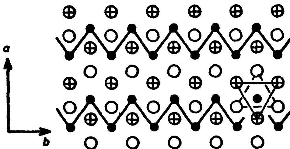
Figure 1. Plan of the structure of a single layer of \beta -MoTe 2 , illustrating the formation of zig-zag chains of Mo atoms (after Brown 1966). \oplus represents the top sheet of Te atoms and \bigcirc the lower sheet, while \bullet represents the middle sheet of Mo atoms.
