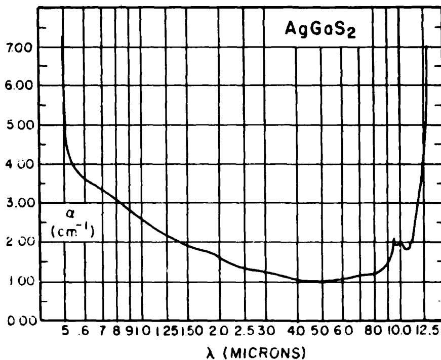
Figure 2. Room temperature absorption coefficient \alpha (cm -1 ) versus wavelength ( \lambda ) for AgGaS 2
