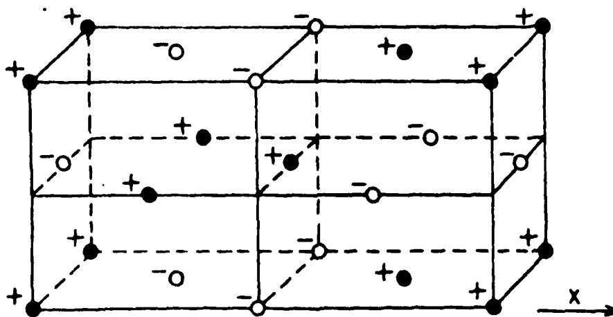
Figure 5. Magnetic ordering scheme deduced from diffraction studies. Spins lie in the yz plane but the direction within this plane is not completely determined.
