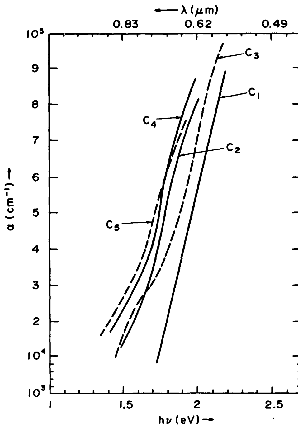
Fig. 3 ABSORPTION COEFFICIENT VS. PHOTON ENERGY
