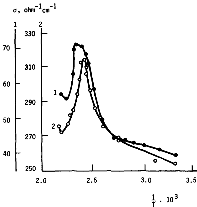
Figure 1. Effect of temperature on the electrical conductivity of Ag 2 Te (1), and Ag 2 Se (2).
