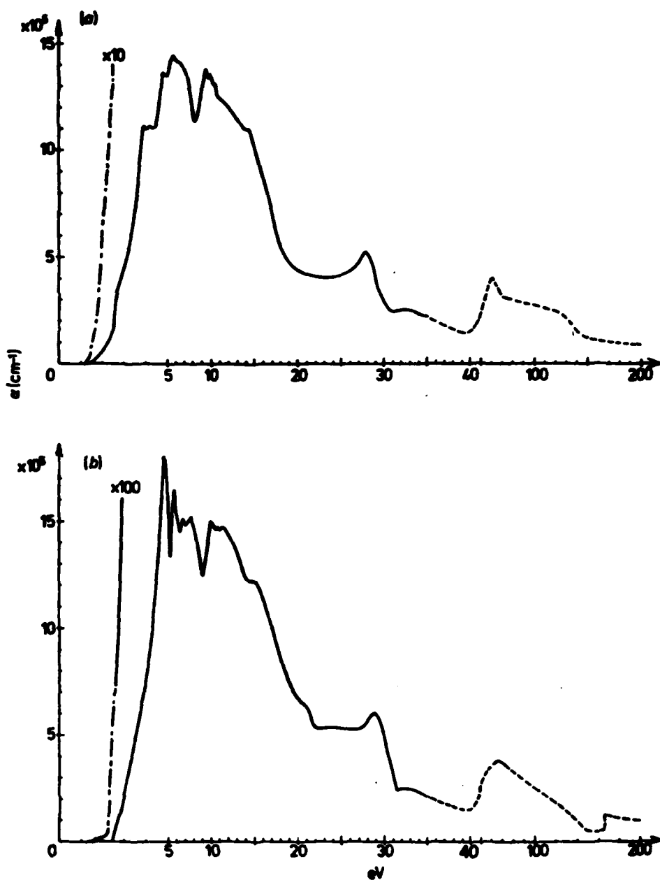
Figure 10. Absorption coefficient of (a) \text{SnSe}_2 and (b) \text{SnS}_2 .
