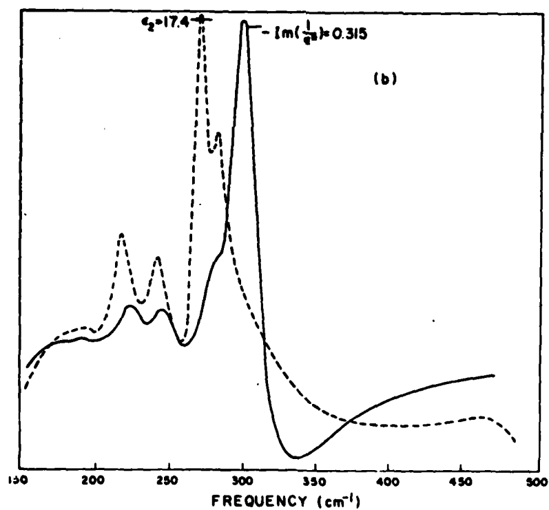
Figure 3. Calculated frequency dependence of \epsilon_2 (dashed lines) and -\text{Im}(1/\epsilon^*) (solid lines) of \text{HfS}_3 from the reflectivity spectra. (a) parallel, (b) perpendicular to the chains.
