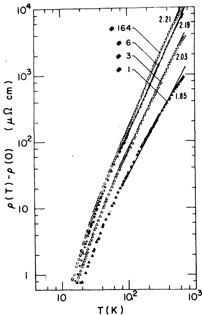
Figure 2. Log-log plot of the temperature-dependent electrical resistivity of four samples of titanium disulfide \text{Ti}_{1+x}\text{S}_2 for varying degrees of nonstoichiometry.
