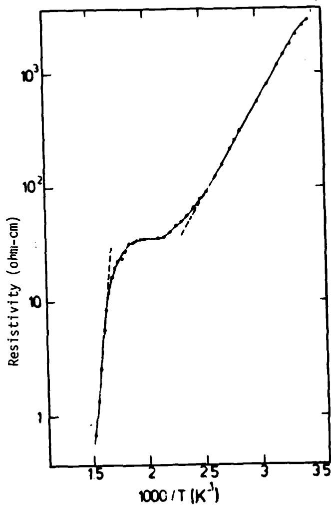
Figure 7. Temperature dependence of the resistivity of the same crystal as used in Figure 6 after two heating-cooling cycles.
