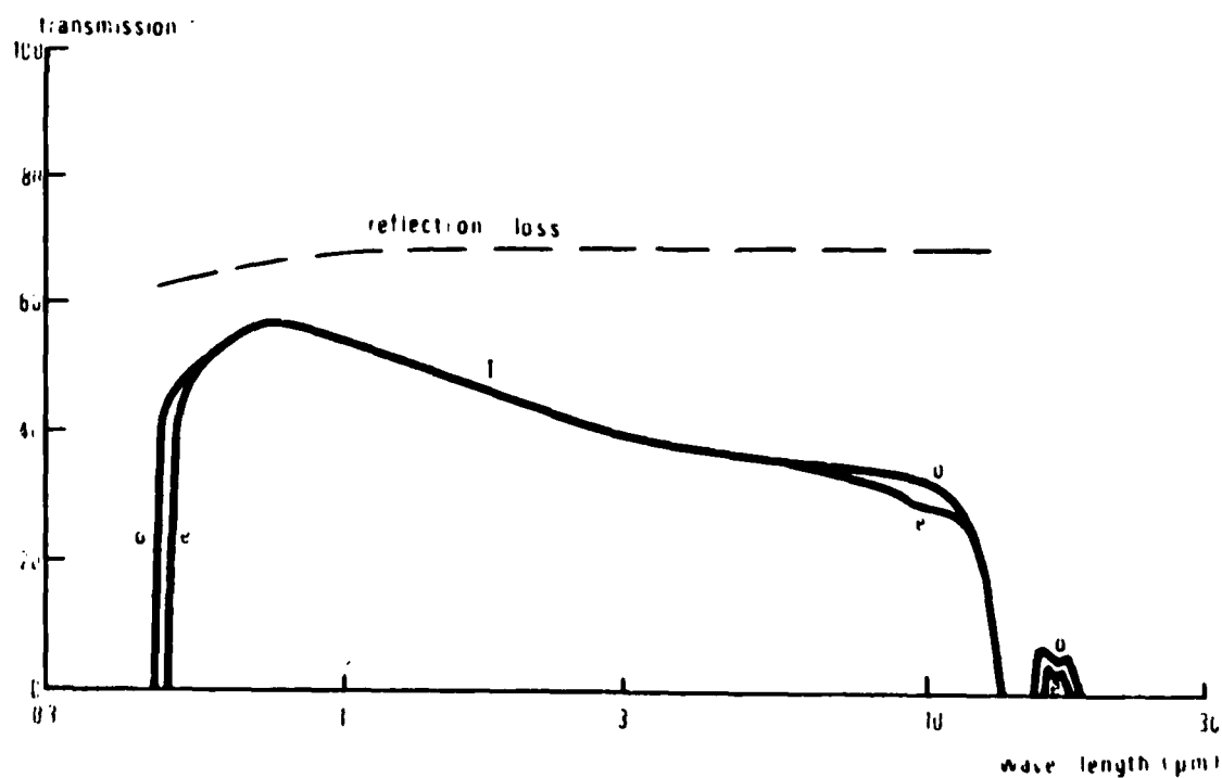
Figure 3. Transmission of a 1.2mm plate of AgGaS 2 . The optic axis was at 40° to the plate.
