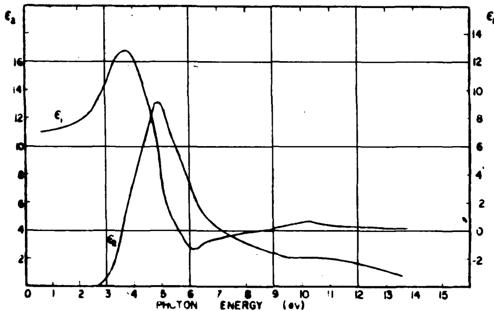
Figure 13. Spectral dependence of the real and imaginary parts of the dielectric constant calculated from reflectance data.
