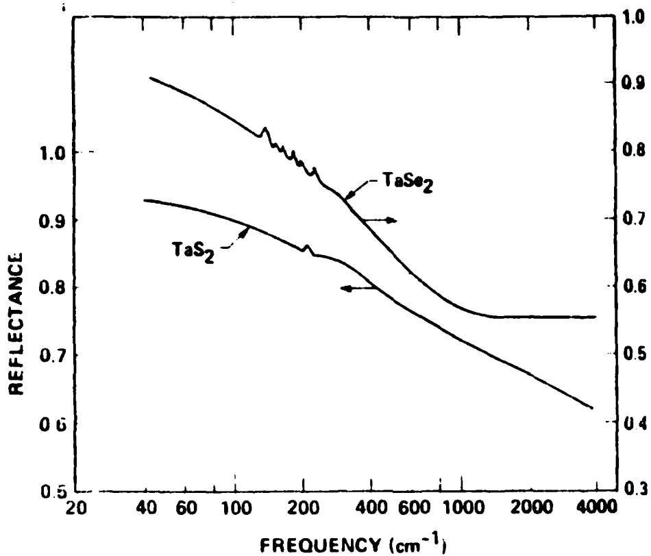
Figure 6. Room-temperature reflectance spectra for \text{TaS}_2 and \text{TaSe}_2 .
