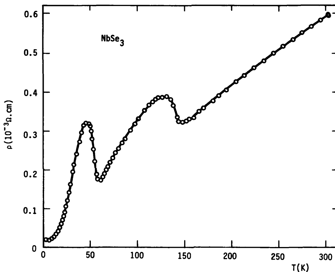
Figure 2. Electrical resistivity as a function of temperature along the b-axis of NbSe 3 showing the two phase transition at T_{e1} = 145\text{K} and T_{e2} = 59\text{K} . The resistivity maxima are for 125 and 49K.
