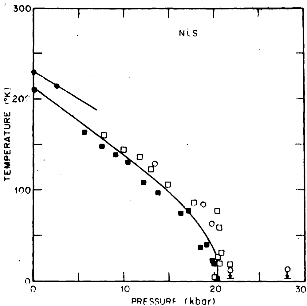
Figure 2. Pressure-temperature phase diagram for NiS. Open and closed symbols are for increasing and decreasing temperature of pressure. Circles are sample with T_N = 230^\circ\text{K} at 1 atm and squares for sample with T_N = 210^\circ\text{K} .
