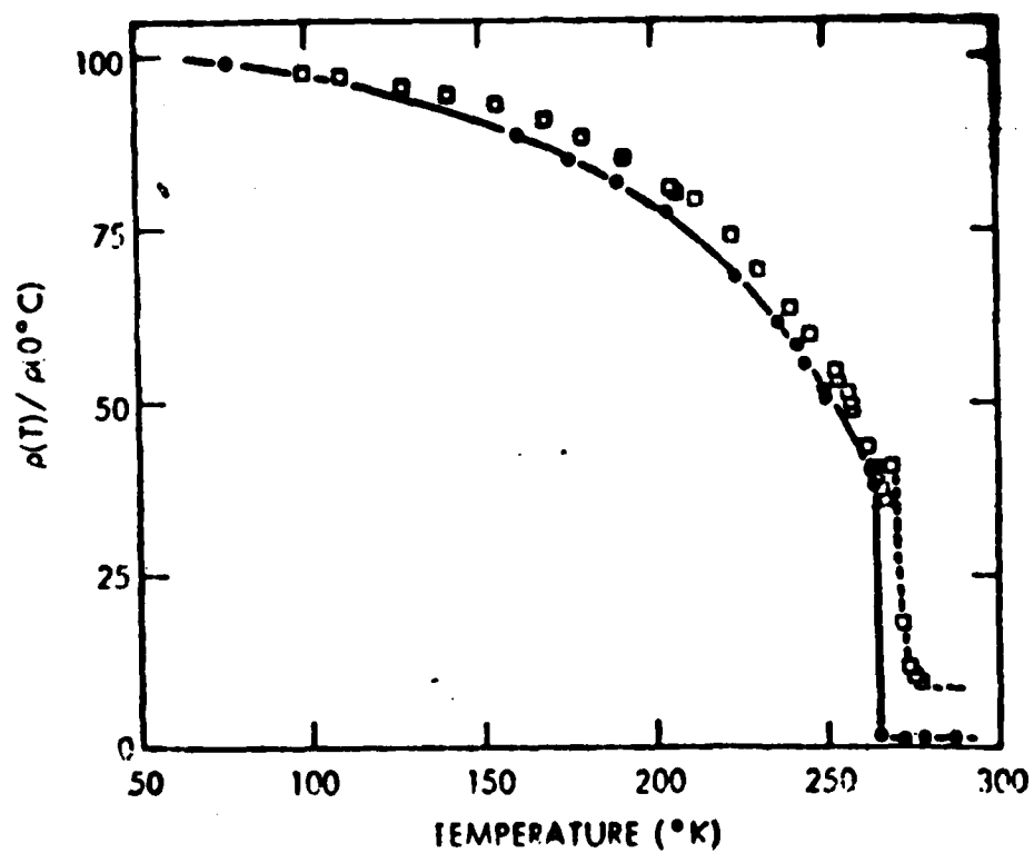
Figure 4. Relative resistivity versus temperature for a single crystal of NiS.
