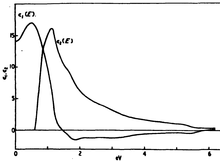
Figure 6. Real and imaginary parts of the dielectric constant \epsilon_1 and \epsilon_2 of \text{MoTe}_2 from Kramers-Kronig analysis.
