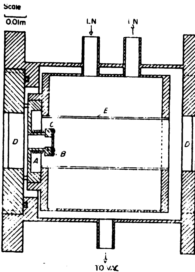
Figure 1 - Cross-section diagram of the optical cryostat.
