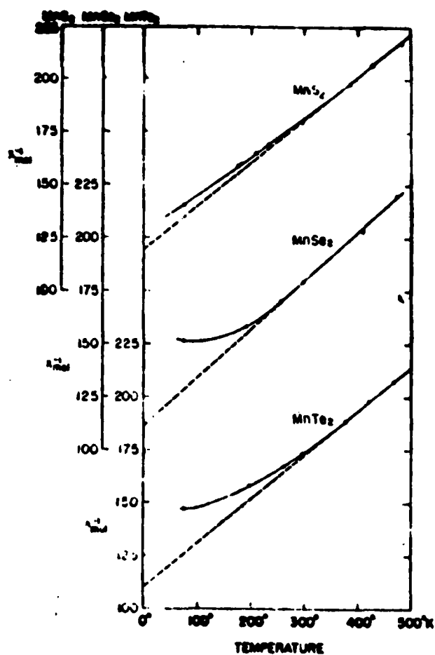
Figure 2. Inverse susceptibilities of \text{MnS}_2 , \text{MnSe}_2 , and \text{MnTe}_2 as a function of temperature.
