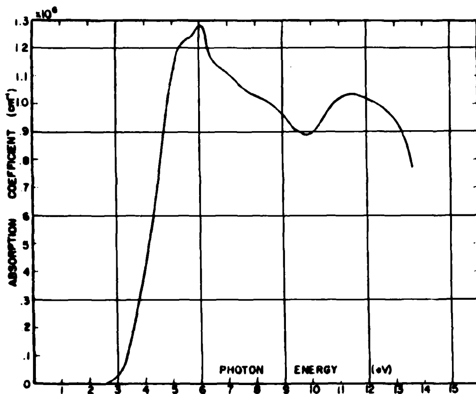
Figure 9. Spectral dependence of the absorption coefficient calculated from reflectance data.
