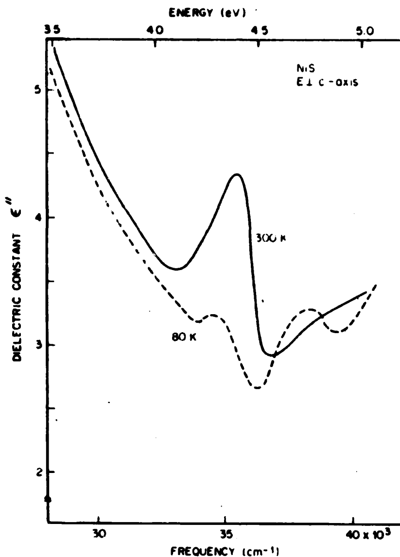
Figure 6 - Imaginary part of the dielectric constant \epsilon'' obtained by Kramers-Kronig analysis of the reflectivity data in the visible and ultraviolet regions.
