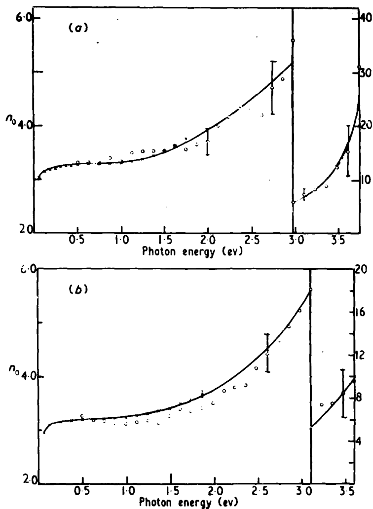
Figure 11. Spectral variation of the ordinary refractive index n_0 of \text{SnSe}_2 at (a) 290^\circ\text{K} , (b) 77^\circ\text{K} . (x) determined from interference spectra and (o) thick crystal reflectivity R_0 .
