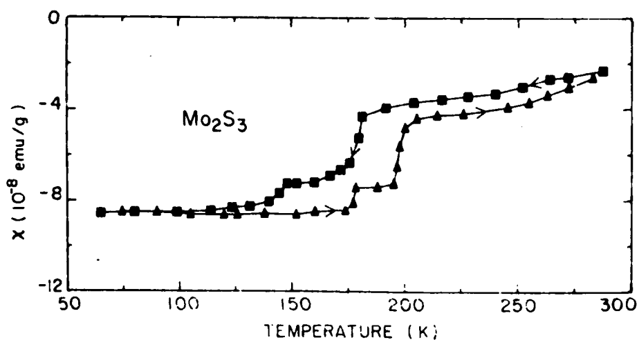
Figure 3. Magnetic susceptibility of \text{Mo}_2\text{S}_3 as a function of temperature. The solid lines are guides to the eye.
