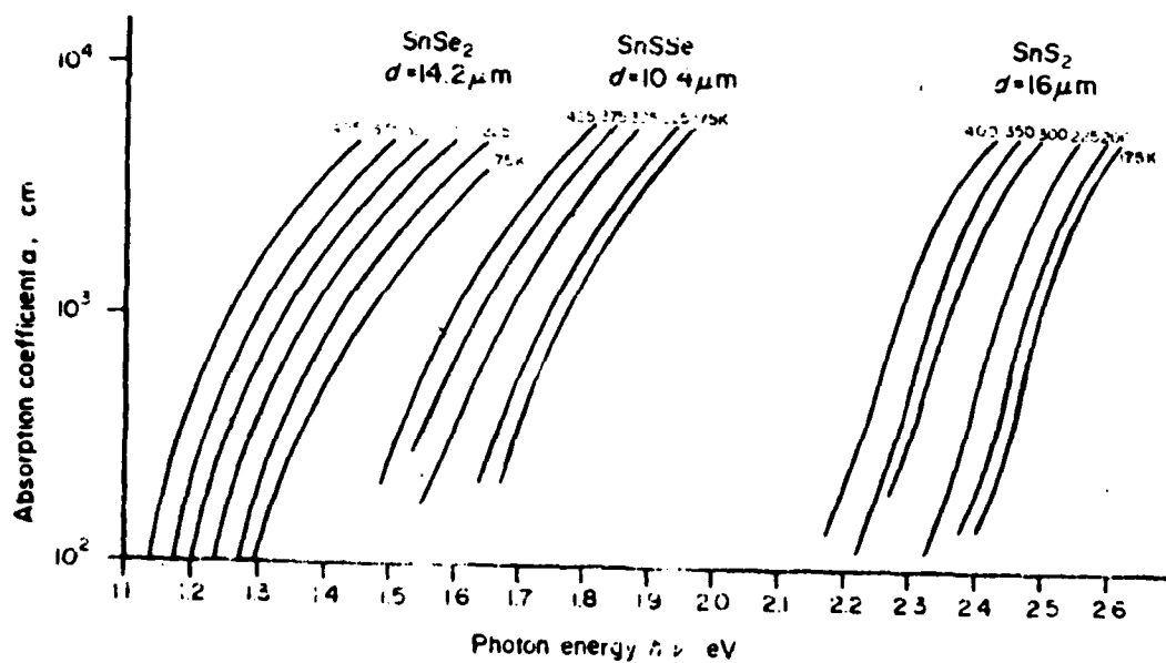
Figure 4 - The absorption coefficient for SnS_xS_{2-x} ( x = 0, 1, 2 ) as a function of photon energy and temperature.
