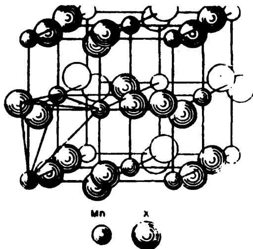
Figure 1. The pyrite structure.
