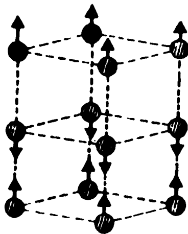
Figure 1. Spin structure in hexagonal NiS. The sulfur atoms are not shown.
