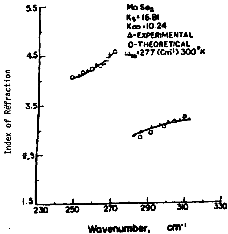
Figure 2 - Index of refraction vs. frequency near the fundamental infrared lattice vibration region.
