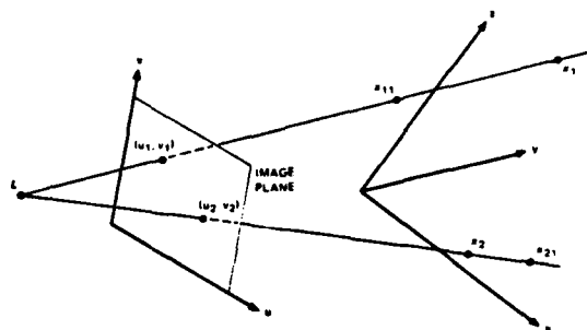
FIGURE 3 DETERMINING THE LOCATION OF THE CAMERA
