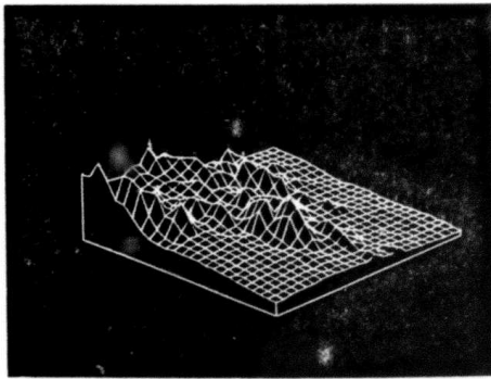
Figure 2. Data Sampled at Grid Intersections
