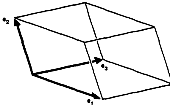
Figure 9: Parallelepiped Associated with Basis Vectors
