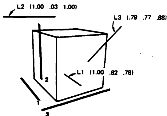
Figure 13: Consistencies of Three Lines
