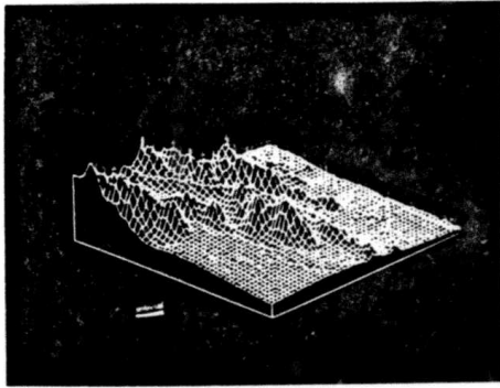
Figure 1. Real Surface Used as Ground Truth
