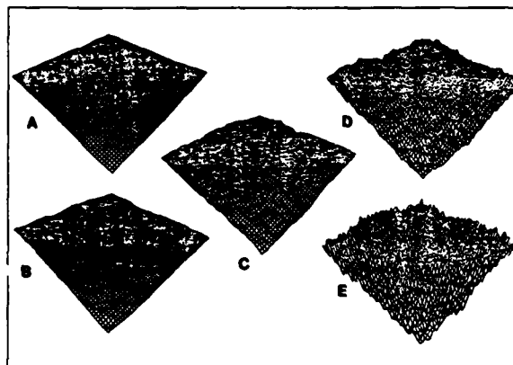
Figure 1. Surfaces of Increasing Fractal Dimension.
