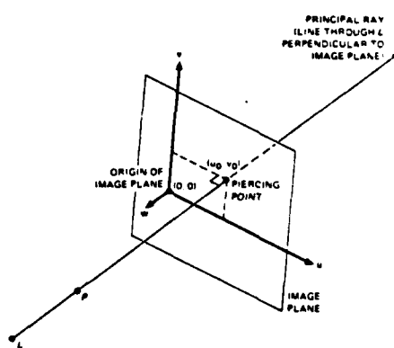
FIGURE 5 DETERMINING THE PIERCING POINT
