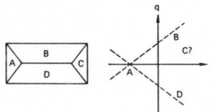
Figure 10: Another ambiguous drawing.
