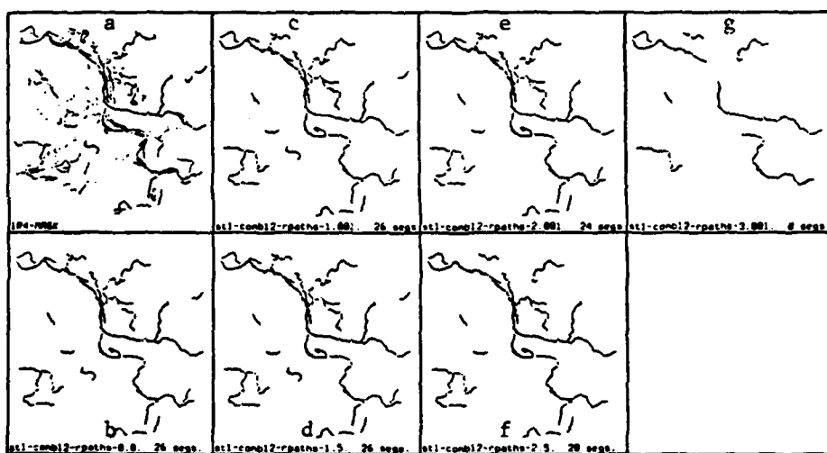
Figure 6. Linear Structure in the Composite Vertical Image
