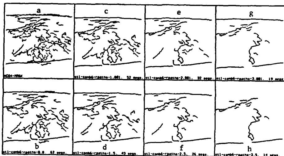
Figure 5. Linear Structure in the Composite Oblique Image
