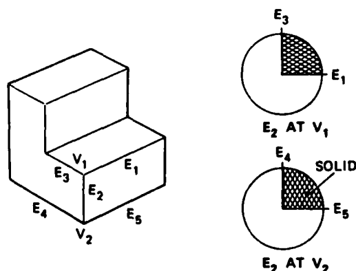
Figure 6: Propagation of Intervortex Constraints.
