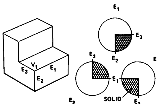
Figure 5: Propagation of Intravertex Constraints.
