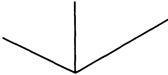
Figure 1: A Right-Angle Illusion
