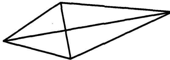
Figure 3: A Tetrahedron
