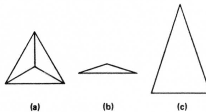
Figure 9: An ambiguous drawing.
