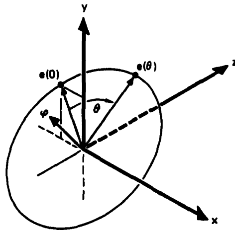
Figure 8: Basis Vector in an Interpretation Plane
