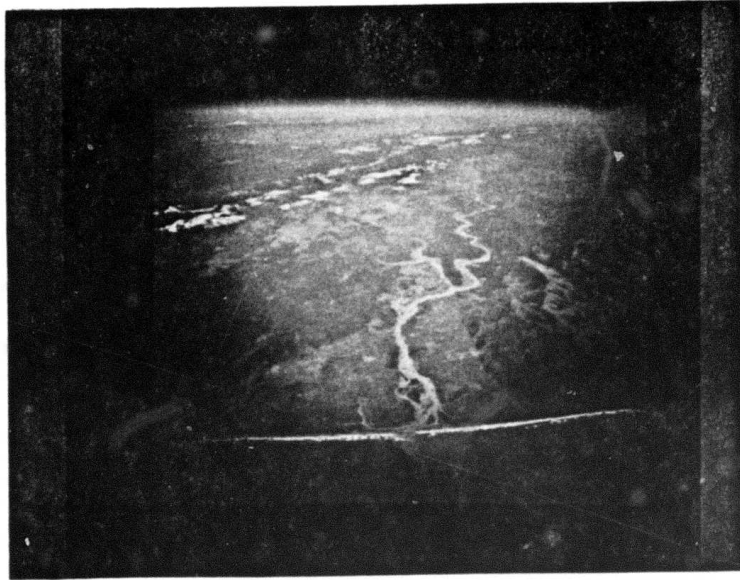
Figure 1. Oblique Natural-Color Image of the Eel River
