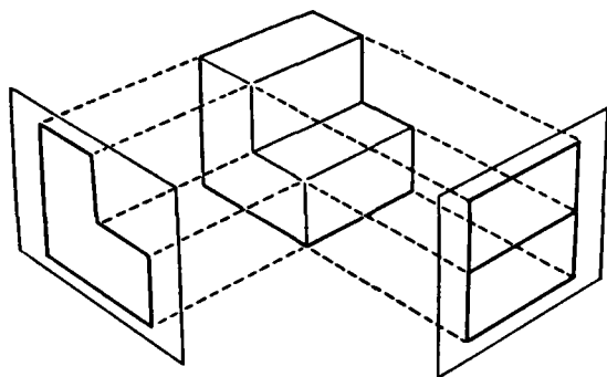
Figure 3: The geometry of backward projection.
