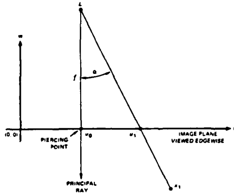
FIGURE 6 DETERMINING THE SCALE FACTOR
