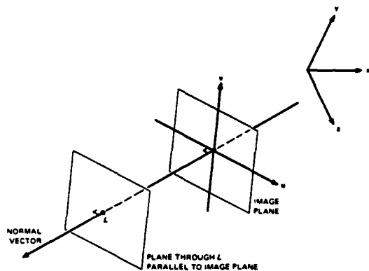
FIGURE 4 DETERMINING THE ORIENTATION OF THE CAMERA
