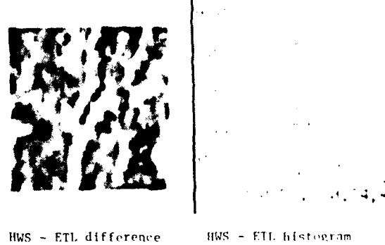
FIGURE 5 HWS vs. ETL results for area B
