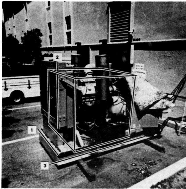
Figure 11: The Interpretation of Figure 10d in Context
