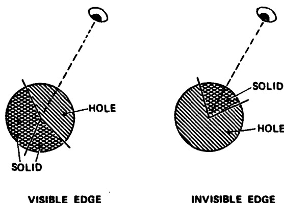
Figure 7: Hidden-line removal.
