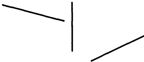
Figure 2: A Common Vertex is not Required
