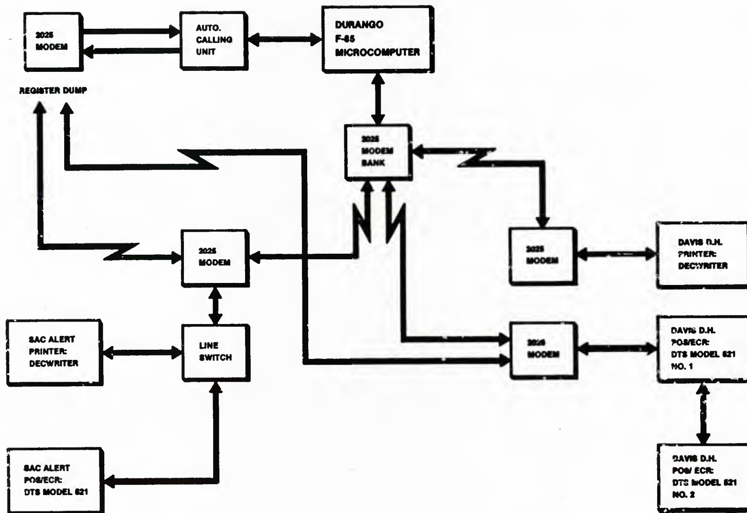
Figure 2. AFSOS Hardware and Telecommunications Network
