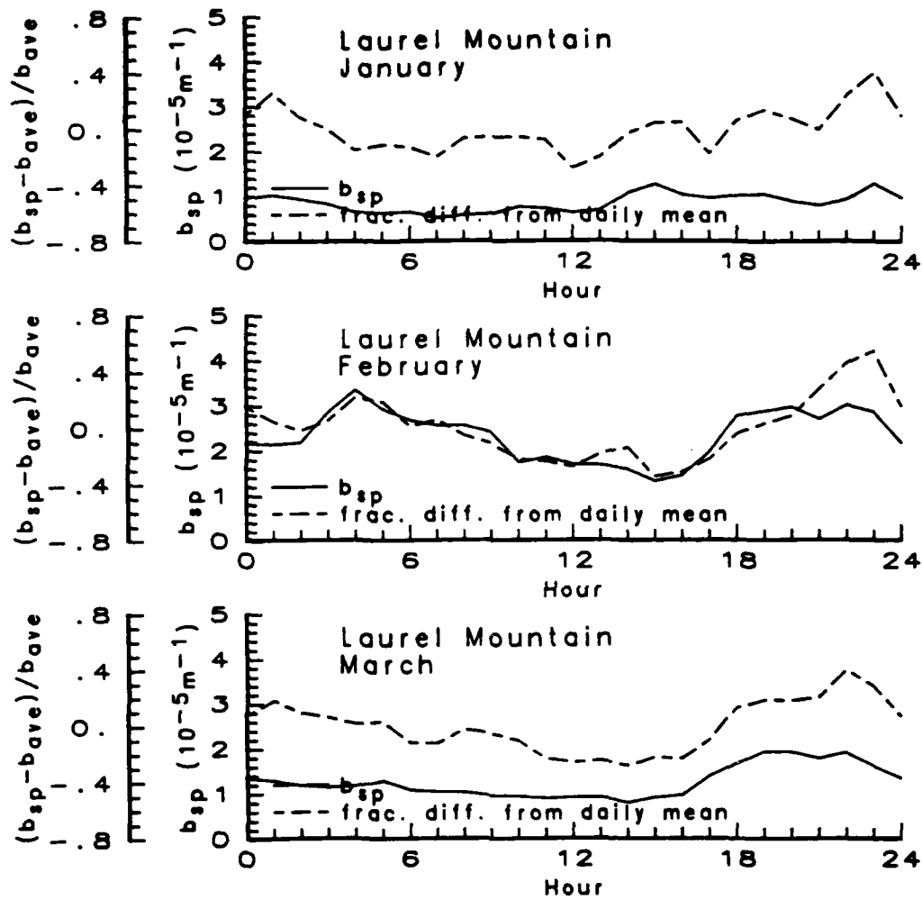
FIGURE A-3. Monthly Diurnal Patterns of Particle Scattering at Laurel Mountain.
