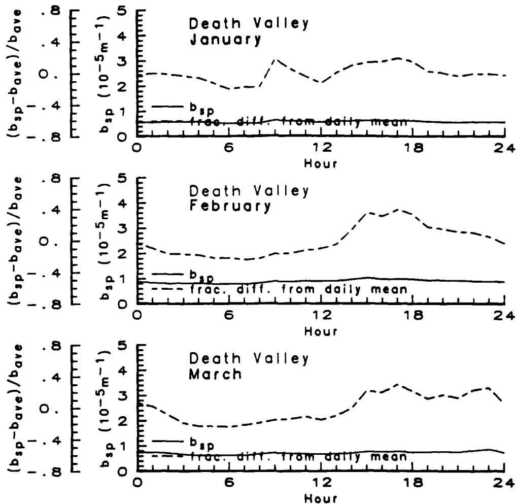
FIGURE A-5. Monthly Diurnal Patterns of Particle Scattering at Death Valley.
