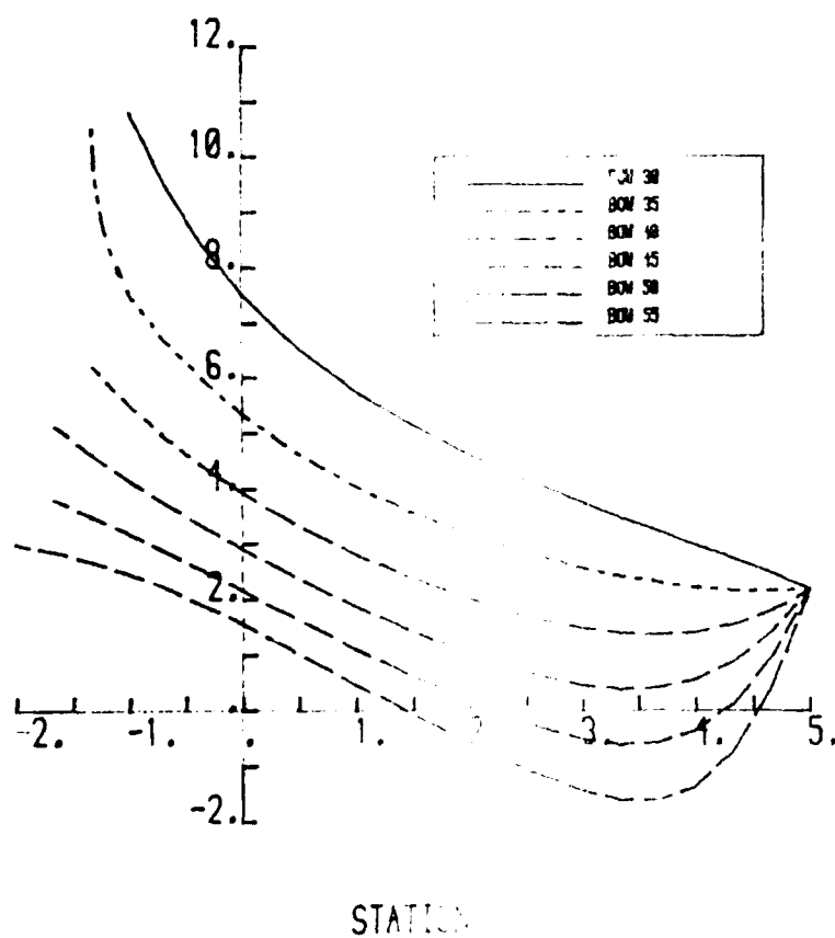
FIG. 37 CRITICAL AREA OF VERTICAL WATER VELOCITY
