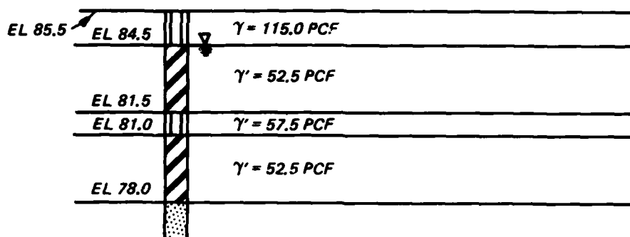
Figure A17. Soil stratification for Example Problem A5
