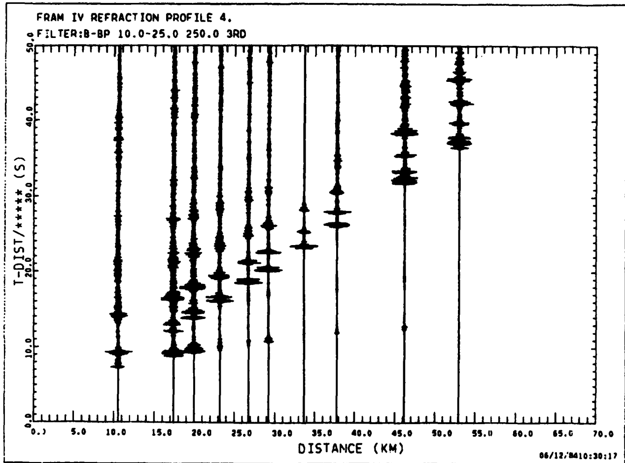
Fig. VII.7.2 Record section of filtered hydrophone playout for Line 4. Ten shots were recorded on 19th and 20th April 1982. Sampling rate in 4 ms. The dominant arrivals are the water-wave and multiple reflections.
