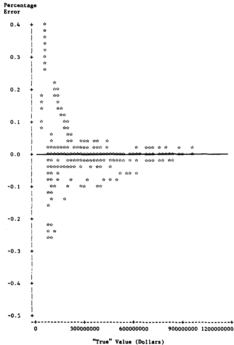
Fig. 10—Percentage error vs "true" actual depot repairs (valued at repair cost) for the F-4 aircraft alternative peacetime programs
