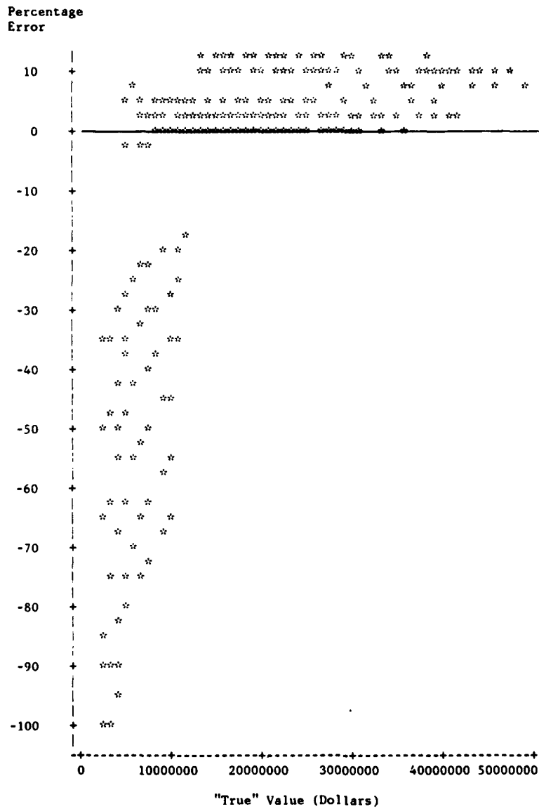
Fig. 8—Percentage error vs "true" required buy of 1-2 year lead time items for the F100 engine alternative wartime programs
