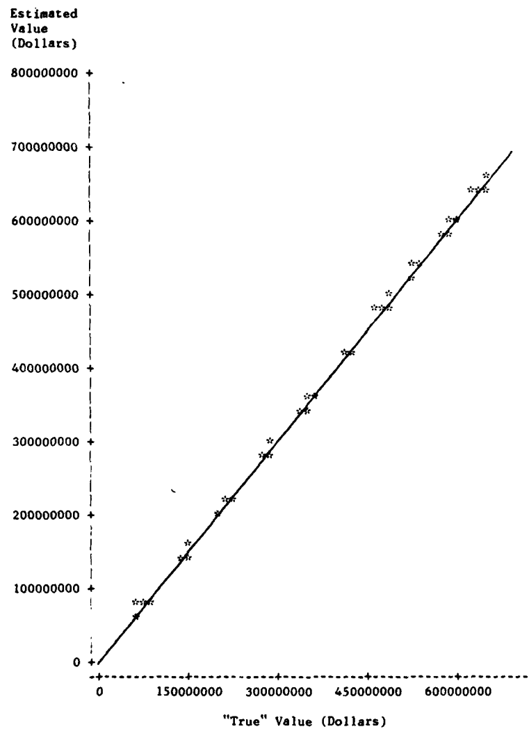
Fig. 11—Estimated vs "true" actual depot repairs (valued at repair cost) for the F-4 aircraft alternative wartime programs
