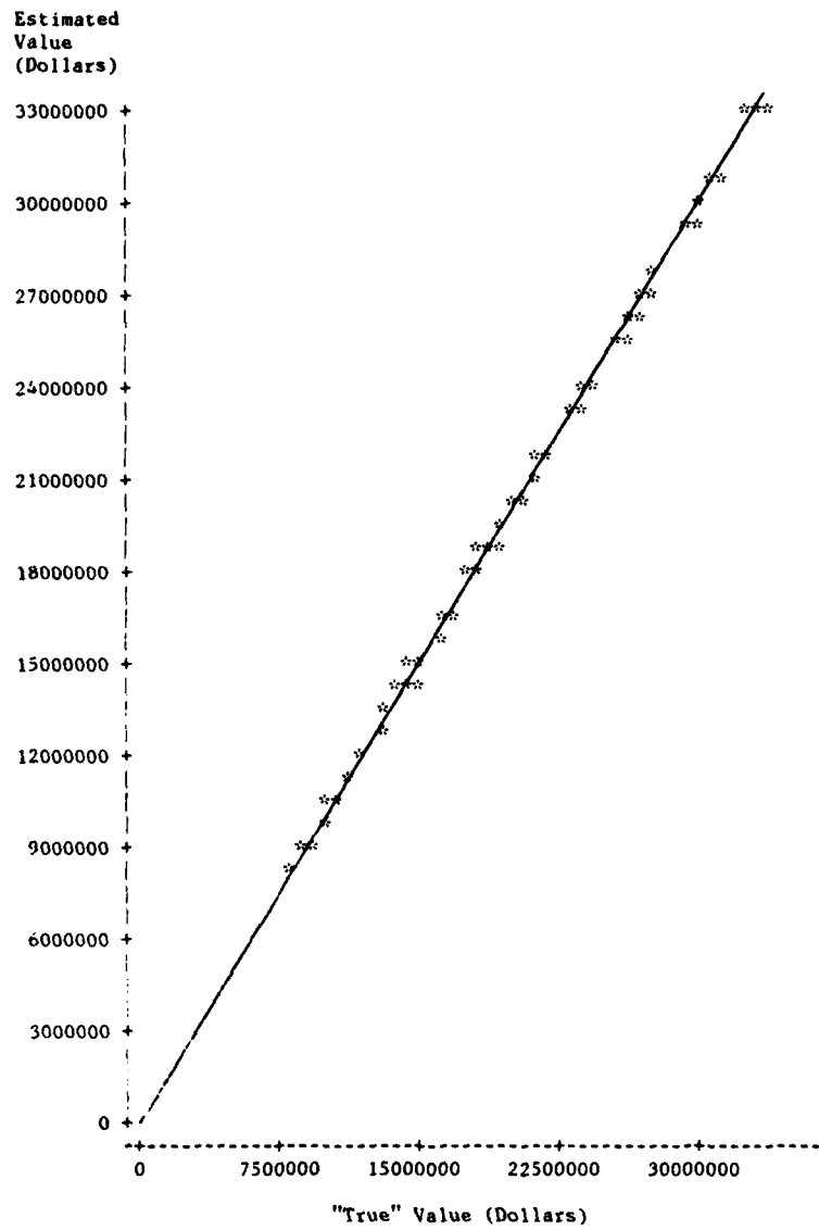
Fig. 5—Estimated vs "true" required buy of 1-2 year lead time items for the F100 engine alternative peacetime programs
