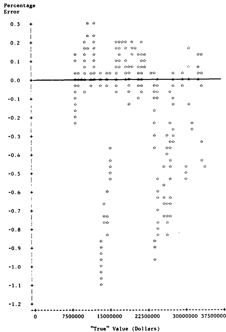
Fig. 6—Percentage error vs "true" required buy of 1-2 year lead time items for the F100 engine alternative peacetime programs
