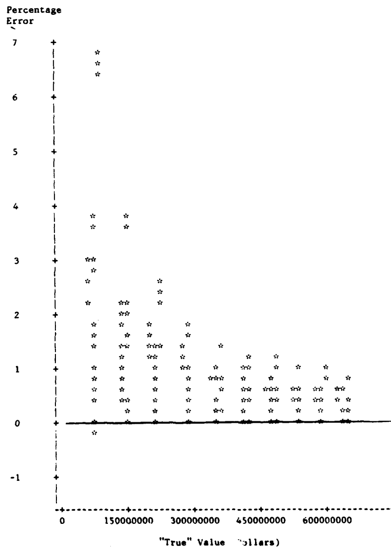
Fig. 12—Percentage error vs "true" actual depot repairs (valued at repair cost) for the F-4 aircraft alternative wartime programs
