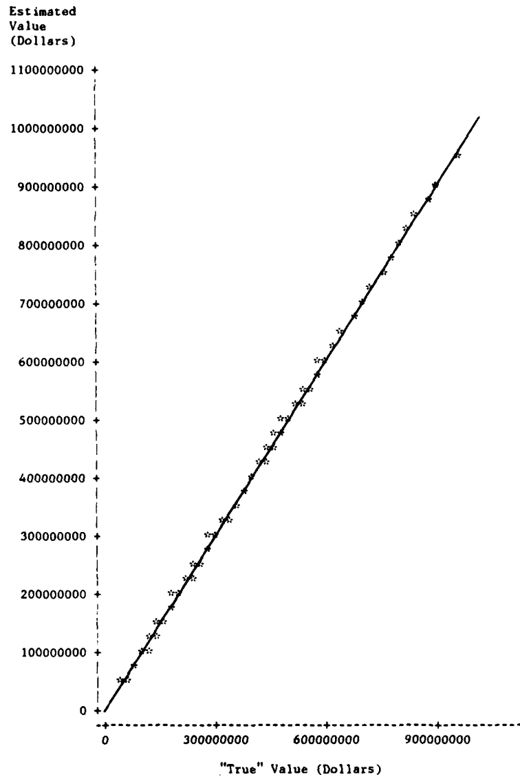
Fig. 9—Estimated vs "true" actual depot repairs (valued at repair cost) for the F-4 aircraft alternative peacetime programs
