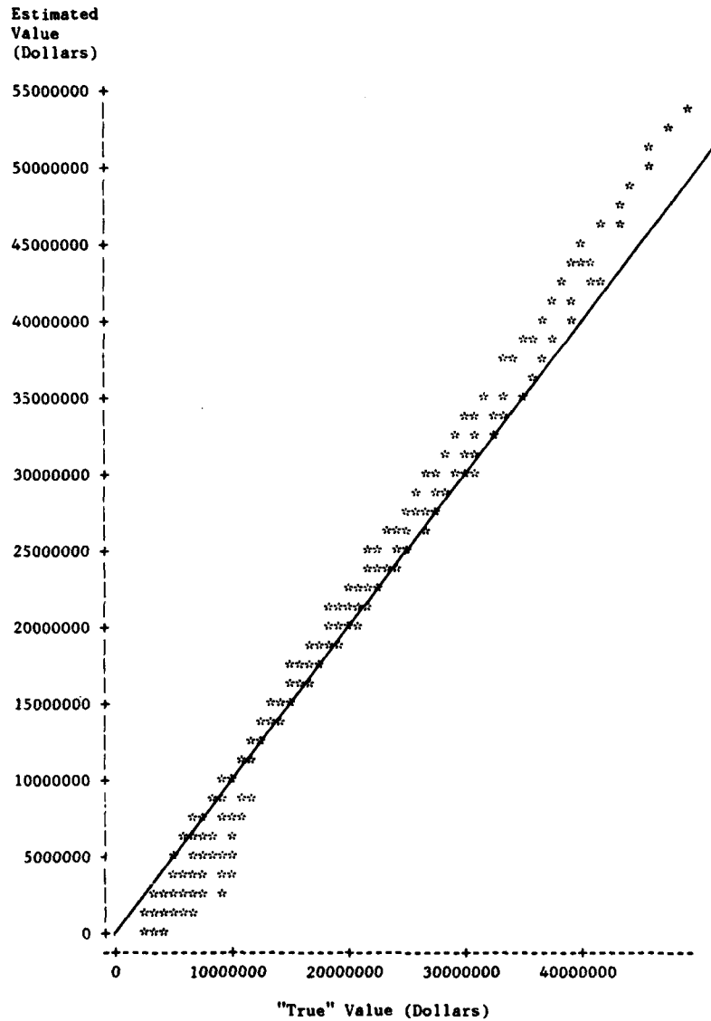
Fig. 7—Estimated vs "true" required buy of 1-2 year lead time items for the F100 engine alternative wartime programs
