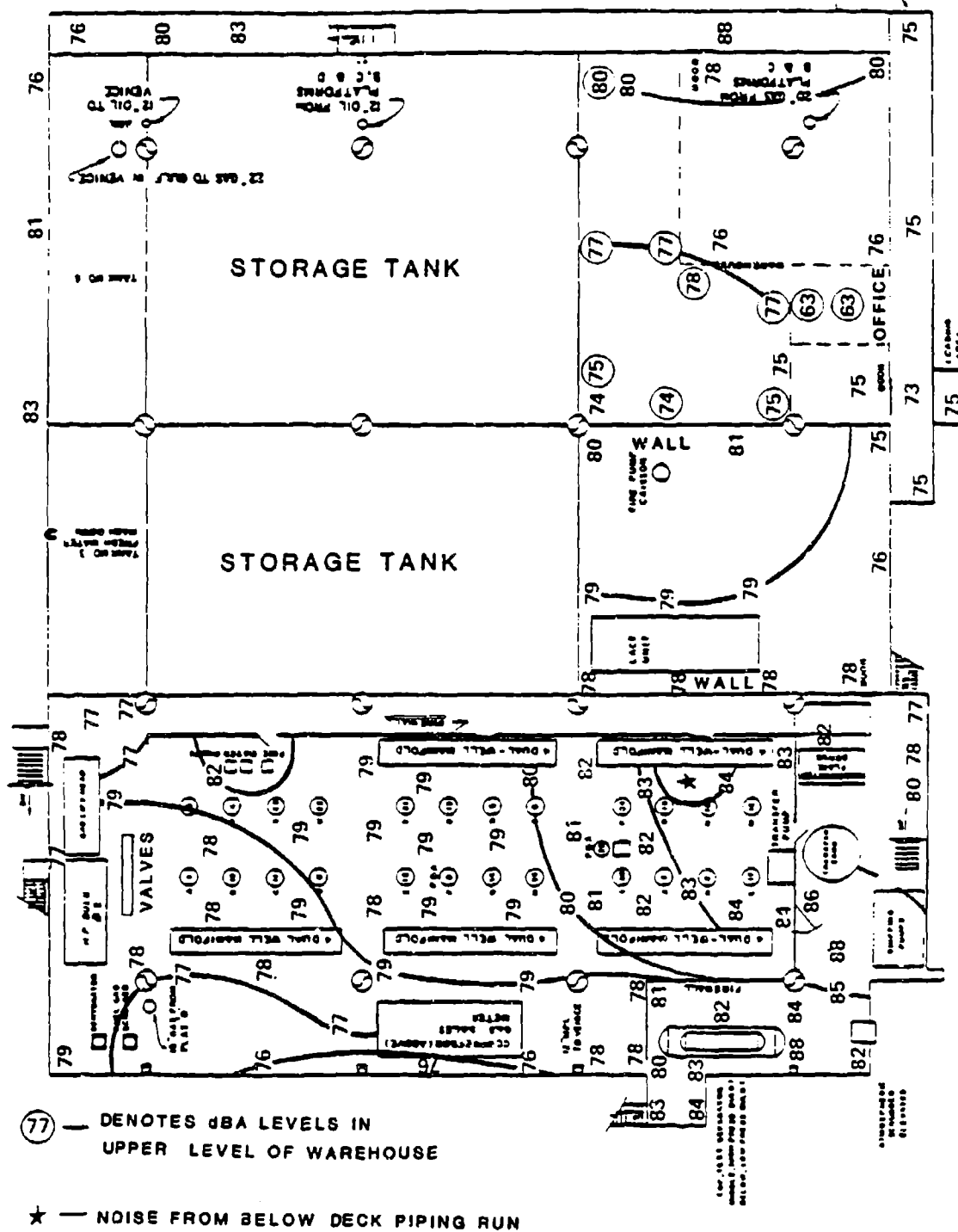
FIGURE A.4. LOWER LEVEL - PLATFORM NO. 1 SOUND PRESSURE LEVEL CONTOURS IN dB(A)
