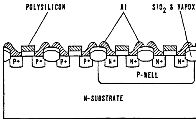
Figure 3b. The Fairchild Isoplaner C-CMOS process utilizing local oxide isolation in place of diffused channel stops (Ref. 2).
