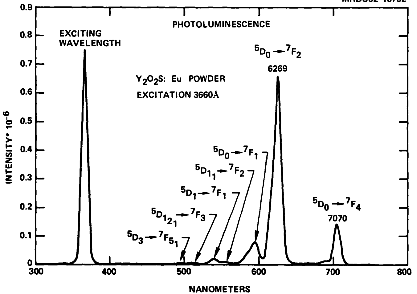
Fig. 7 Photoluminescent spectrum of yttrium oxysulfide europium powder used as CRT phosphor.
