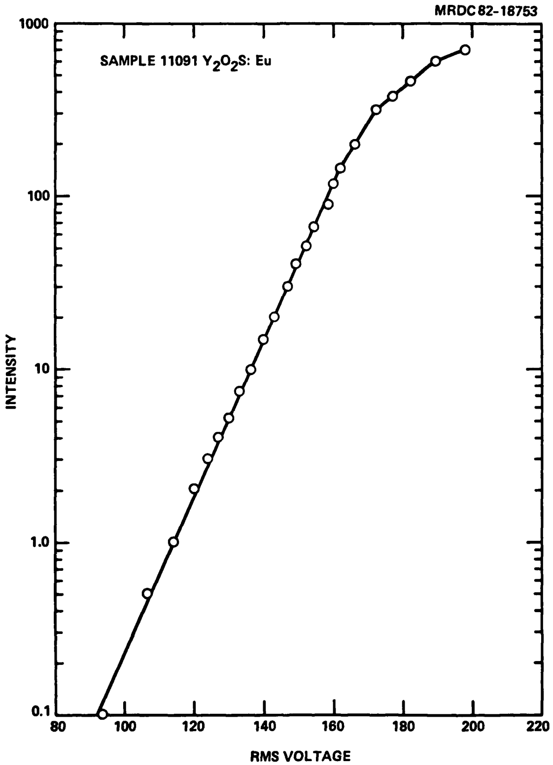
Fig. 11 Brightness-voltage curve for Y_2O_2S:Eu^{+3} thin film emitter.
