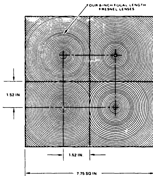
Figure 44. Fresnel Field Lens, Direct Light From Four Projection Modules to Single Exit Pupil
