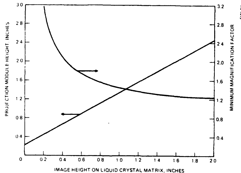
Figure 40. Projection Module Height and Minimum Magnification Factor for 100 Element-Per-Inch Two-Matrix Display
