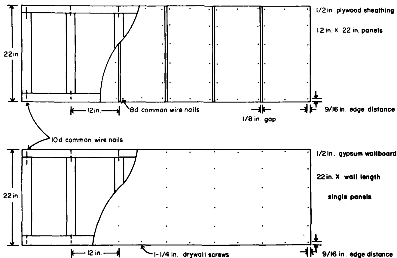
Figure 1.--Typical wall construction used in wall racking test (6-foot wall used for illustration). (ML84 5245)
