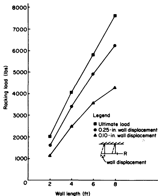
Figure 10.—Racking load versus wall length for double-sided plywood-gypsum walls at 0.10-, 0.25-inch horizontal wall displacements and at ultimate load. (ML84 5253)
