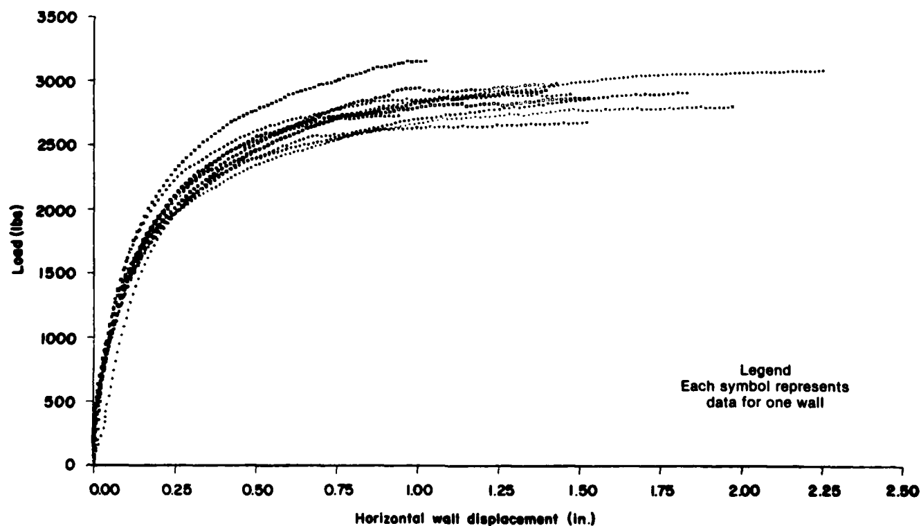
Figure 4.--Load versus horizontal wall displacement for 10 plywood one-sided walls 4 feet in length. (ML84 5247)
