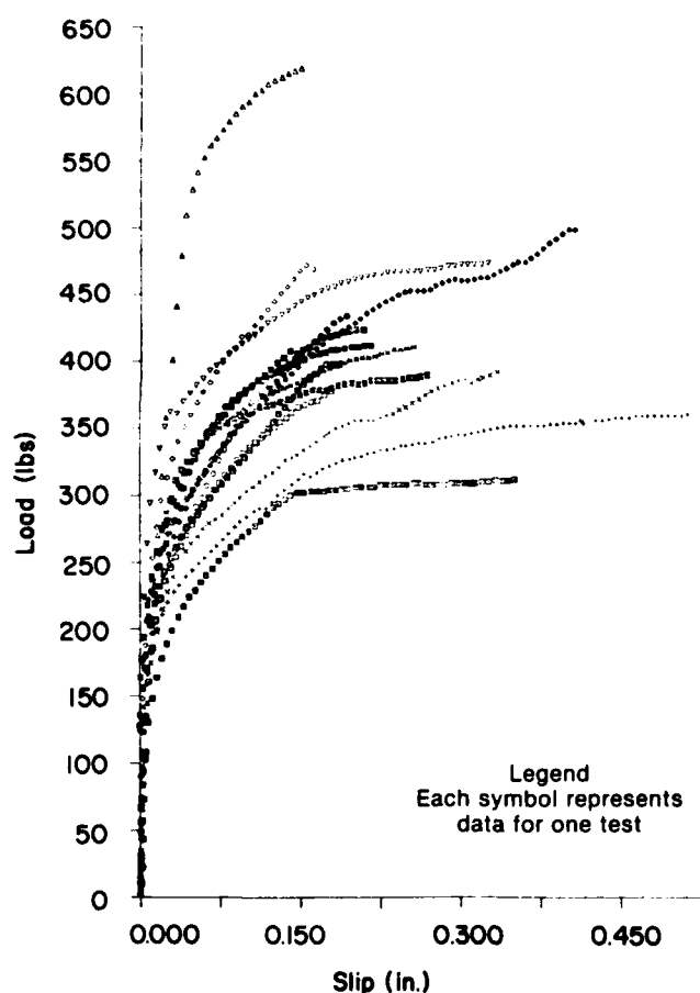
Figure B-1.--Load versus slip for 8d common wire nails and 1/2-inch plywood. (ML84 5254)
