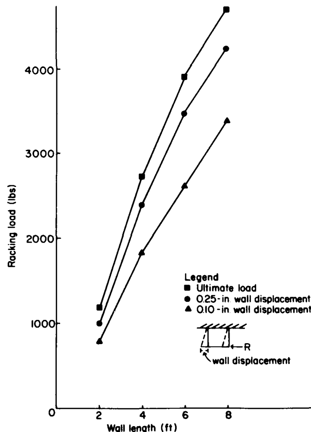
Figure 9.--Racking load versus wall length for double-sided gypsum-sheathed walls at 0.10-, 0.25-inch horizontal wall displacements and at ultimate load. (ML84 5252)
