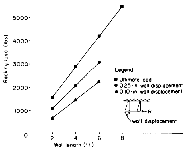
Figure 6.--Racking load versus wall length for single-sided plywood-sheathed walls at 0.10-, 0.25-inch horizontal wall displacements and at ultimate load. (ML84 5249)
