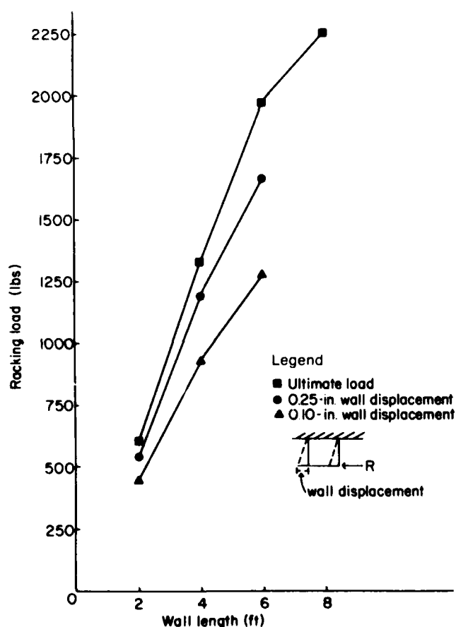
Figure 8.--Racking load versus wall length for single-sided gypsum-sheathed walls at 0.10-, 0.25-inch horizontal wall displacements and at ultimate load. (ML84 5251)
