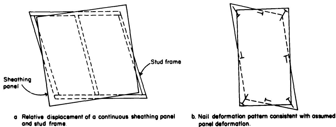
Figure 2.--Nail deformation pattern during wall racking tests. (ML84 5246)
