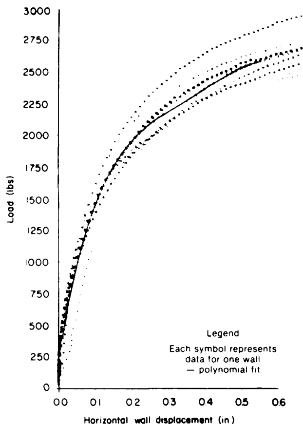
Figure 5.--Load versus horizontal wall displacement for 10 plywood one-sided walls 4 feet in length with polynomial fit. Points from polynomials are used to compare wall types and lengths. (ML84 5248)
