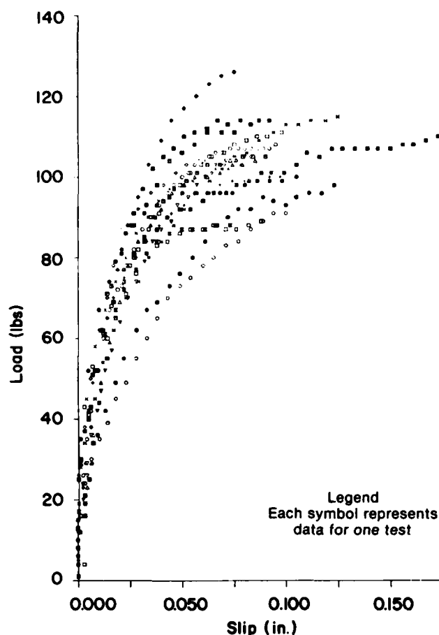
Figure B-2.--Load versus slip for 1-1/4-inch drywall screws and 1/2-inch gypsum. (ML84 5255)
