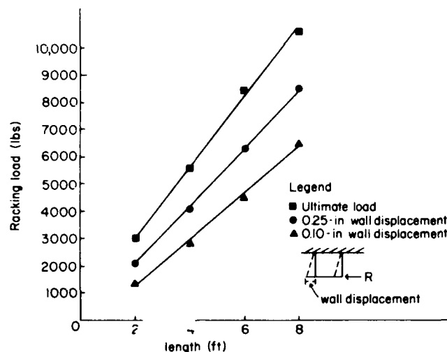
Figure 7.--Racking load versus wall length for double-sided plywood-sheathed walls at 0.10-, 0.25-inch horizontal wall displacements and at ultimate load. (ML84 5250)
