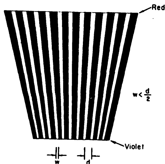
Figure 4(b). A source encoding mask.
