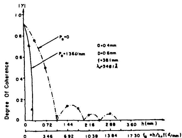
Fig. 12. Plots of degree of coherence along the \alpha direction as a function of slit separation h for two values of sampling grating frequency p_0 .
