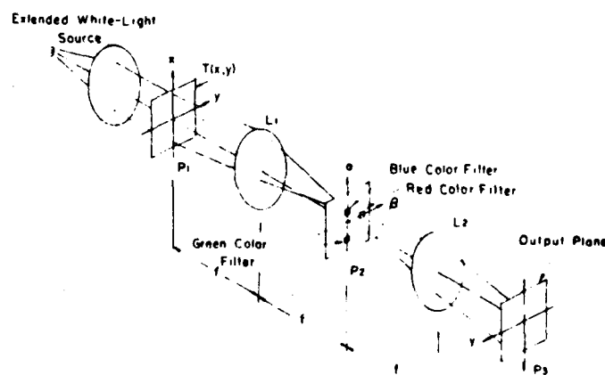
FIG. 2. A white-light pseudocolor encoder
