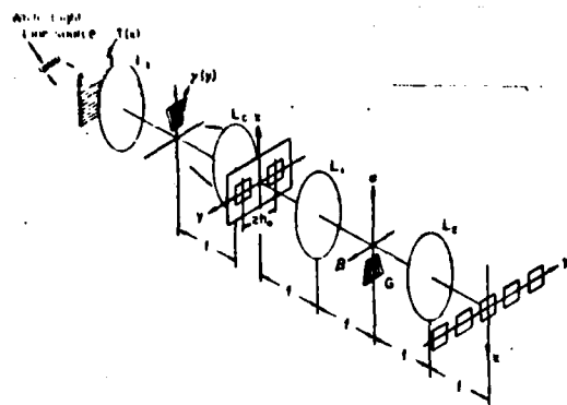
FIG. 3. — A white-light image subtraction processor. T(x) : phase grating, L_1 : image lens, L_2 : collimated lens, L_3 and L_4 : achromatic transform lenses, G : source encoding mask, G : fan-shape diffraction grating.
