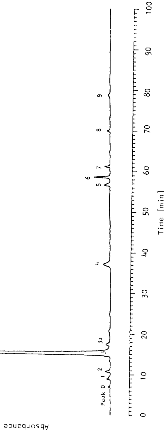
Figure 5: High pressure liquid chromatographic separation of a chloroethyl ethyl sulfide-deoxyguanosine reaction mixture. A sample containing 20 µg of nucleosides was separated on a 5 µm Spherisorb column (4.6 x 250 mm) at a flow rate of 1 ml/min with 3% acetonitrile in 25 mM \text{KH}_2\text{PO}_4 , pH 4.5, and then with a 3-30% gradient of acetonitrile in the same buffer for 50 min, and finally with 30% acetonitrile in buffer for 25 min. Peak 3 is unmodified deoxyguanosine and peak 8 is O 6 -ethylthioethyl deoxyguanosine.
