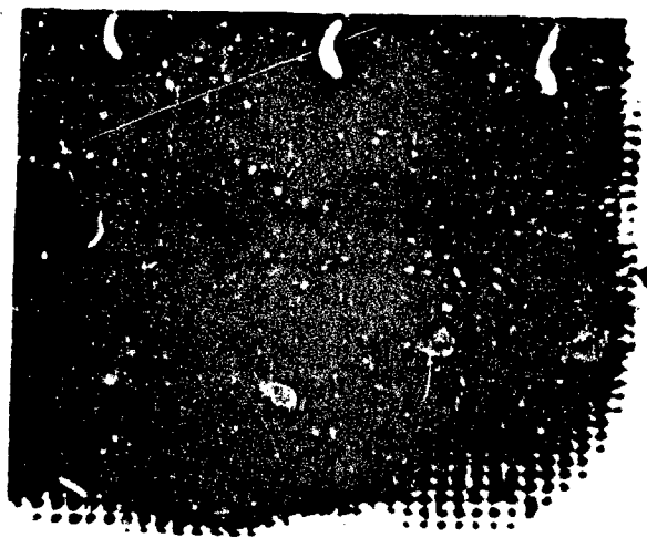
Figure 13. Damage Regions on Silicon Wafer with about 2 \text{ J/cm}^2 Input Energy Density at 532 nm. Nominal Mag. 65X
