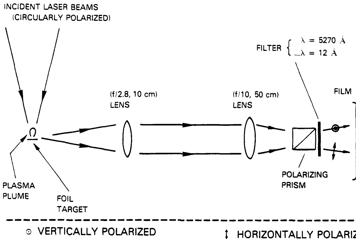
Figure 1 Experimental arrangement for making spatially-resolved, time-integrated observations of emission at the second-harmonic wavelength.
