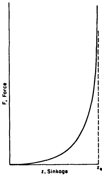
Figure 3. Idealized force vs sinkage curve generated by a plate-sinkage device in shallow snow.
