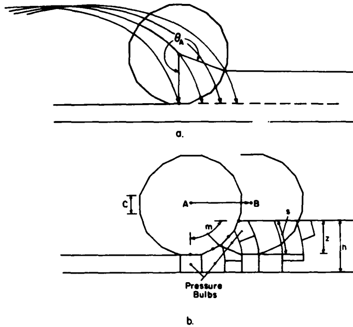
Figure 4. Sinkage path (a) and pressure bulb development (b) beneath a wheel made of plates.
