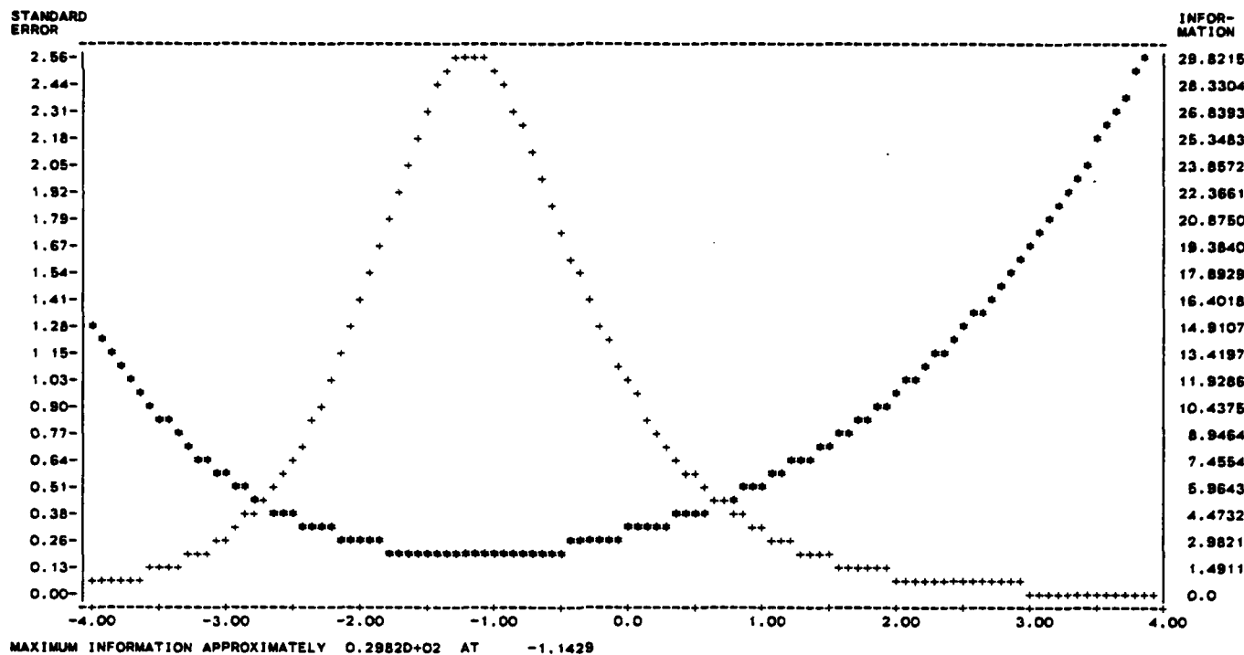
EXHIBIT 1-3 TEST INFORMATION AND STANDARD ERROR CURVES FOR WORD KNOWLEDGE; 2-PARAMETER LOGISTIC MODEL
