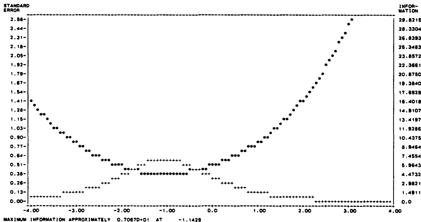
EXHIBIT 1-4 TEST INFORMATION AND STANDARD ERROR CURVES FOR PARAGRAPH COMPREHENSION; 2-PARAMETER LOGISTIC MODEL
