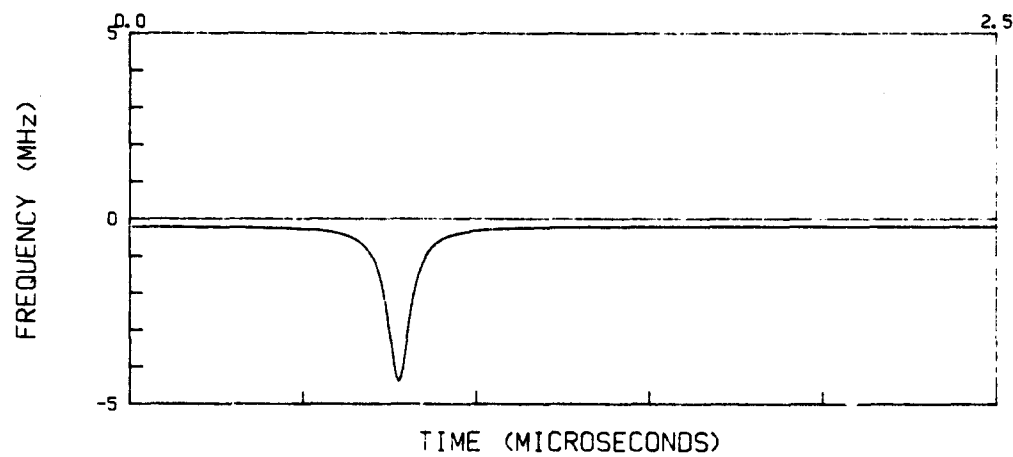
Figure A-11. Demodulator Output ( N=1.1S ).
