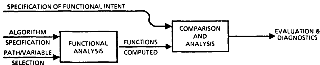
Figure 4.2-4. General Form of a Formal Functional Analysis
