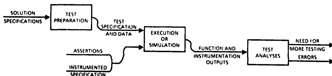
Figure 4.2-3. General Form of Dynamic Analysis
