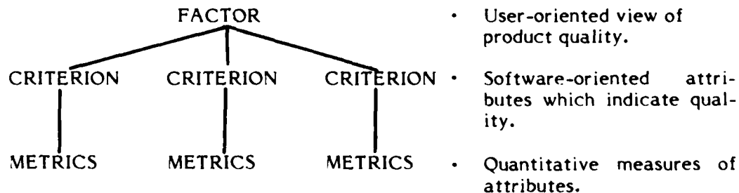
Figure 4.3.1.4-2. Software Quality Metrics Framework
