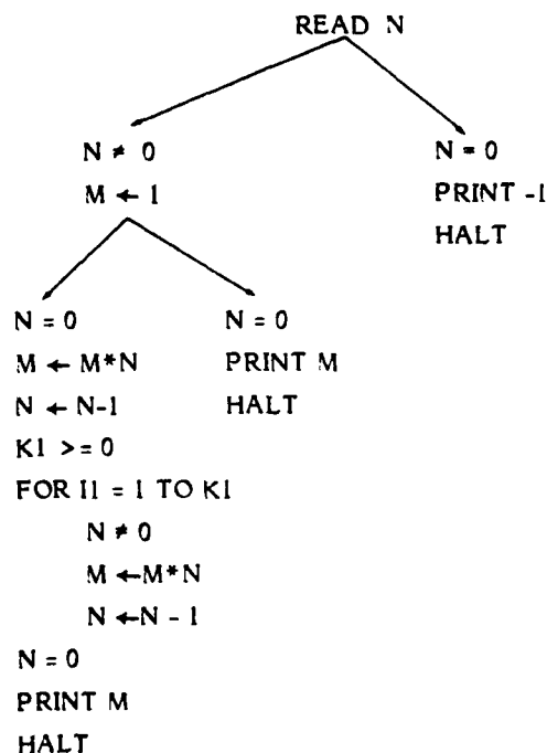
Figure 4.3.1.5-2. Description Tree
