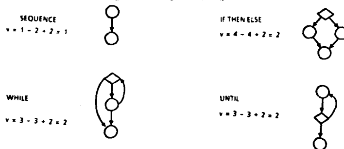
Figure 4.3.1.4-1. Control Graphs of Language Structures
