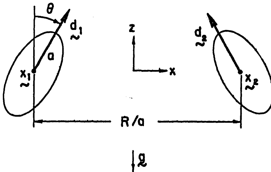
Figure 7. Mirror symmetry geometry of two inclined spheroids with their axes in a vertical plane
