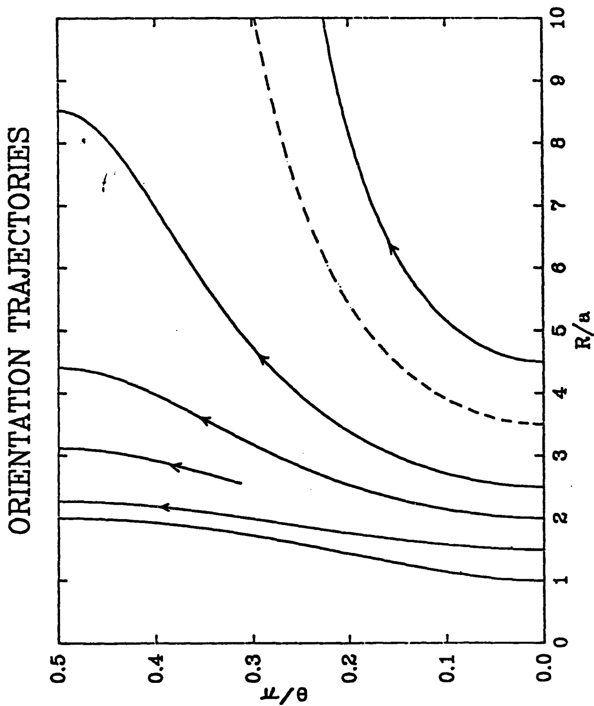
FIGURE 9. Evolution of orientation and separation for two spheroids, aspect ratio = 2, falling as in Figure 7.
