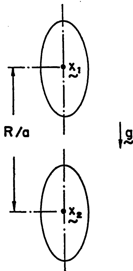
FIGURE 2. Sedimentation of two identical spheroids falling along their line of centers.
