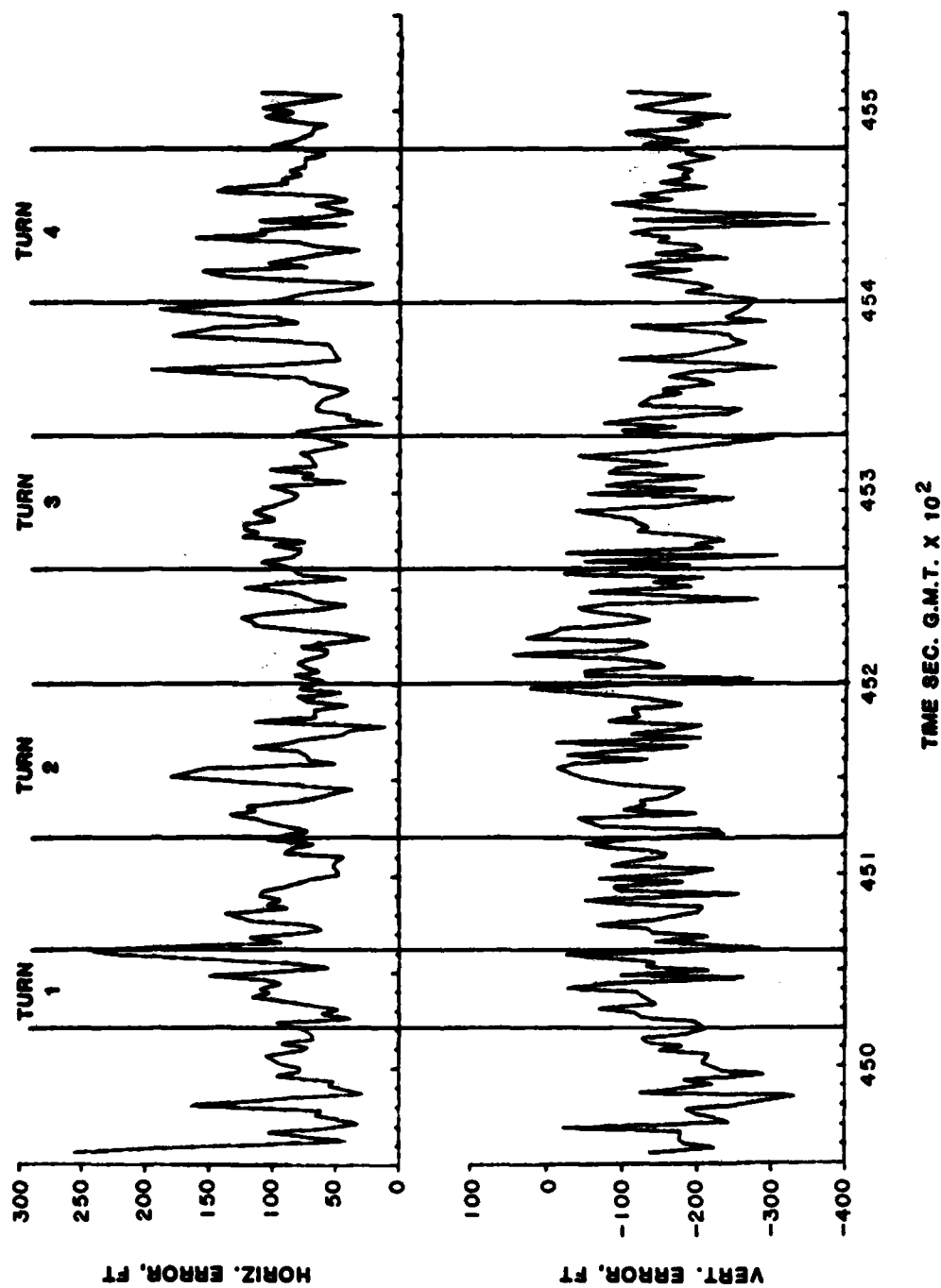
FIG. 4-89. POSITION FIX ERRORS FOR HOLDING PATTERN, 4 FEB 83, RUN 1a
