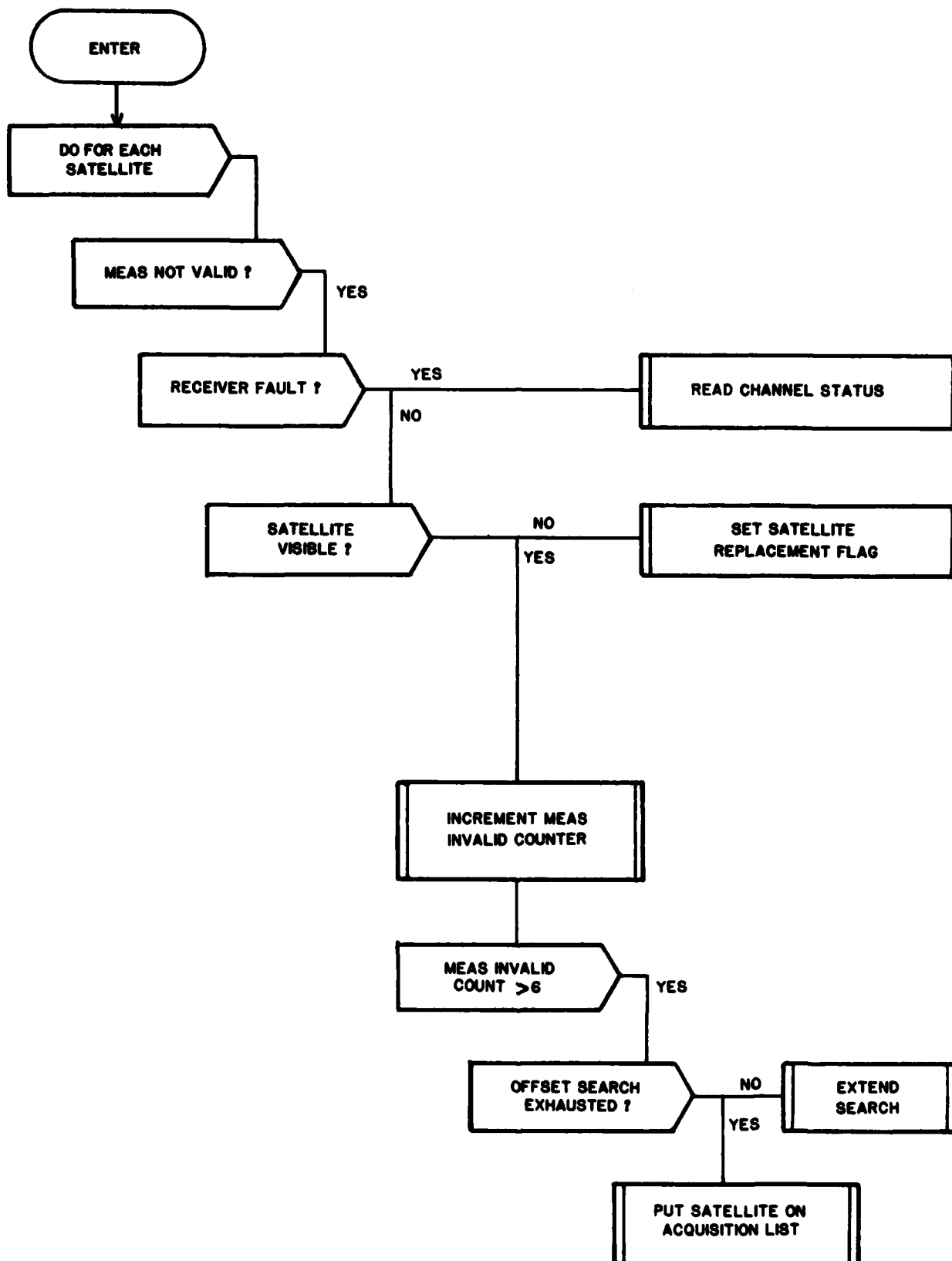
FIG. 3-26. LOSS OF LOCK ALGORITHM
