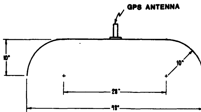
ELEVATION VIEW
