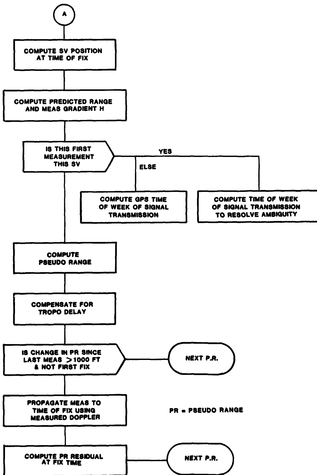
FIG. A-1. POSITION FIX ALGORITHM (CONT.)
