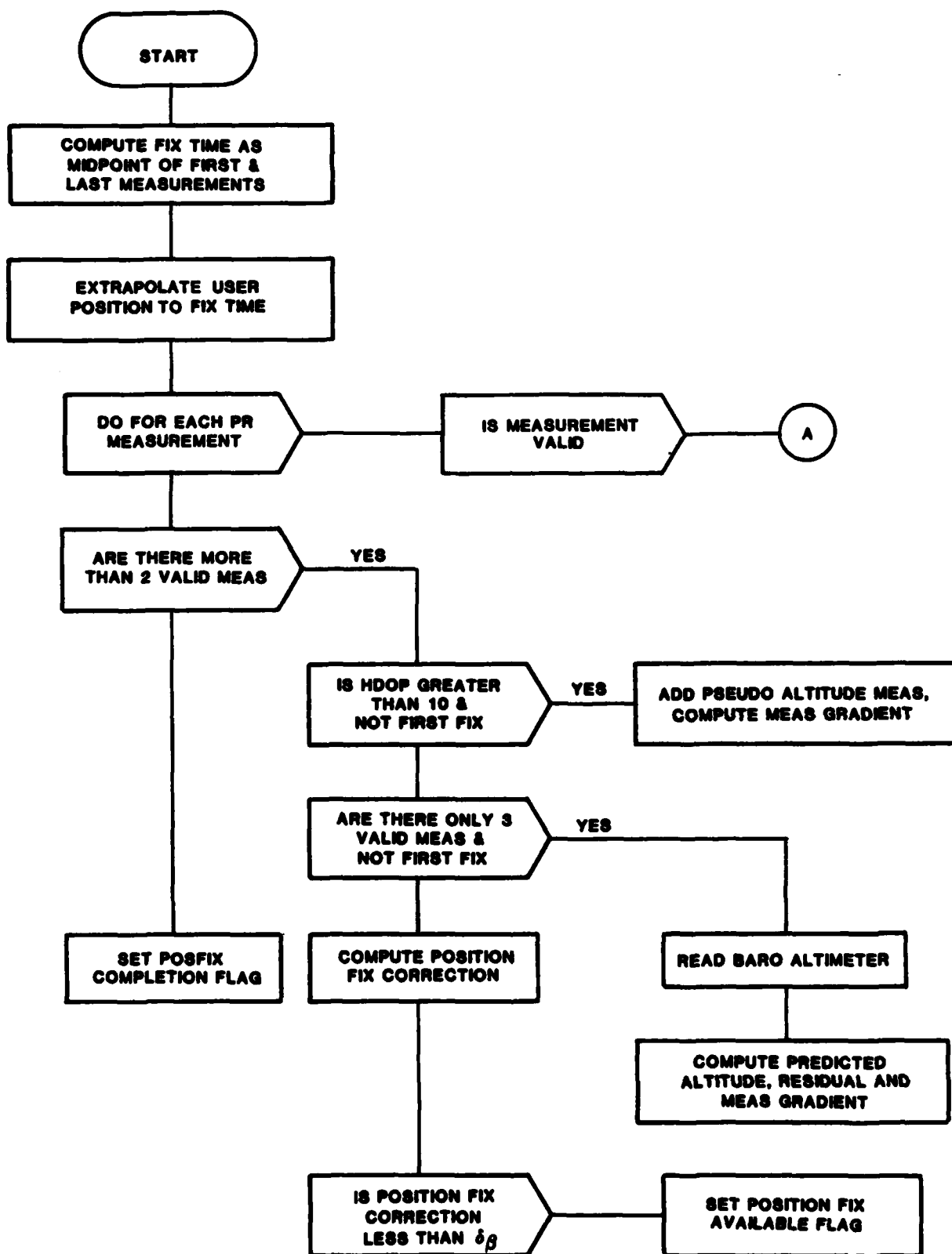
FIG. A-1. POSITION FIX ALGORITHM
