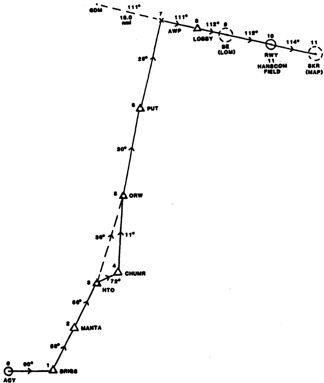
FIG. 3-36. SAMPLE FLIGHT PLAN: ATLANTIC CITY TO HANSCOM FIELD
