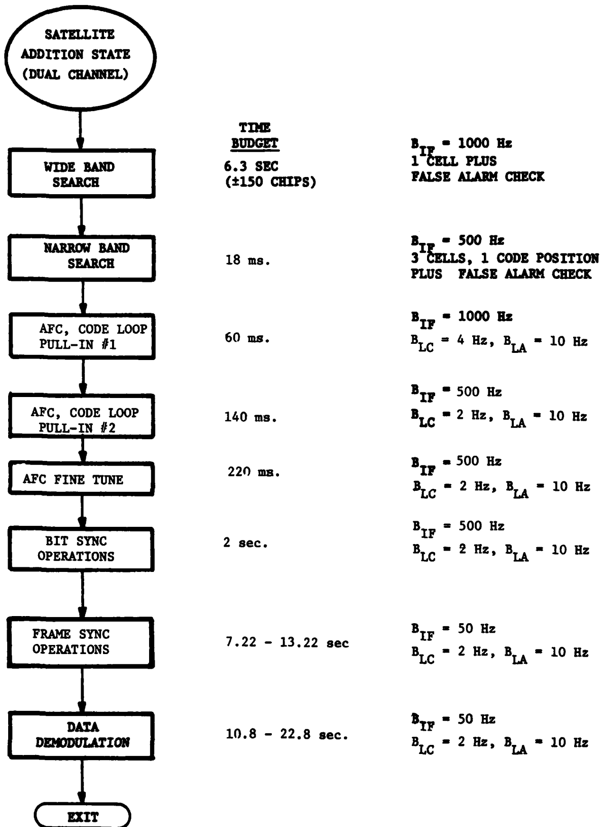
FIG. 3-19. Satellite Addition State Diagram.
