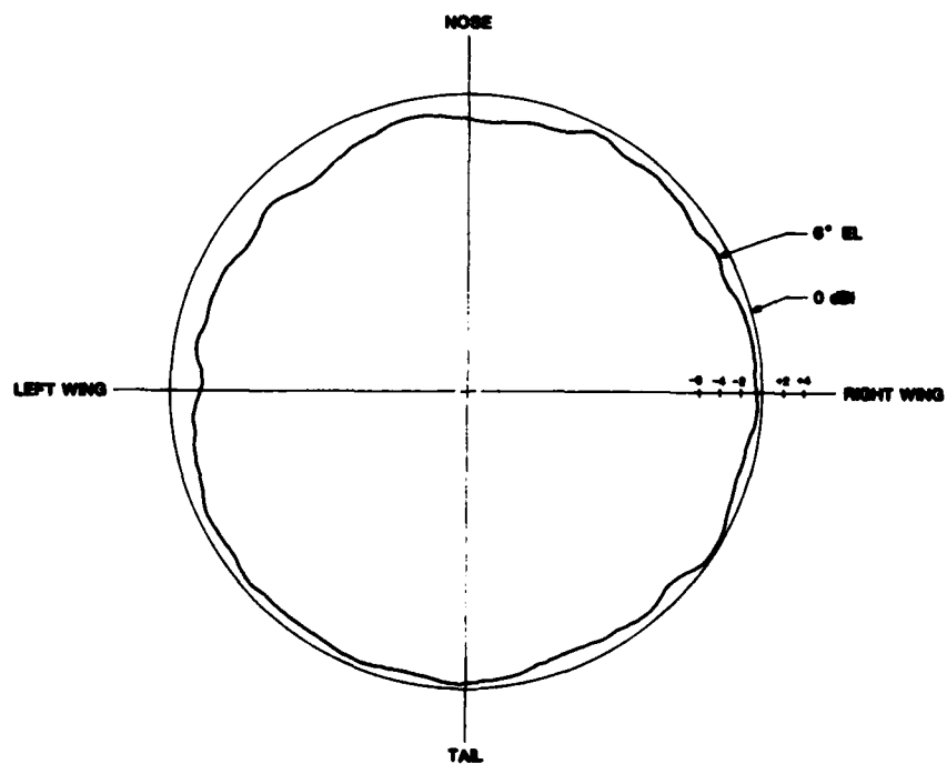
FIG. 4-12. Gain vs. Azimuth for Elevation Cuts at +6° and +17°; Chu Model CA-3224 Volute Antenna.
