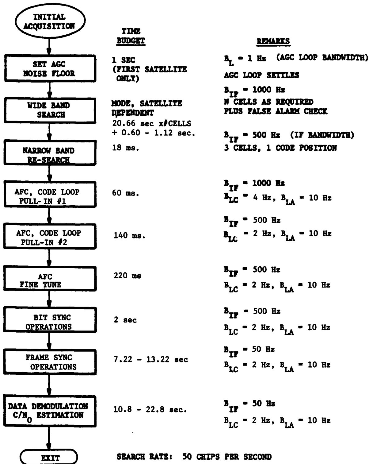
FIG. 3-16. Receiver Acquisition State Diagram.
