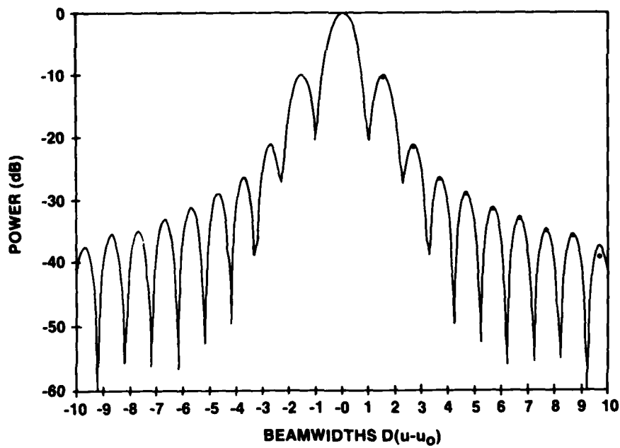
Figure 7b. Pattern in the v -plane Through the Main Beam at u_0 = 0.05 , v_0 = 0
