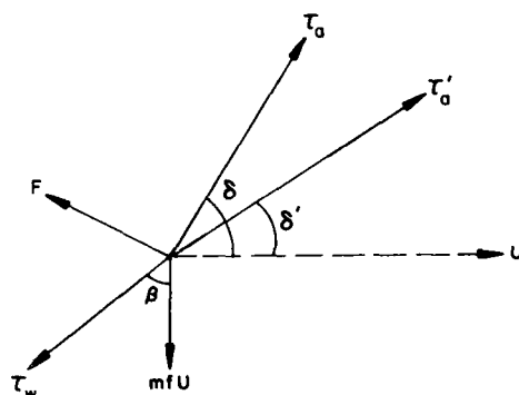
Figure 4. If the wind stress \tau_a balances the water drag, Coriolis and current forces, then a larger stress \tau'_a , turned further to the right, is required to balance the forces with the addition of a force F due to internal ice stress.
