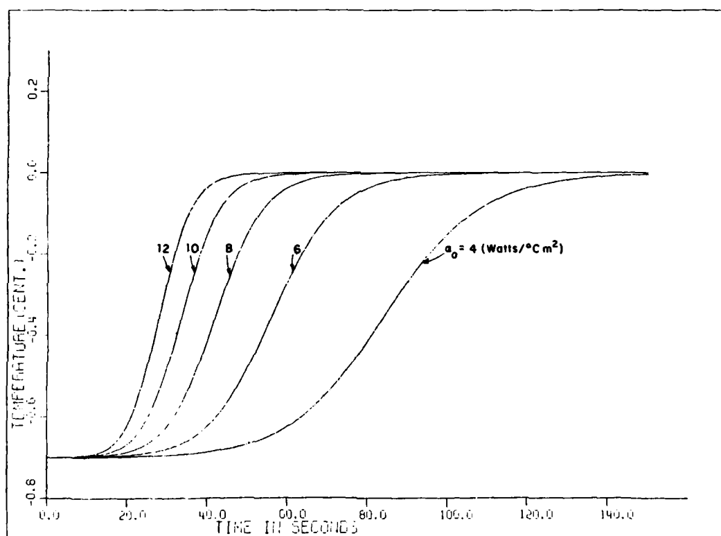
Figure C2. Variation of temperature rise attributable to frazil ice formation with initial value of heat-transfer coefficient, \alpha_o . Grid heating \dot{T} = 0 . Initial temperature of supercooling is T_o .
