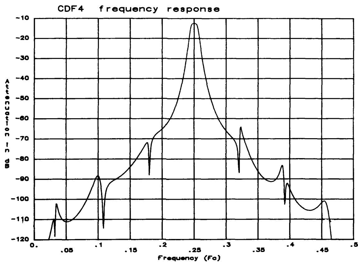
Figure 9.24. Bandpass filter frequency response.
