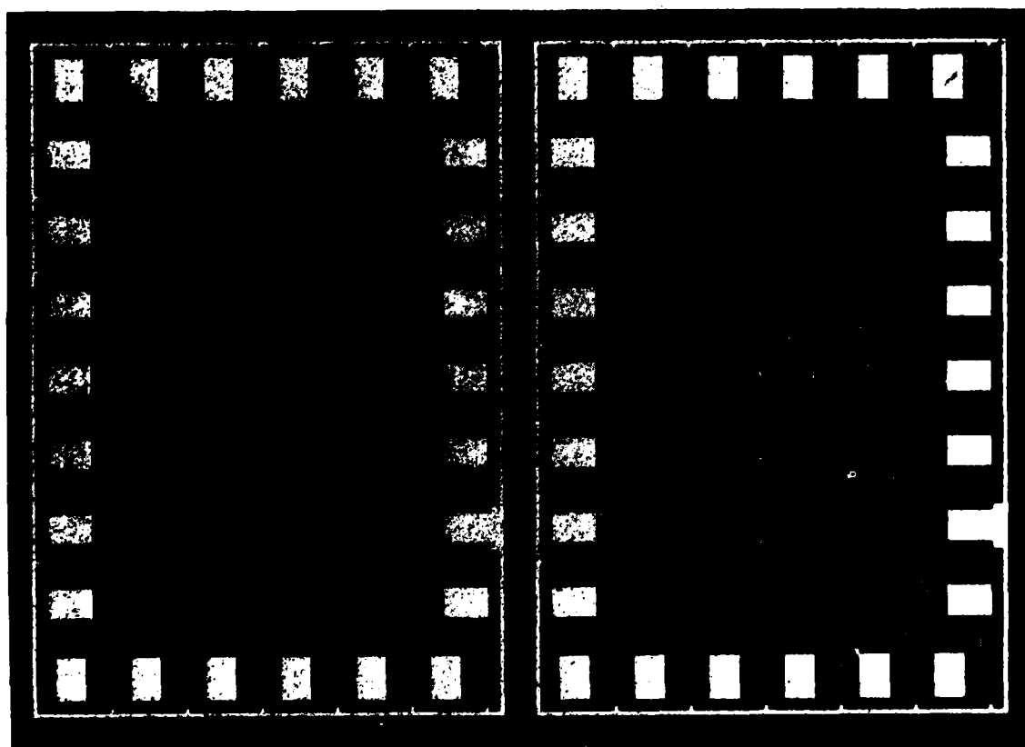
Figure 10.1c. PCDF1C = four stage split electrode filter using sequential splitters PCDF1D = flash splitter
