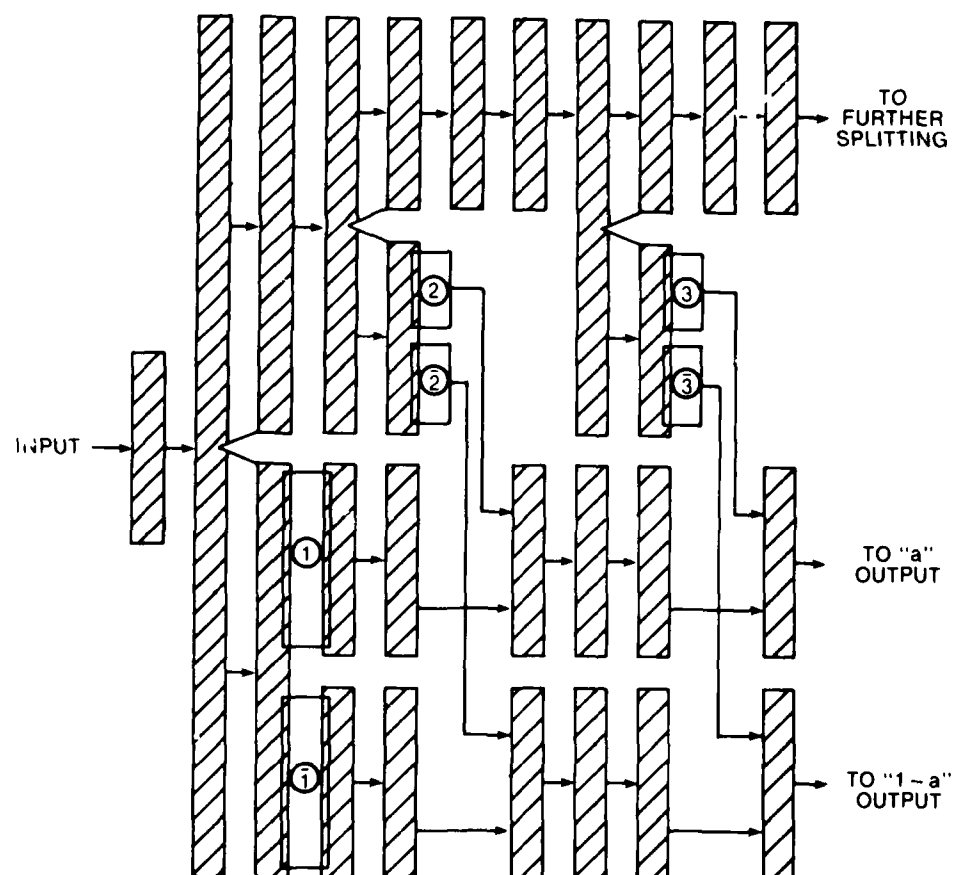
Figure 10.5. Pipelined charge splitter.
