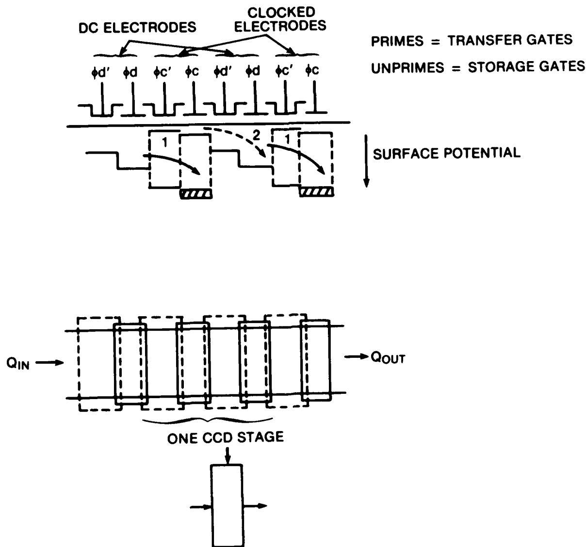
Figure 2.1. Pseudo one phase CCD operation.
