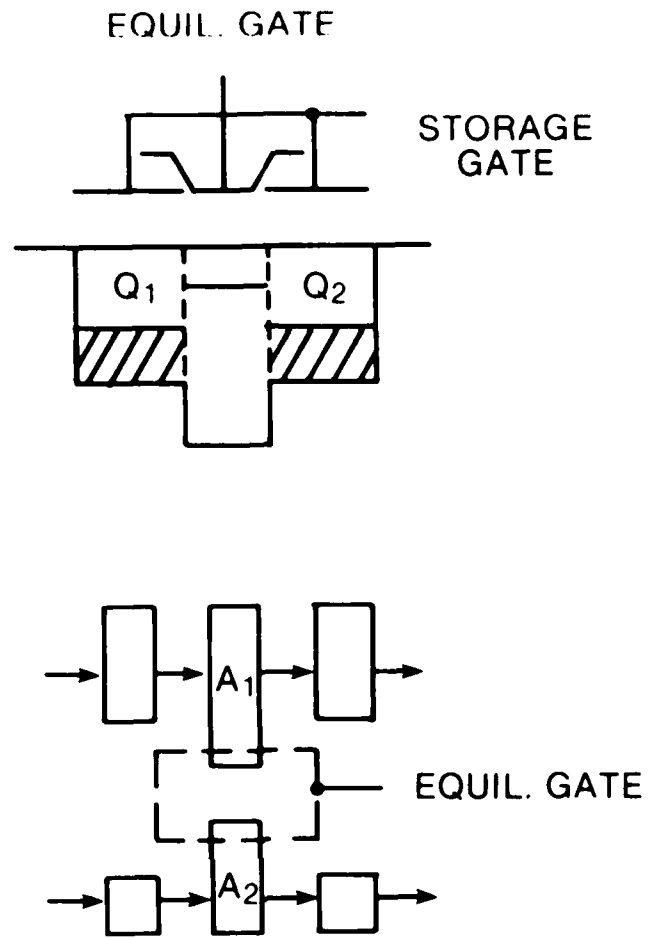
Figure 2.4. Gated equilibration charge splitting.
