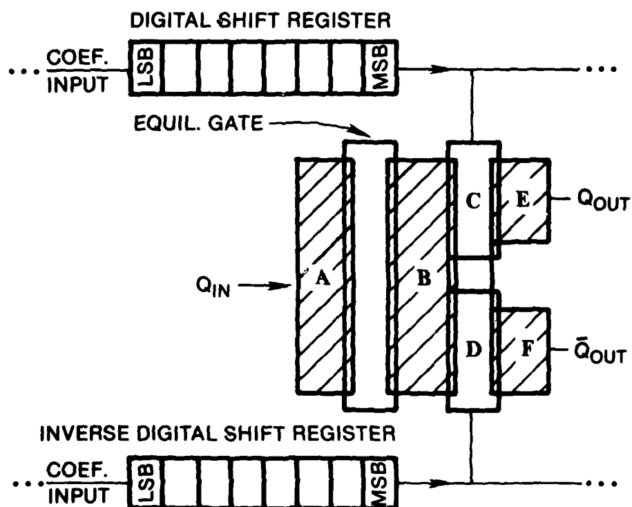
Figure 10.3. In-place sequential charge splitter.
