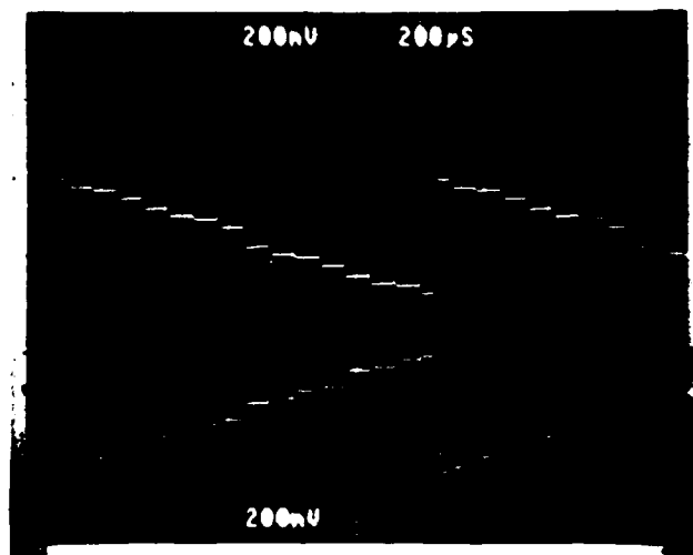
Figure 10.8. Flash charge splitter operated as a four bit MDAC.
