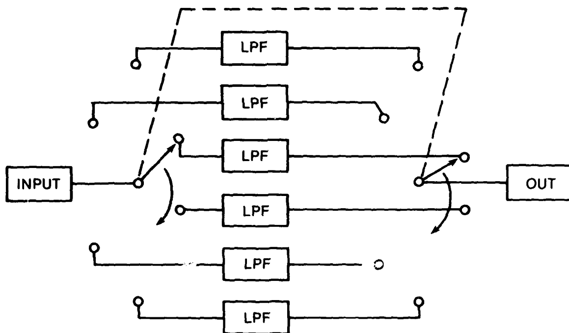
Figure 10.2. N-path filter.
