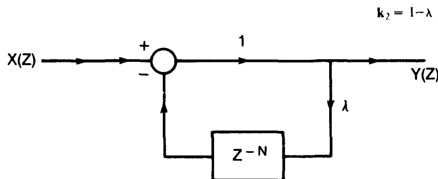
Figure 4.4. Recursive resonator block diagram.
