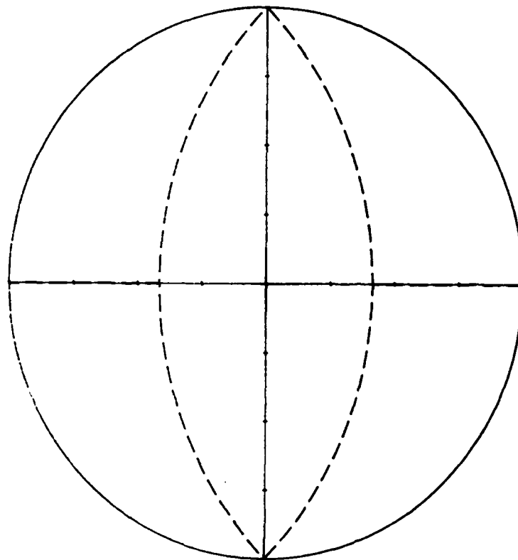
Figure 4.3. Allowable pole locations (inside the dashed lines) with a second order section in charge domain technology.
