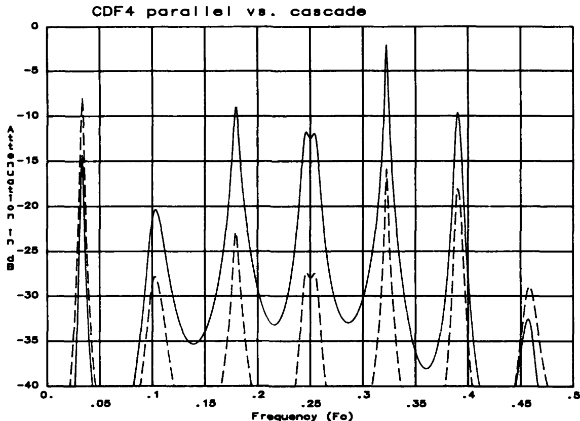
Figure 9.17. Frequency response for cascade (dashed) and parallel (solid) connection of the 89^\circ and 91^\circ pole sections.
