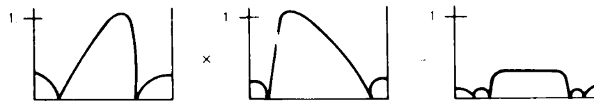
Figure 9.13. Minimizing insertion loss in charge domain filters.
