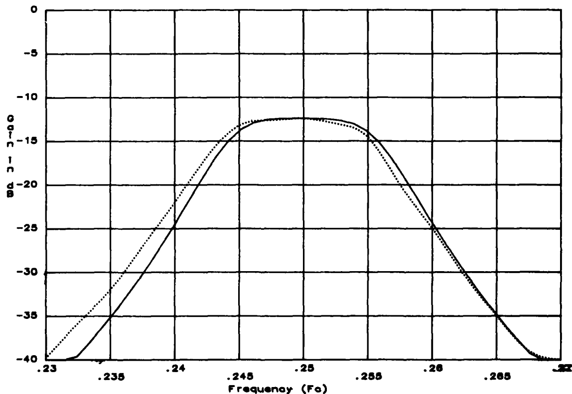
Figure 9.34. Comparison of theoretical (solid) and experimental (dotted) frequency responses for CDF4 - expanded view.
