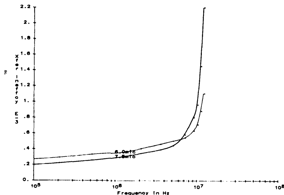
Figure 9.12 Charge transfer inefficiency vs. frequency for 6.0 micron and 7.5 micron processes.
