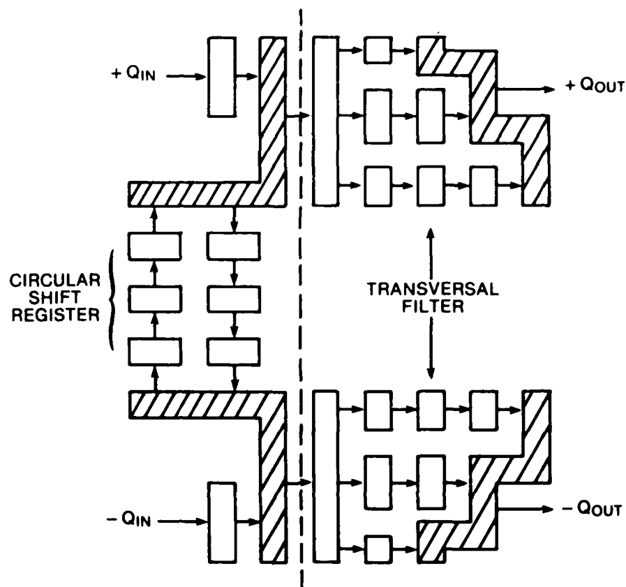
Figure 9.9a. "Form - C" structure for implementing complex pole pairs.
