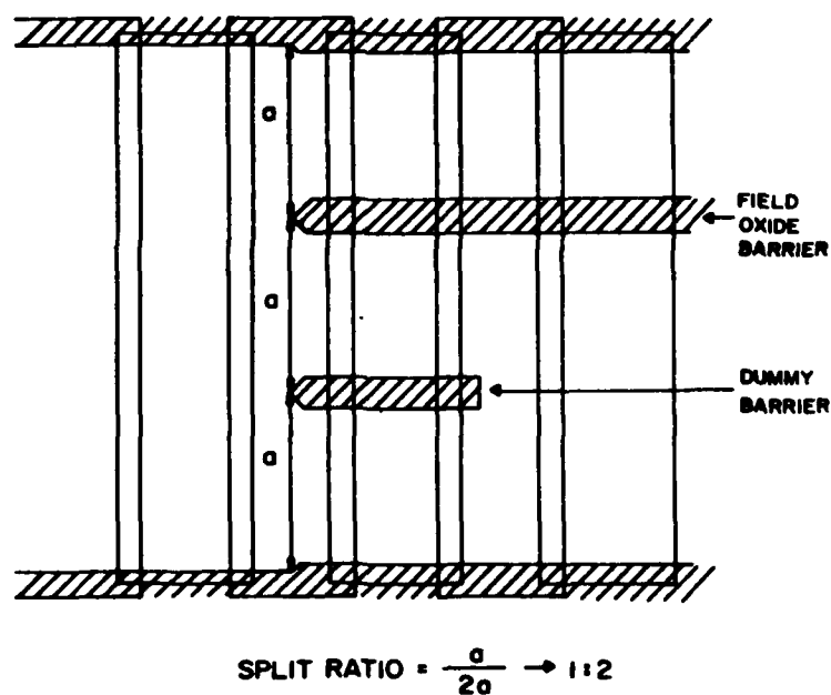
Figure 6.3. Charge splitting using dummy splitter.
