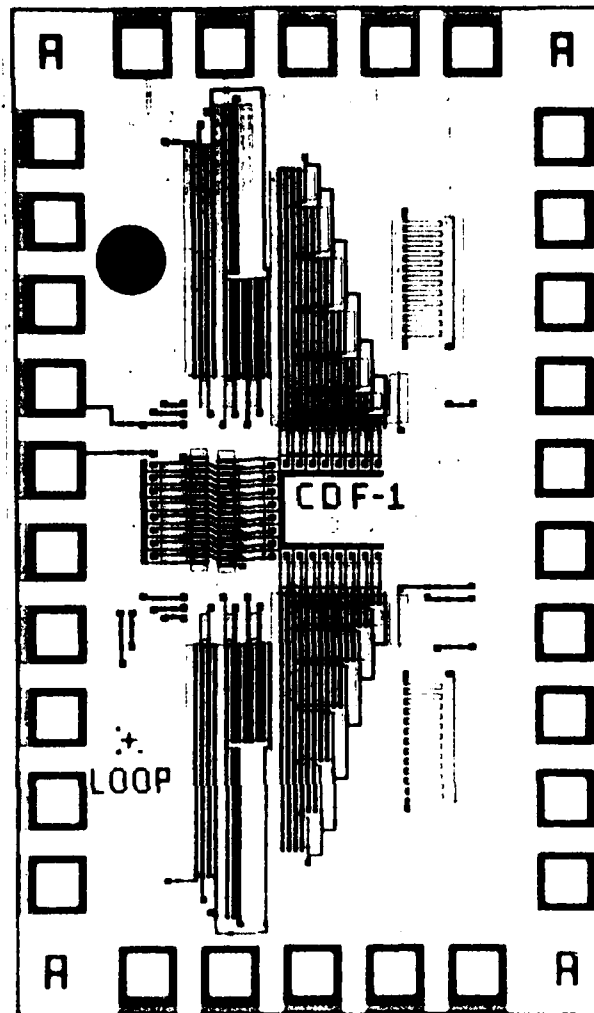
Figure 9.1. CDF1 photo micrograph.
