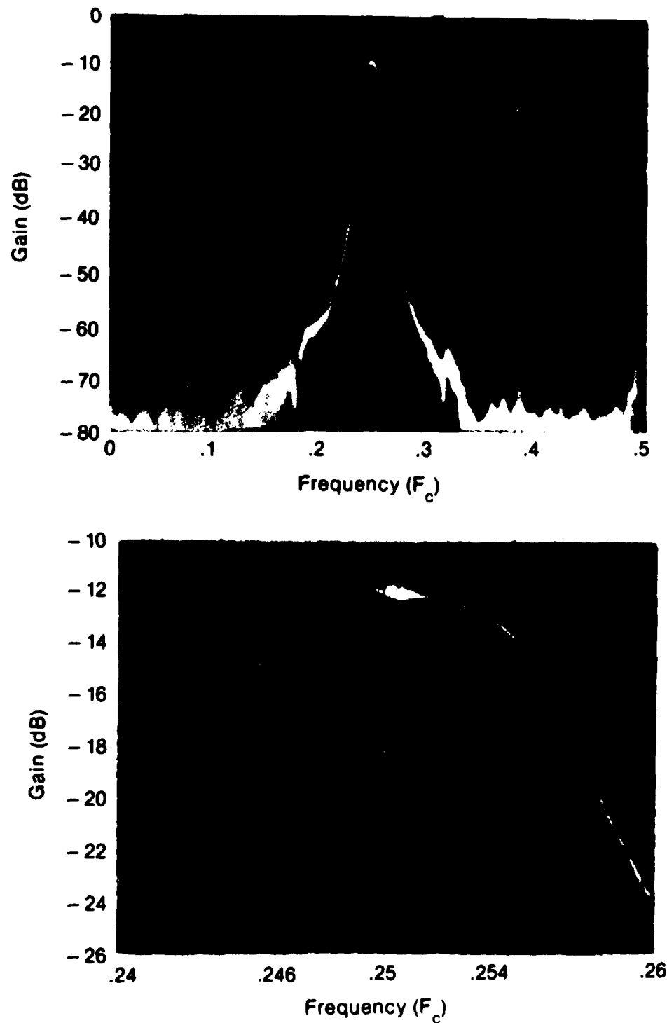
Figure 9.32. CDF4 experimental frequency response.
