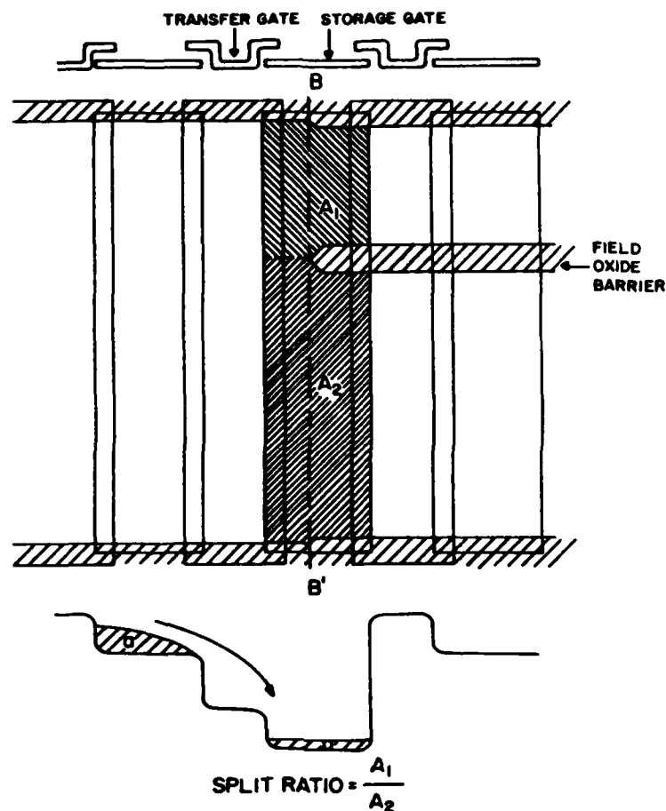
Figure 6.2. Pseudo-static barrier charge splitting.
