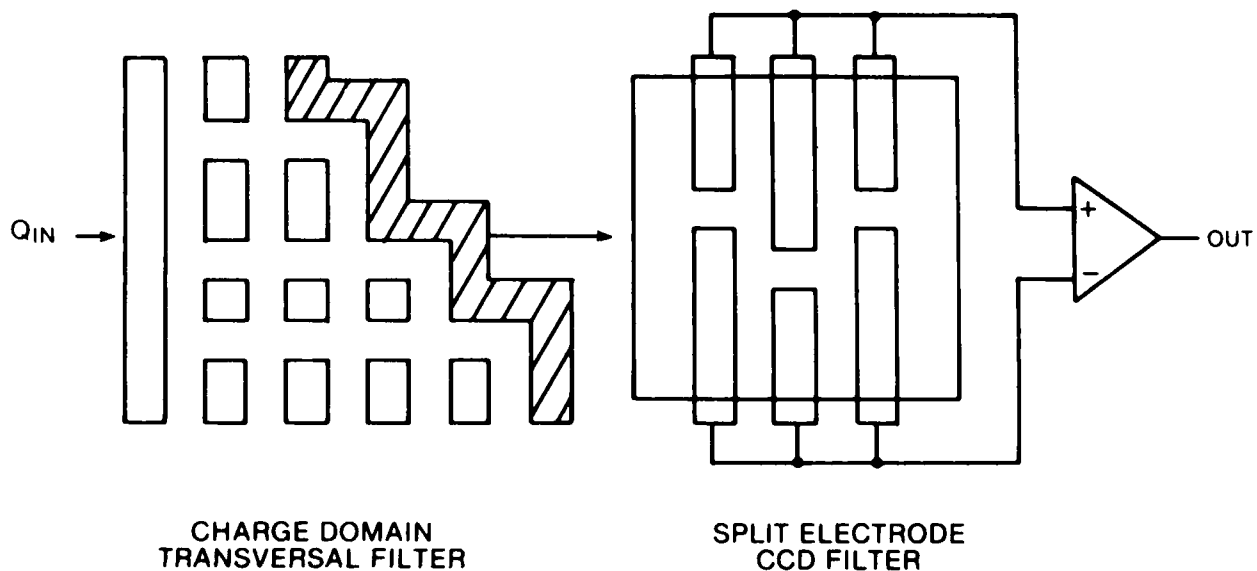
Figure 11.2. CDF/CCD hybrid device.
