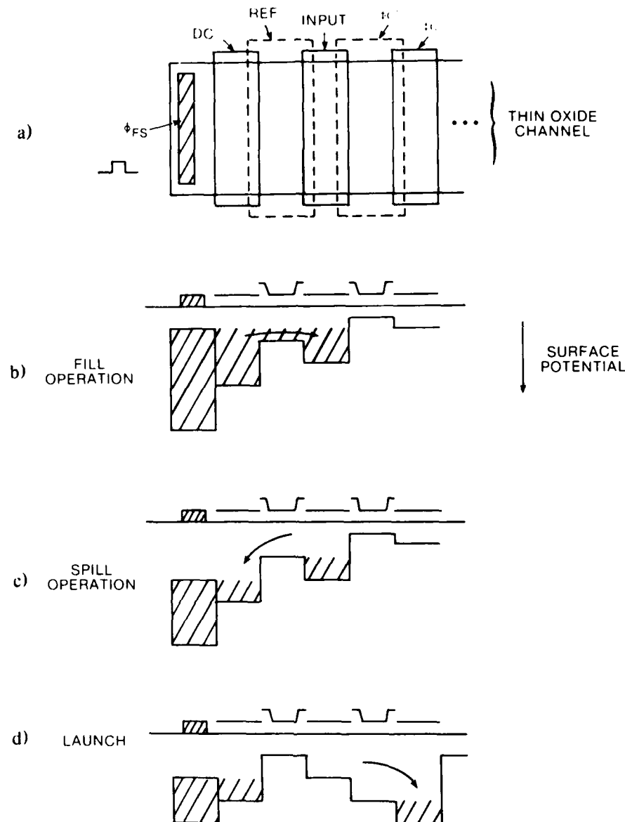
Figure 9.26. Fill and spill charge input circuit.
