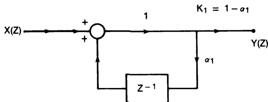
Figure 4.1. Recursive accumulator block diagram
