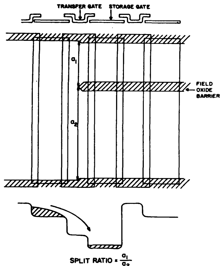
Figure 6.1. Dynamic barrier charge splitting.
