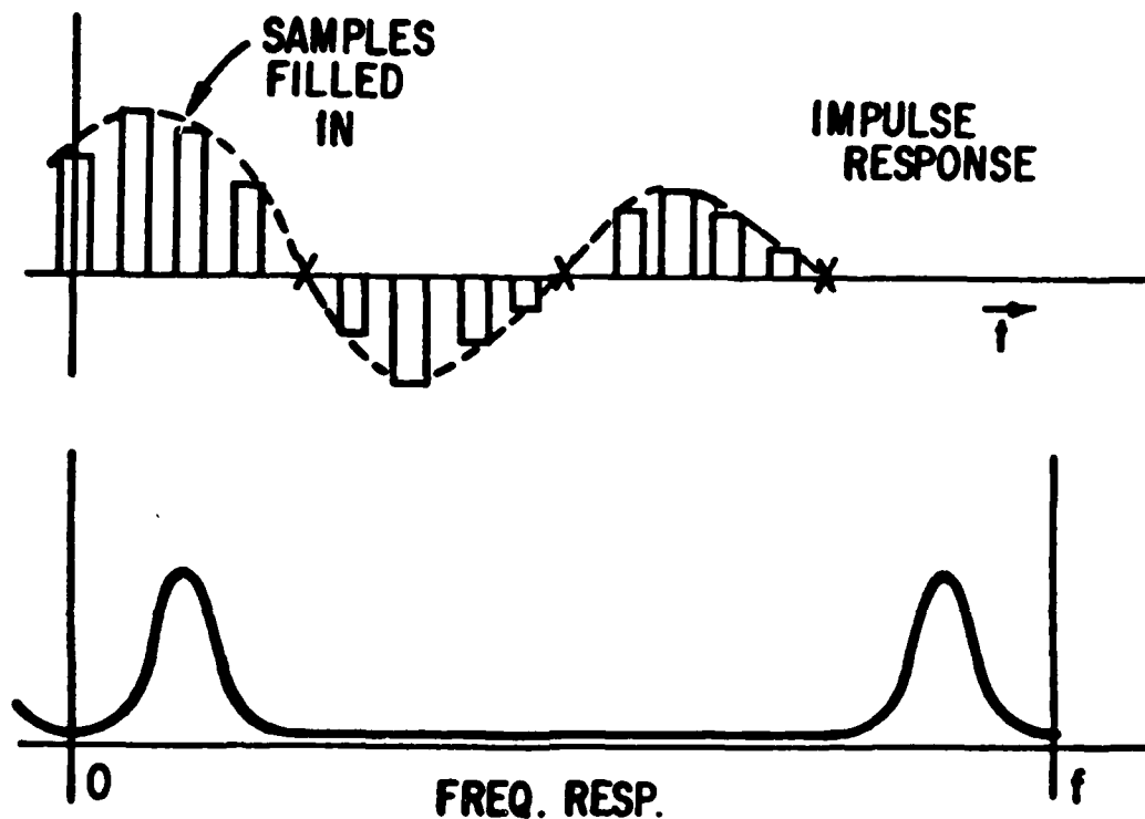
Figure 5.5. Complex pole pair impulse and frequency responses.
