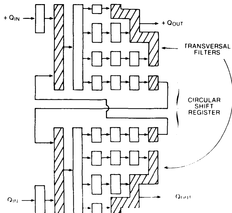
Figure 9.9b. Figure 8 structure for implementing complex pole pairs.
