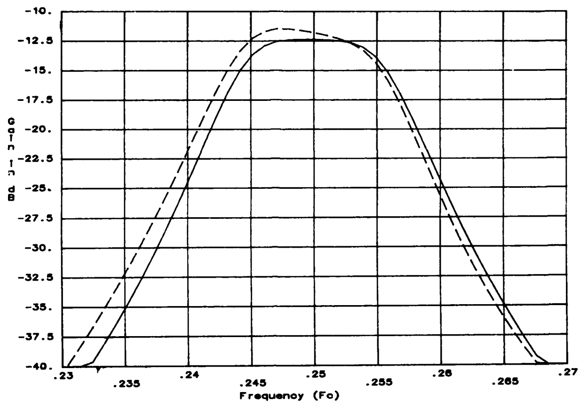
Figure 9.35. The effect of unequal charge packets transferred to the 89^\circ and 91^\circ pole sections on the passband of CDF4 for 0.0% error (solid curve) and 0.5% error (dashed curve).
