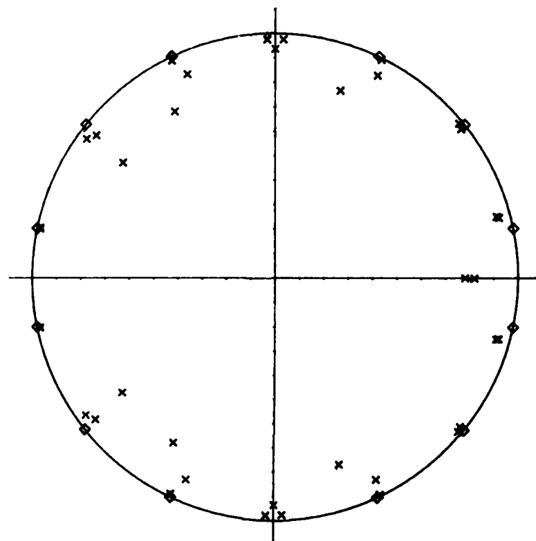
Figure 9.22. Z-plane pole-zero plot for charge domain bandpass filter.
