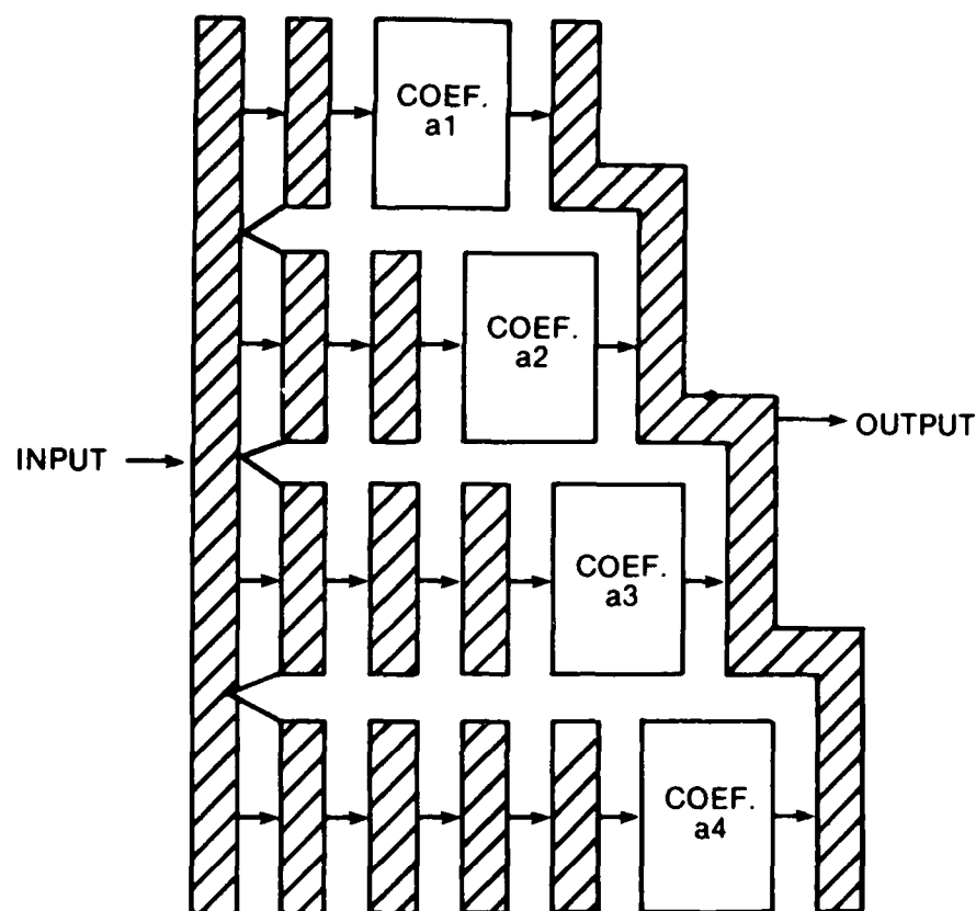
Figure 10.9. Pipe organ type programmable transversal filter.
