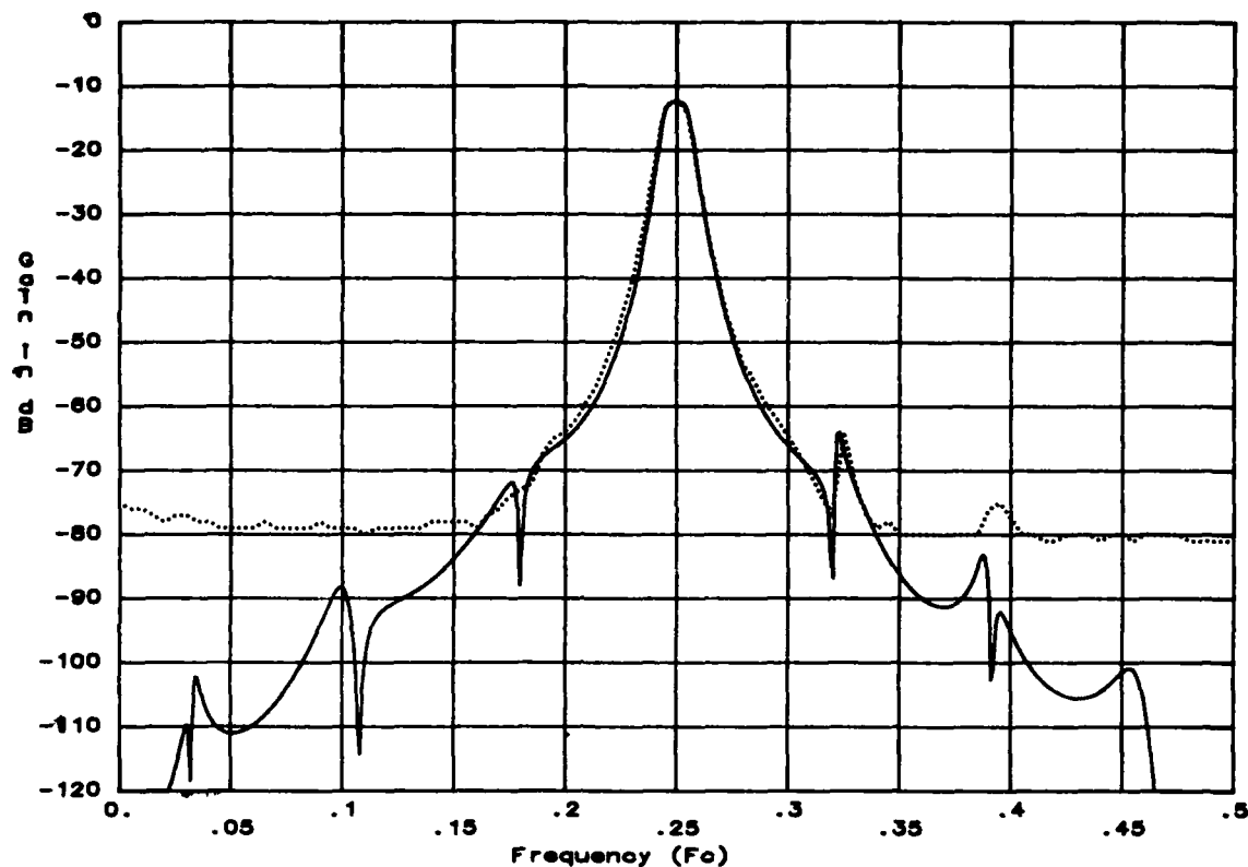
Figure 9.33. Comparison of theoretical (solid) and experimental (dotted) frequency responses for CDF4.
