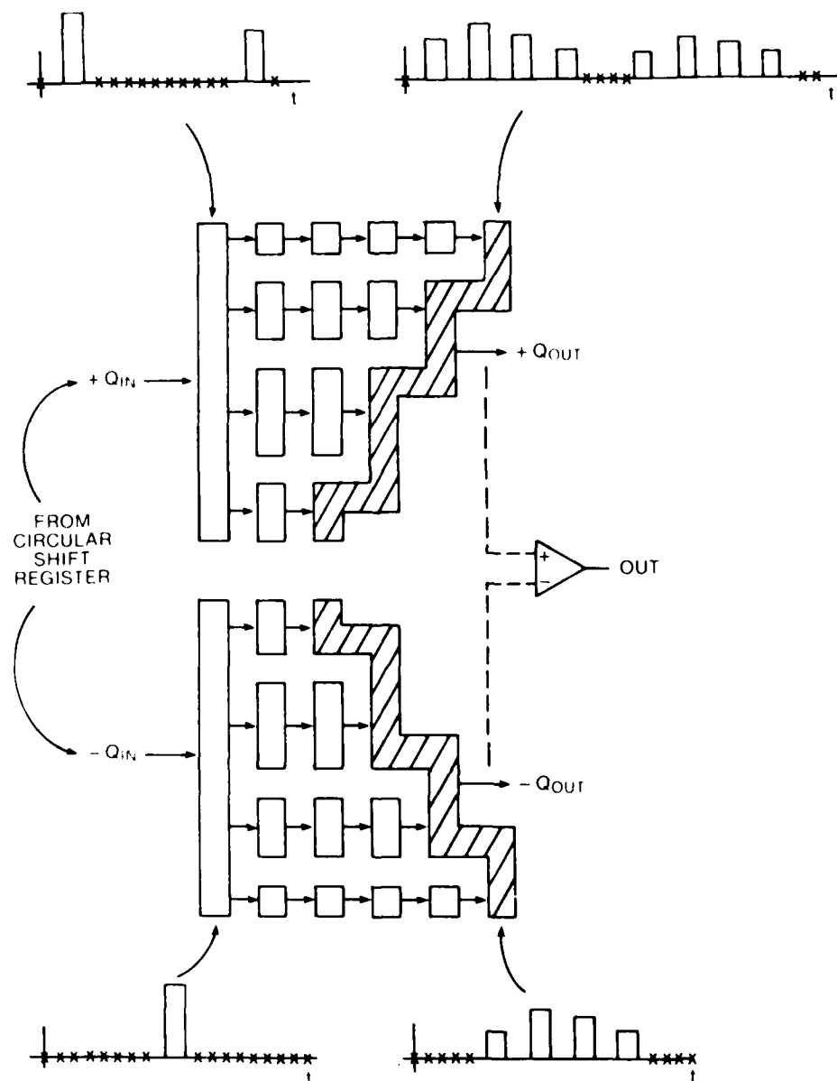
Figure 5.4. Charge domain transversal filter schematic and overall impulse response.
