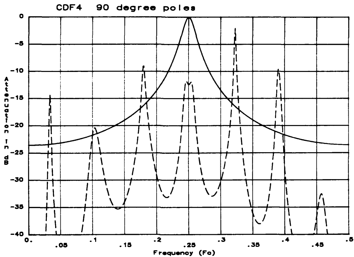
Figure 9.19. Frequency resonance for 89^\circ - 91^\circ pole sections (dashed) and 2 90^\circ pole sections solid.
