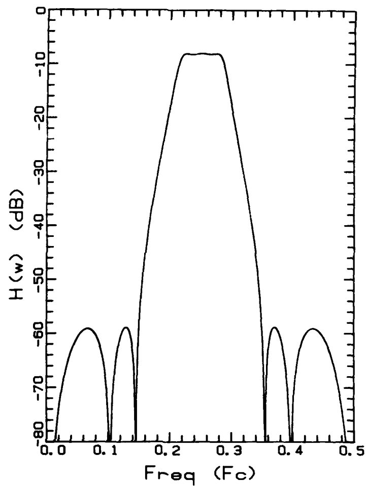
Figure 5.8. Frequency response of a bandpass filter incorporating the pole-grouping modified circular shift register.
