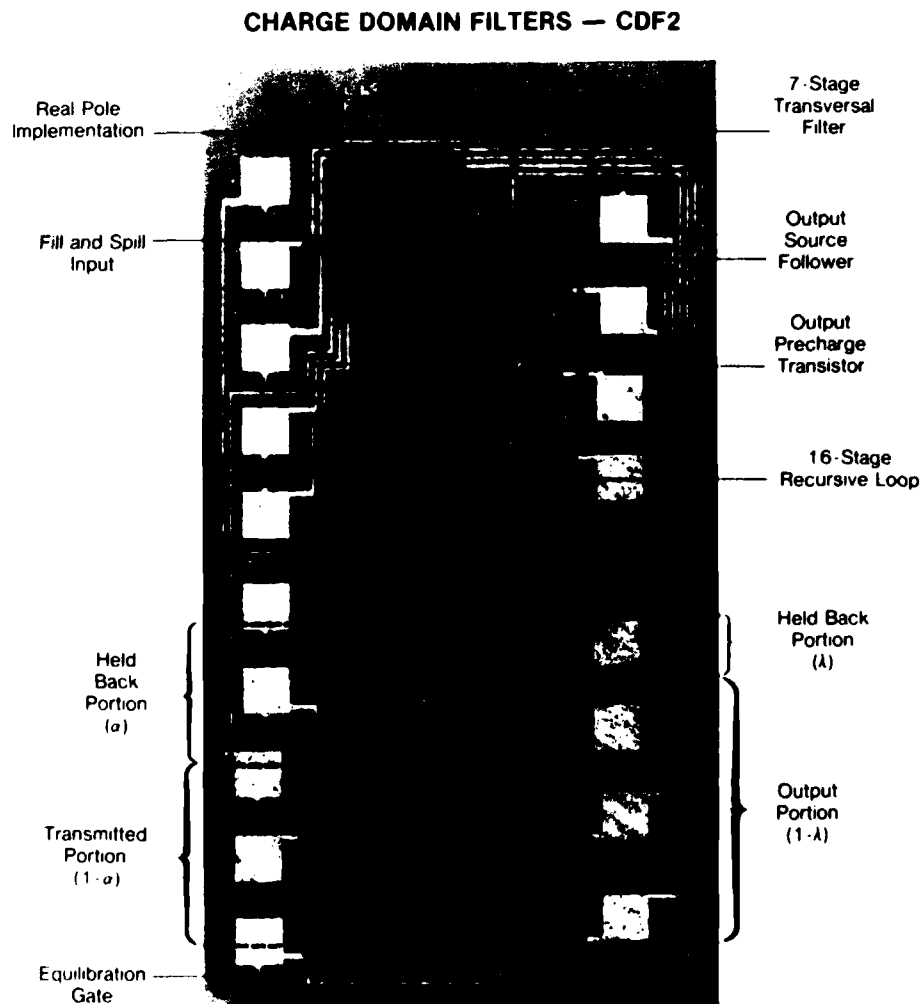
Figure 9.8. CDF2 photomicrograph.
