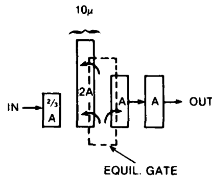
(b) Equilibration technique used for CDF2
