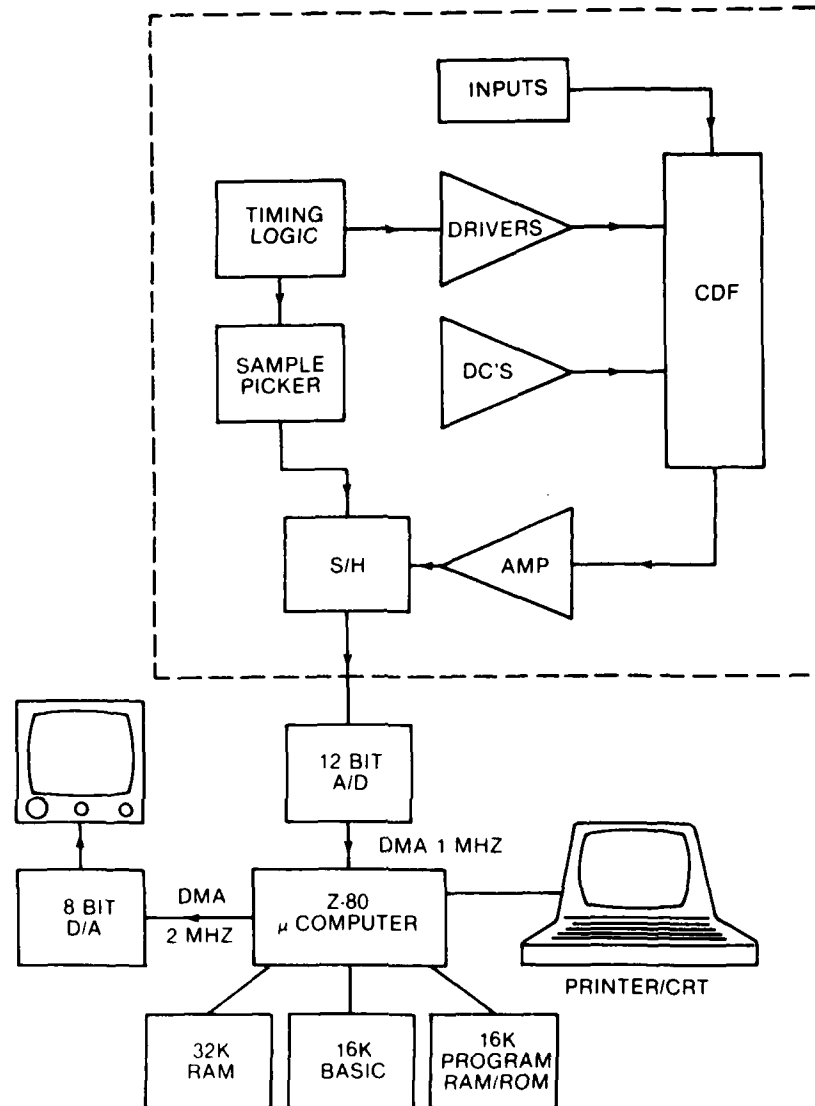
Figure 7.1. Test electronics.
