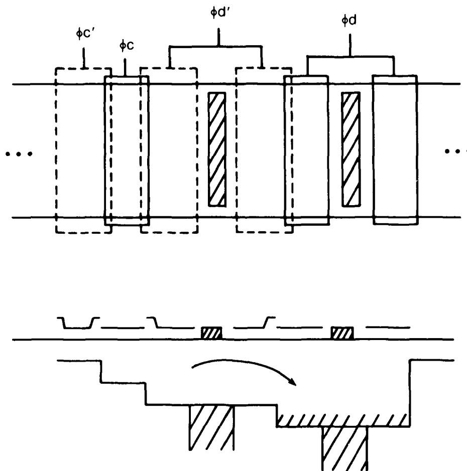
Figure 9.28. CCD structure for enhancing lateral equilibration.
