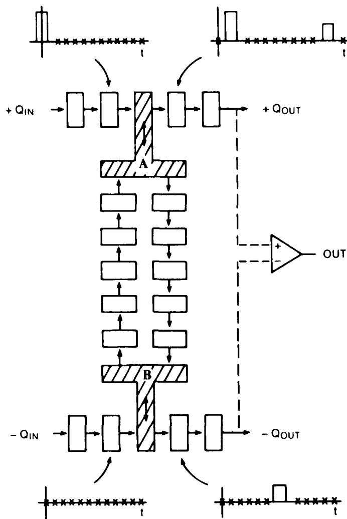
Figure 5.2. Circular shift register schematic showing impulse response.
