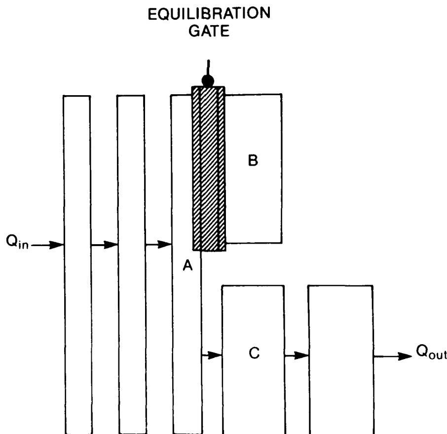
Figure 5.1 Recursive accumulator structure for implementing a real axis pole
