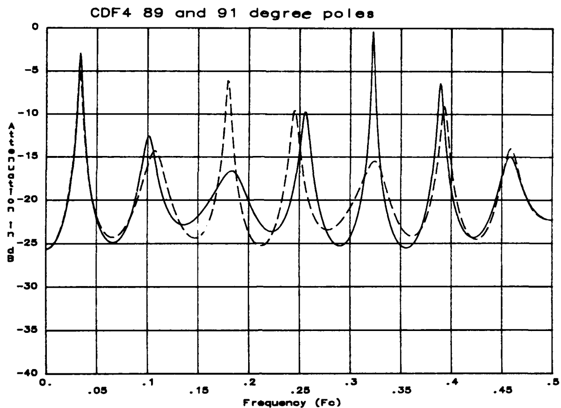
Figure 9.15. Frequency response for 89° pole section (dashed) and 91° pole section (solid).
