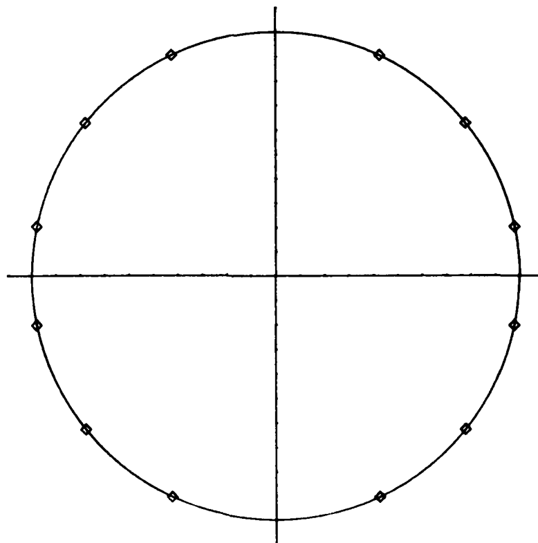
Figure 9.20. Zero locations (diamonds) for transversal filter section.
