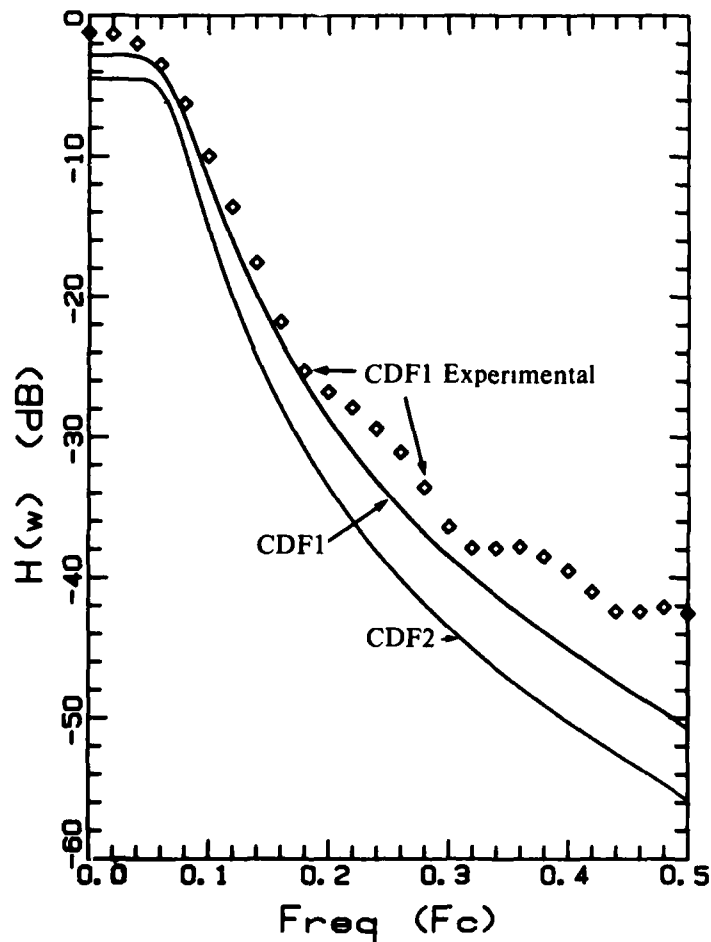
Figure 9.7. Comparison of the frequency response of CDF1 and CDF2.
