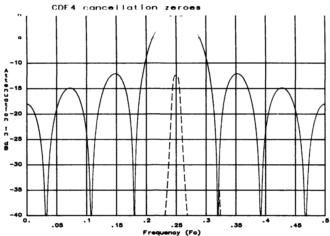
Figure 9.21. Frequency response of 89-91-90-90° pole sections (dashed) and of zero section (solid).
