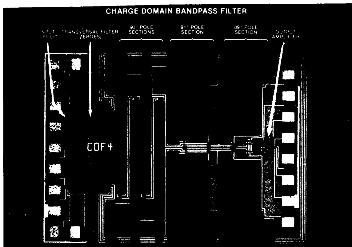
Figure 9.31. CDF4 bandpass filter photomicrograph.
