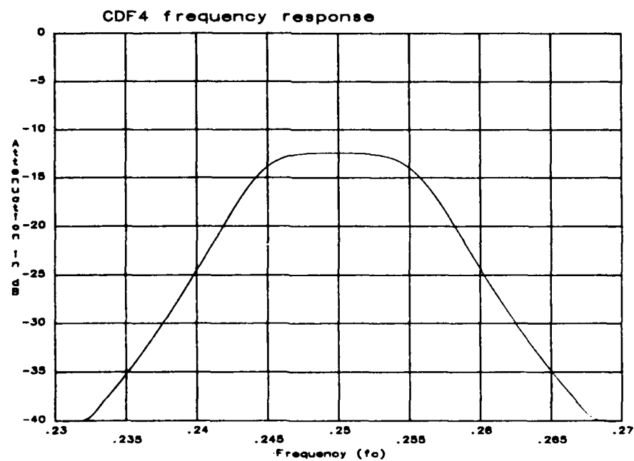
Figure 9.25. Bandpass filter frequency response — expanded view
