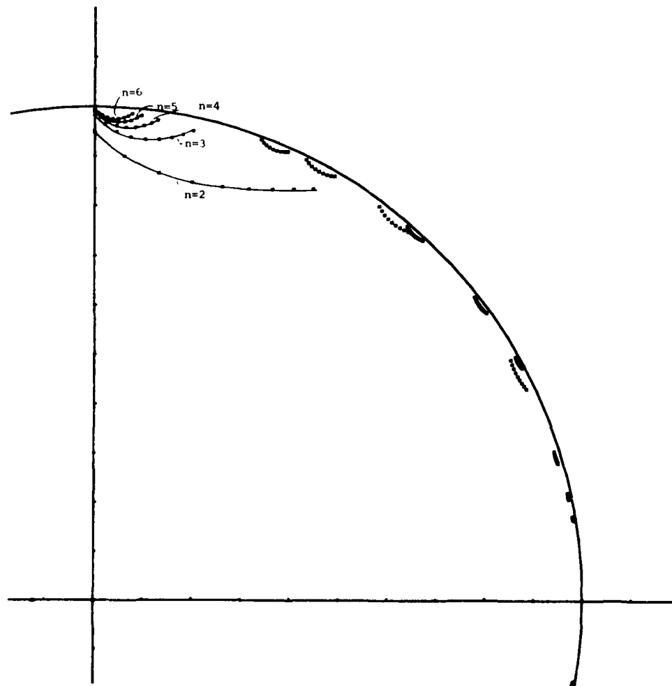
Figure 9.14 Locus of pole locations for various number ( n ) of stages in feedback loop.
