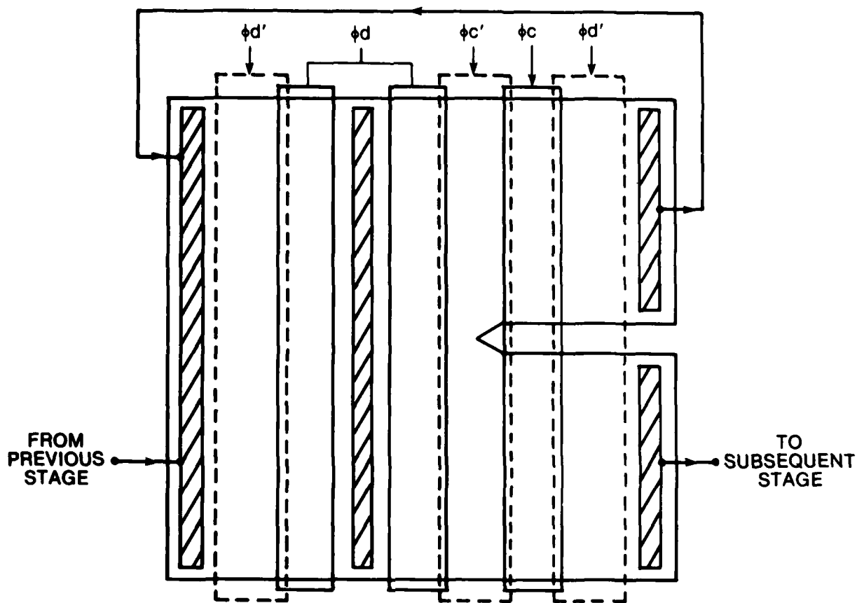
Figure 9.29. Improved single stage feedback structure.
