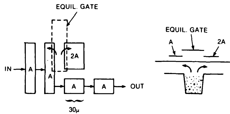
(a) Equilibration technique used for CDF1
