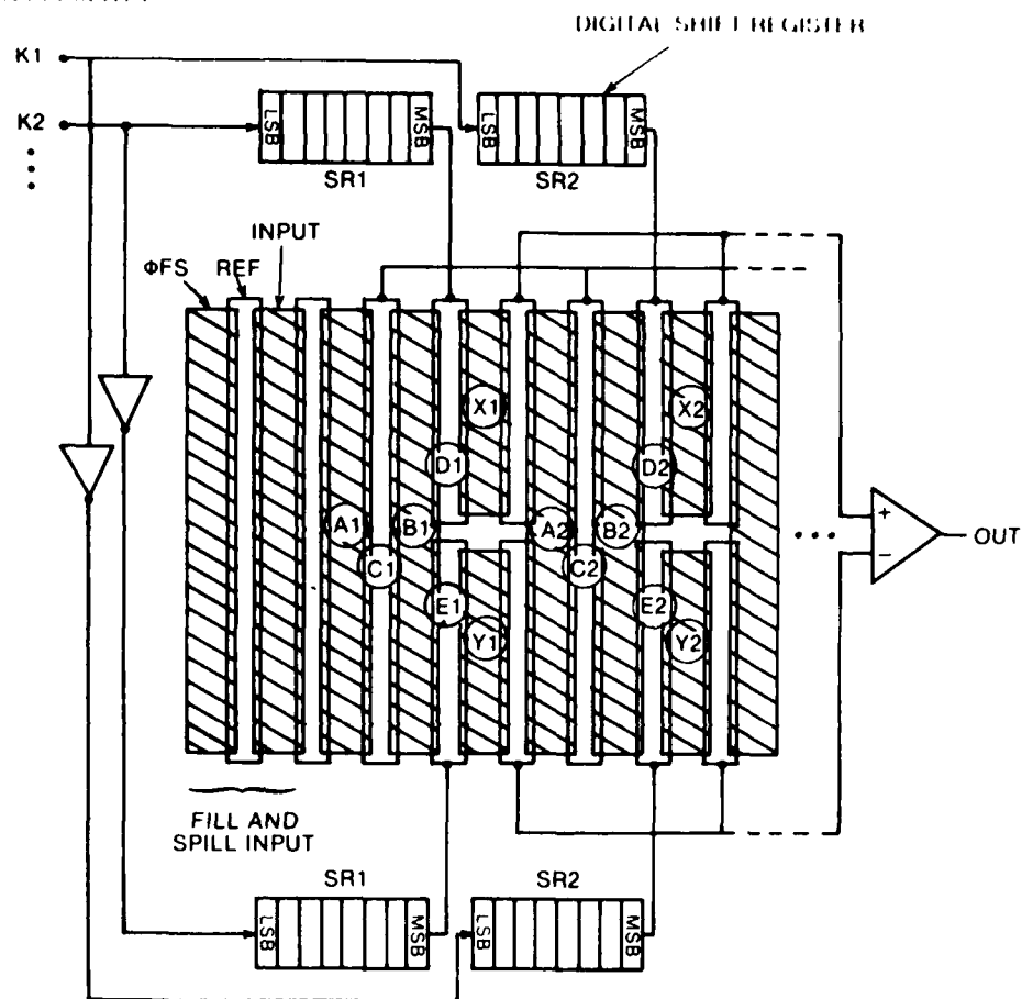
Figure 10.10. Split electrode type programmable transversal filter.
