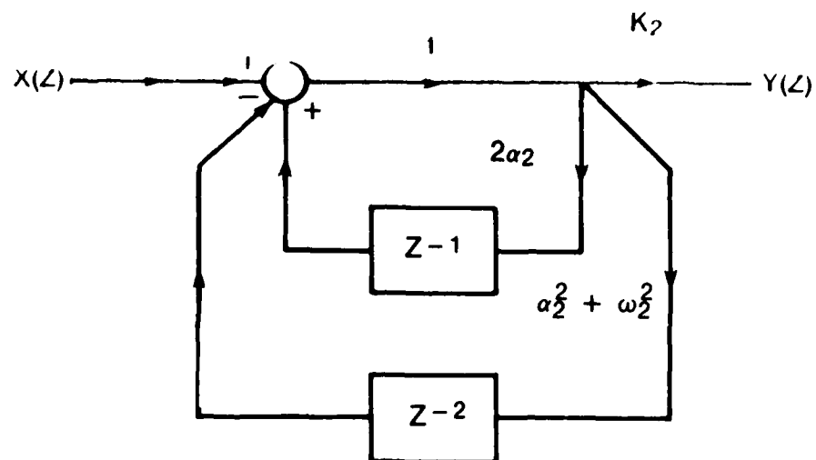
Figure 4.2. Complex pole pair block diagram.
