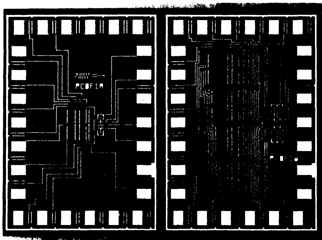
Figure 10.1b. PCDF1A = in-phase sequential splitter PCDF1B = four stage pipe organ filter using sequential splitters.
