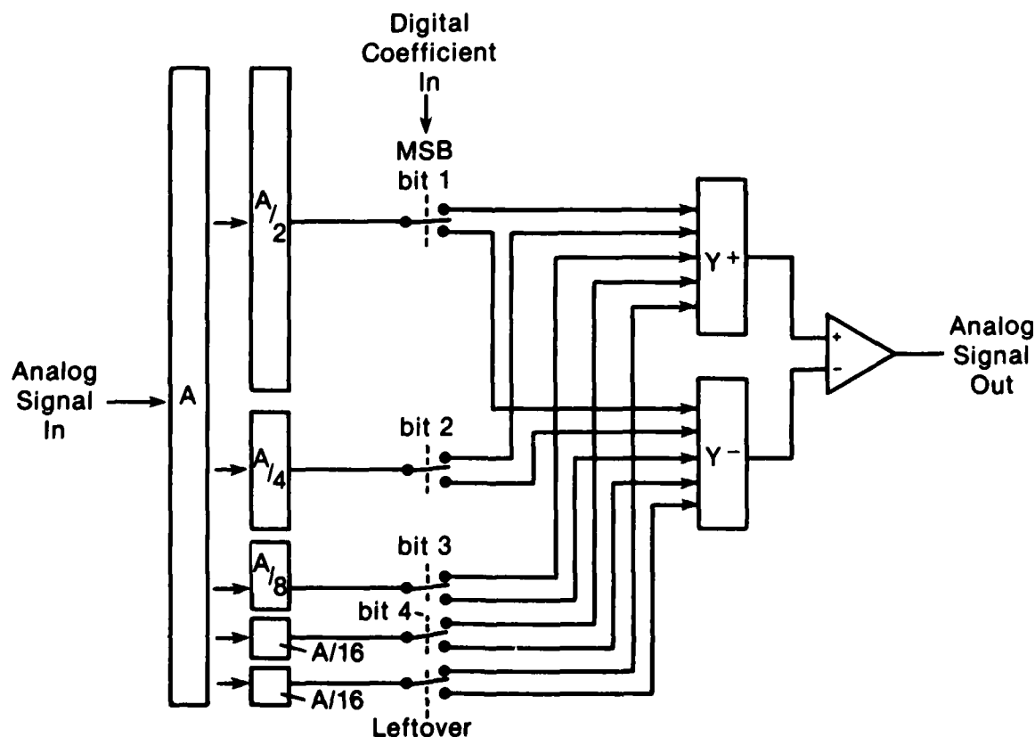
Figure 10.6. Flash charge splitter schematic.
