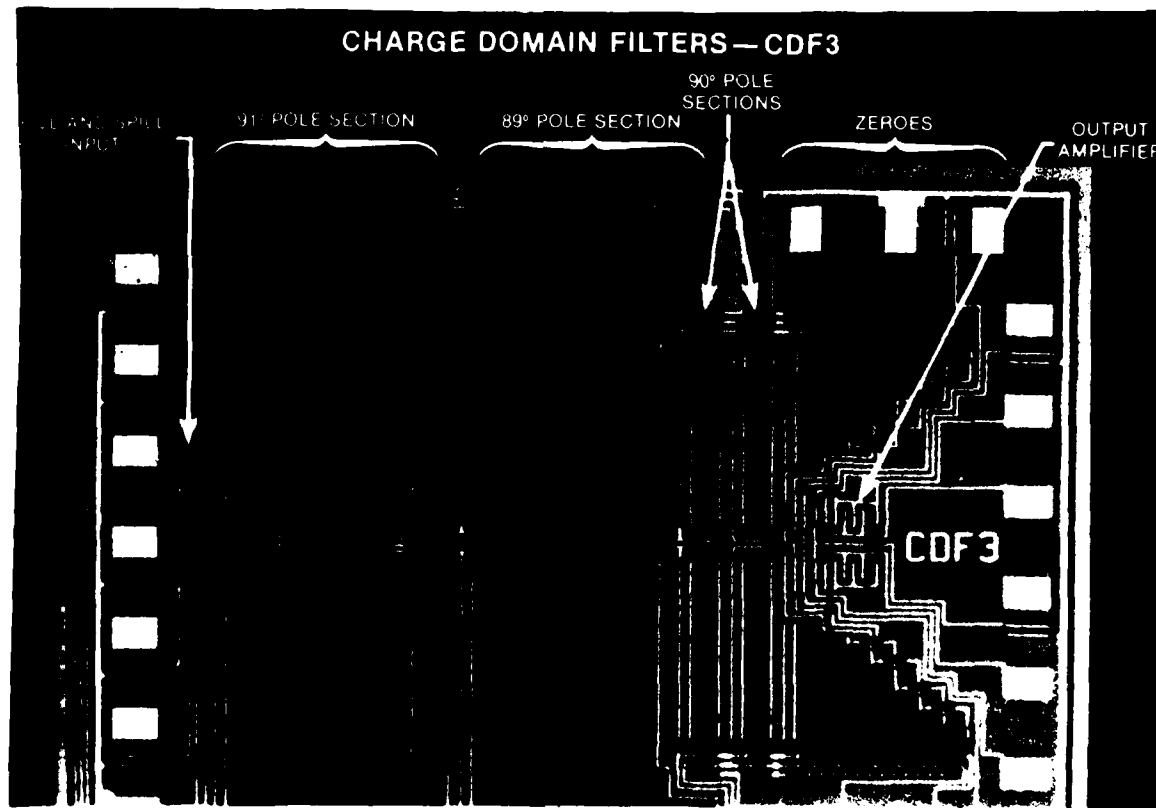
Figure 9.30. Charge domain bandpass filter photomicrograph.
