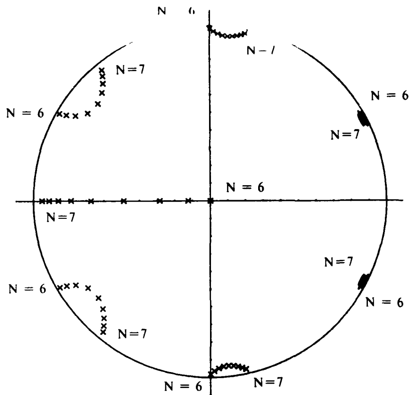
Figure 5.6. Locus of pole locations for 2N = 12 and 2N = 14 stage modified circular shift register.
