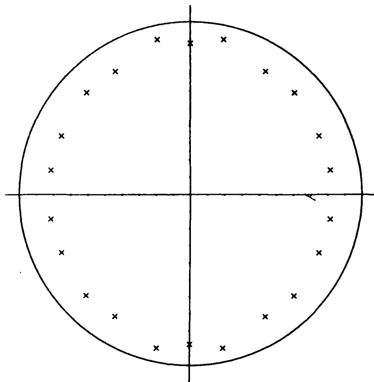
Figure 5.7. Pole-zero diagram showing grouping of poles at the imaginary axis.
