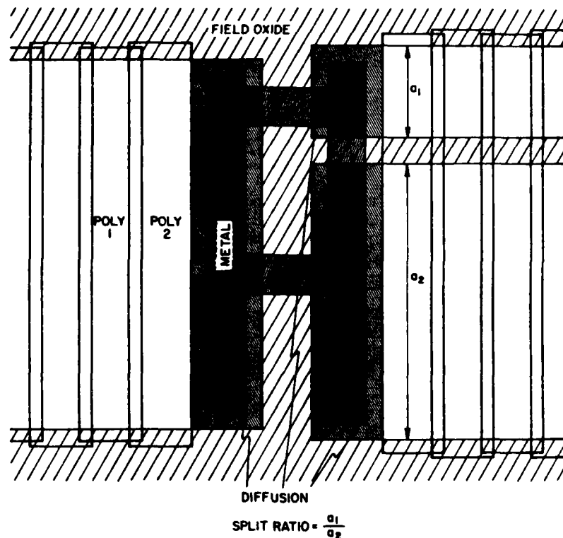
Figure 6.4. Device employing input diffusions for charge splitting.
