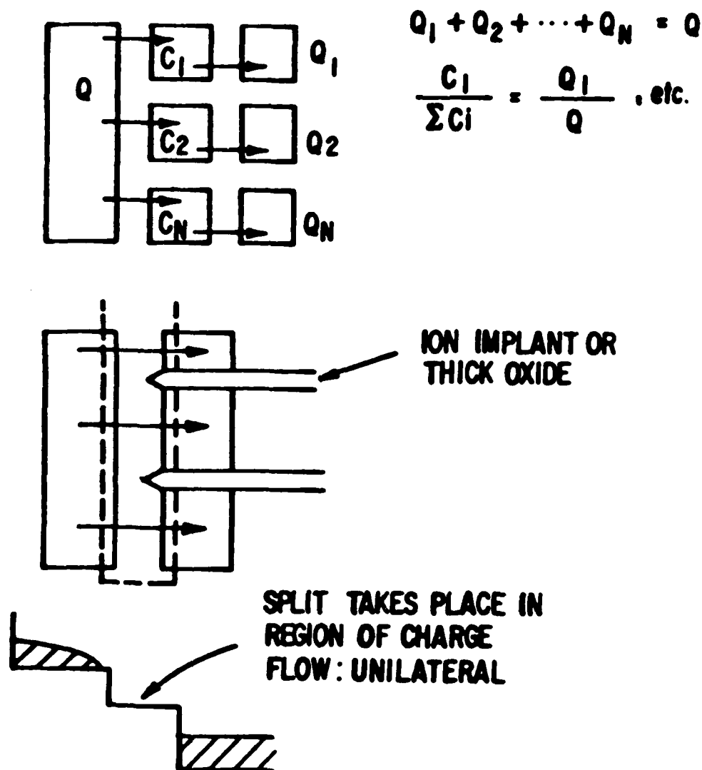
Figure 2.2. Barrier charge packet splitting.
