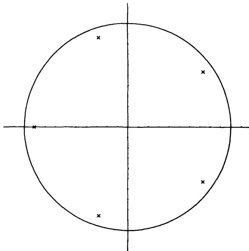
Figure 4.5. Pole locations for an N = 5 stage circular shift register.
