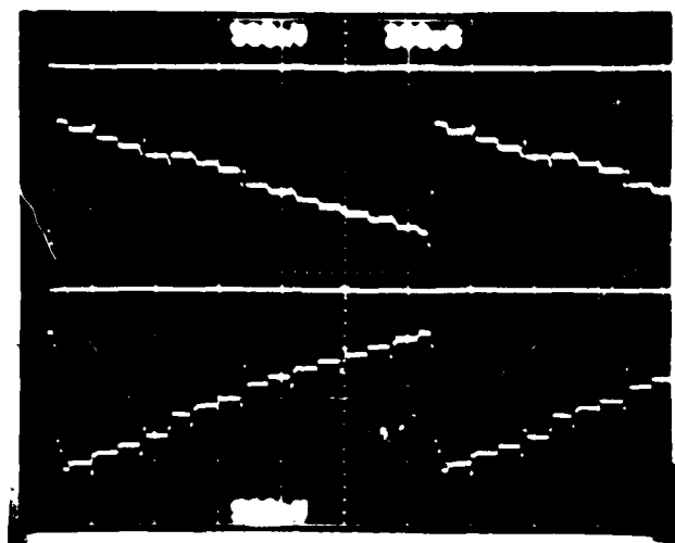
Figure 10.7. Pipelined charge splitter operated as a four-bit MDAC.
