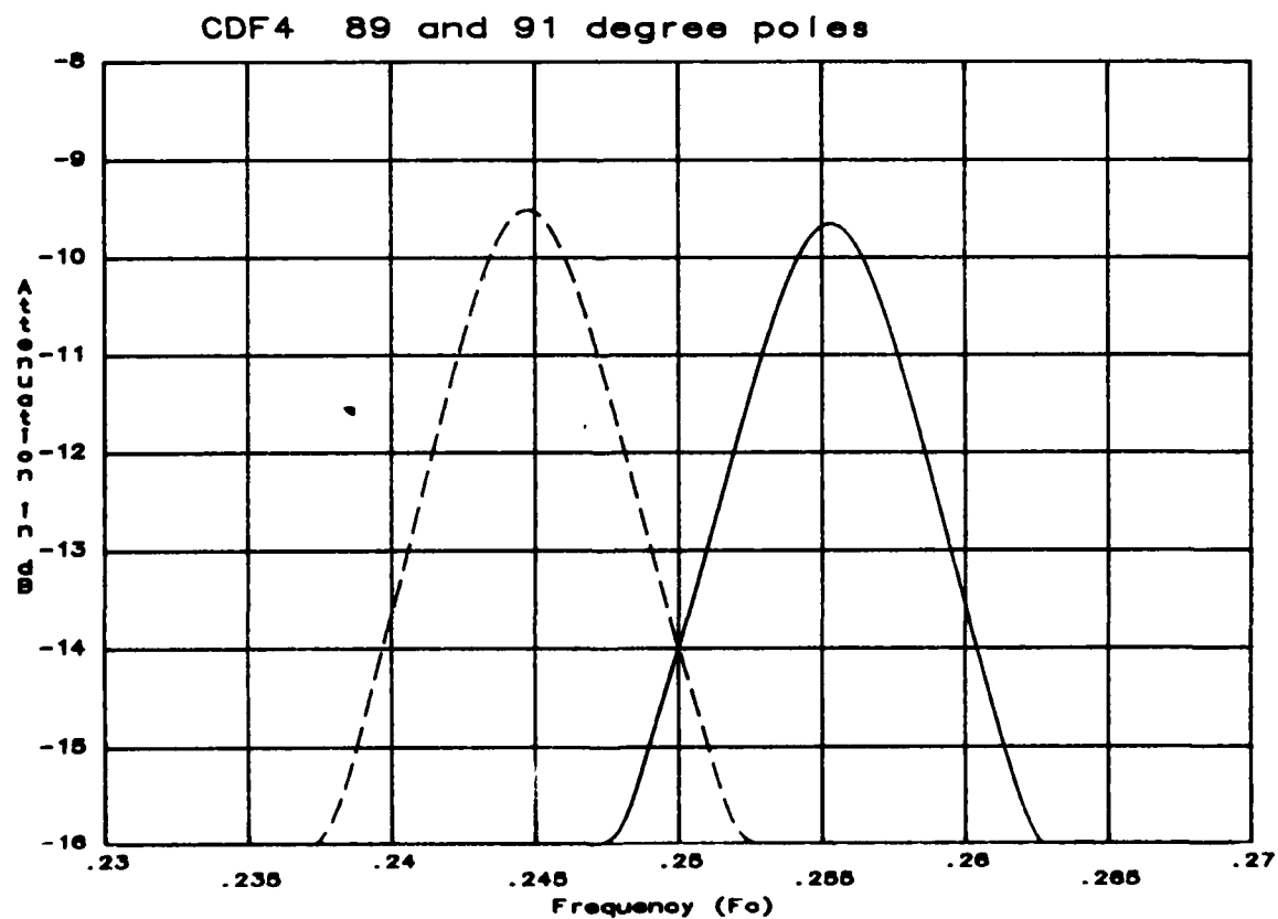
Figure 9.16. Frequency response for 89° and 91° pole sections near center frequency.
