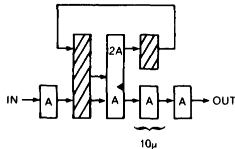
(c) Barrier charge splitting technique used for CDF2
