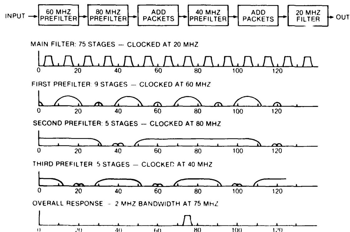
Figure 11.1. 75 MHz filtering utilizing alias bands and small prefilters.
