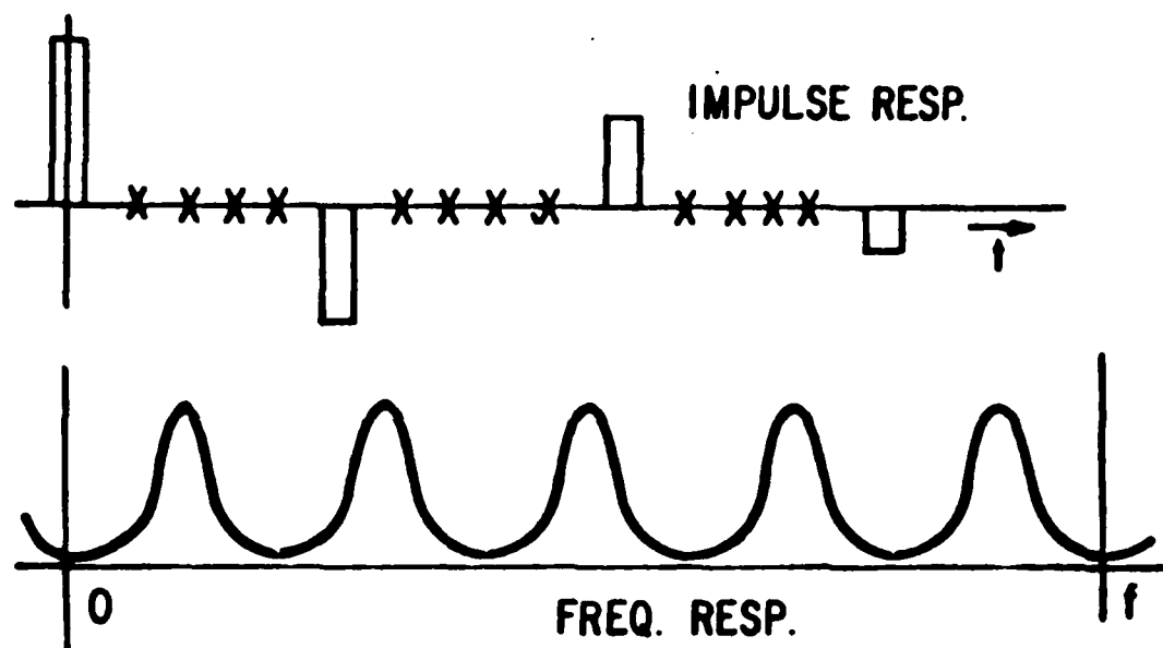
Figure 5.3. Circular shift register impulse and frequency responses.
