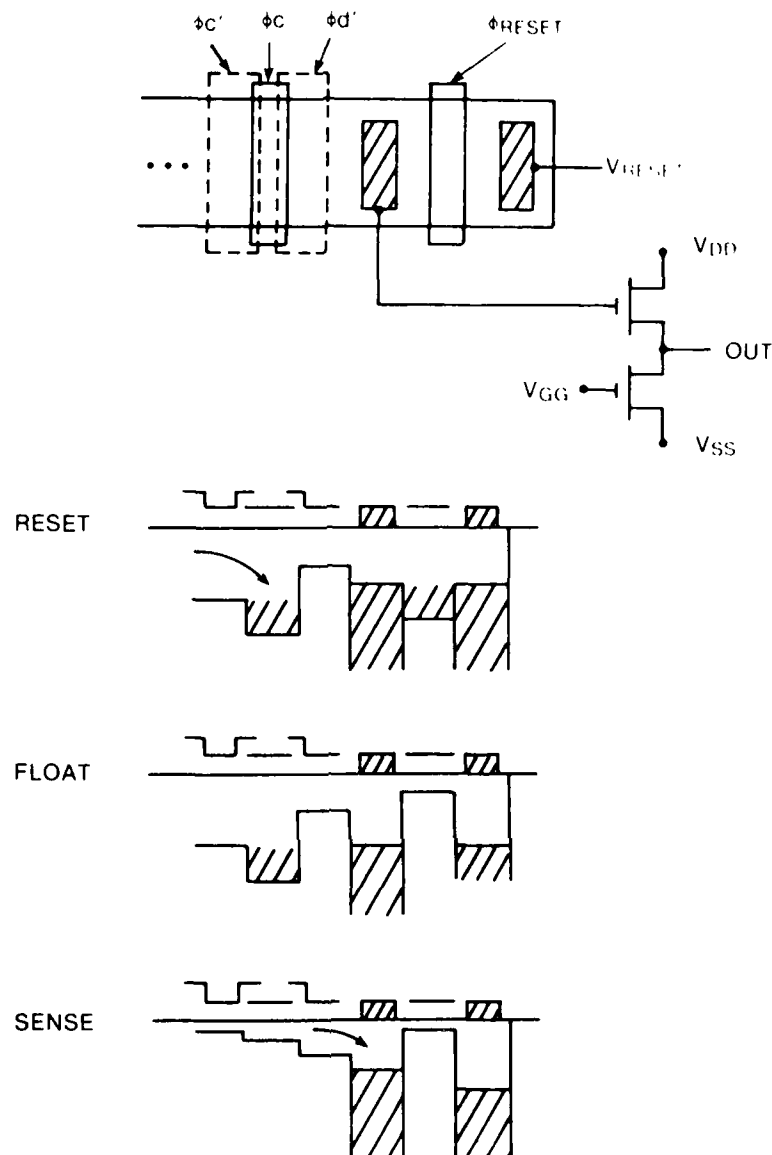
Figure 9.27. Reset and float output circuit.
