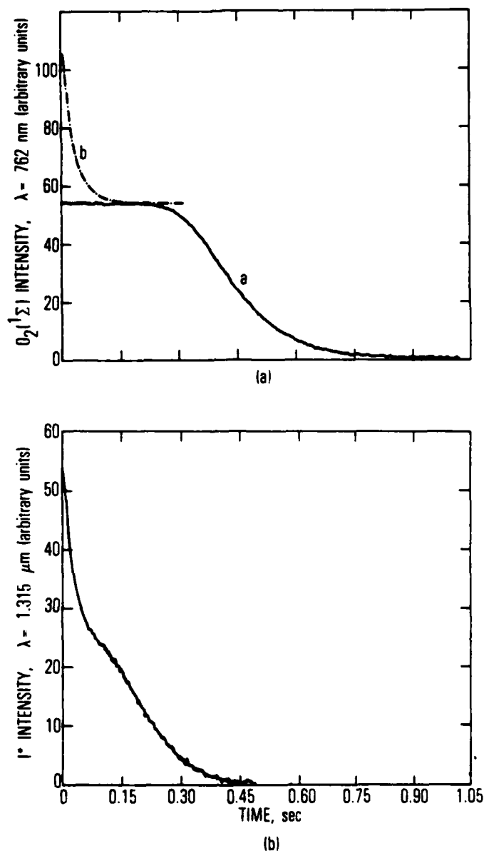
Fig. 7. Diffusion and flow limits on kinetic time scales. (a) — experimental pumpout/axial diffusion curve for O_2(^1\Sigma) [curve (a)]. -.-.- postulated I^* radial diffusion curve for HI photolysis in O_2^* from photolysis volume to cell volume [curve (b)]. (b) Experimental I^* decay in O_2^* at low [HI]. [O_2(^3\Sigma)] = 9.0 \times 10^{16} , [O_2(^1\Delta)] = 7.9 \times 10^{15} , [HI]_0 = 6.4 \times 10^{14}/\text{cm}^3 . Calculated percentage photolysis: 2.2%.
