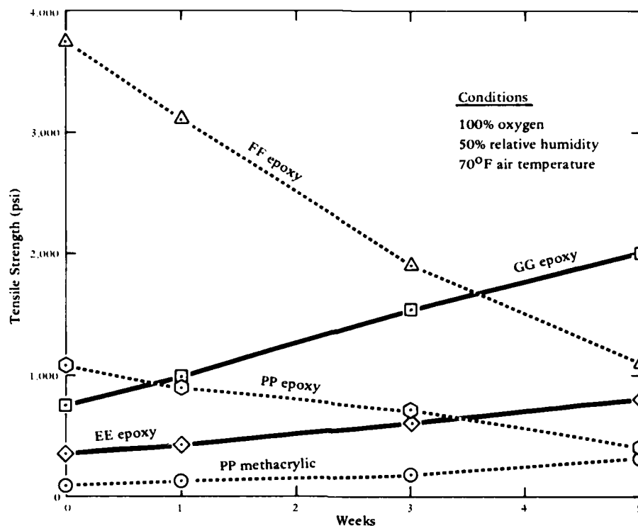
(a) Steel-to-steel.
