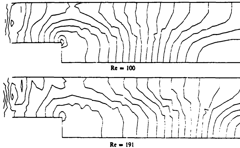
Figure 7.3. Isopressure lines
