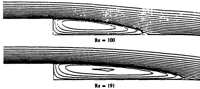
Figure 7.2. Stream lines
