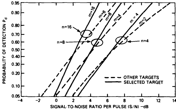
Fig. 7 - Comparison of performance of target of opportunity using fixed sample-size selection for another chosen target to that of random selection for n = 16, 8, \text{ and } 4 , and m = m_{opt} . In all cases k = 1 , the probability of false alarm is 10^{-6} and noncoherent integration is used.
