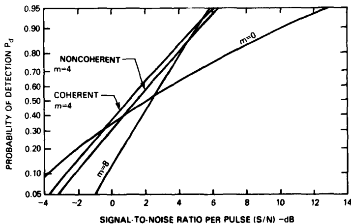
Fig. 2 — Performance characteristics for n = 8 pulses, k = 1 range cells, probability of false alarm of 10^{-6} for the cases of (1) random frequency selection m = 8, (2) fixed frequency selection using coherent integration m = 0, (3) fixed sample size using coherent integration m = m_{opt} = 4, and (4) fixed sample size using noncoherent integration m = m_{opt} = 4.
