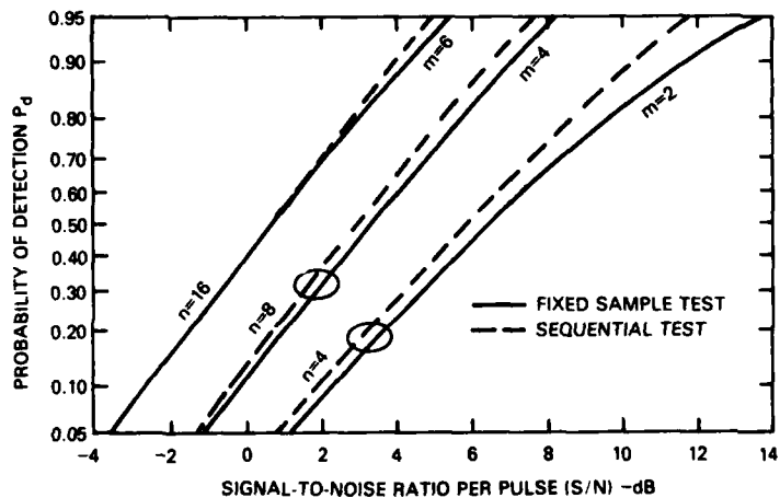
Fig. 8 - Comparison of performance of sequential selection criteria to the fixed sample-size selection criteria for m = m_{opt} using n = 16, 8, \text{ and } 4 . In all cases k = 1 , the probability of false alarm is 10^{-6} and noncoherent integration is used.
