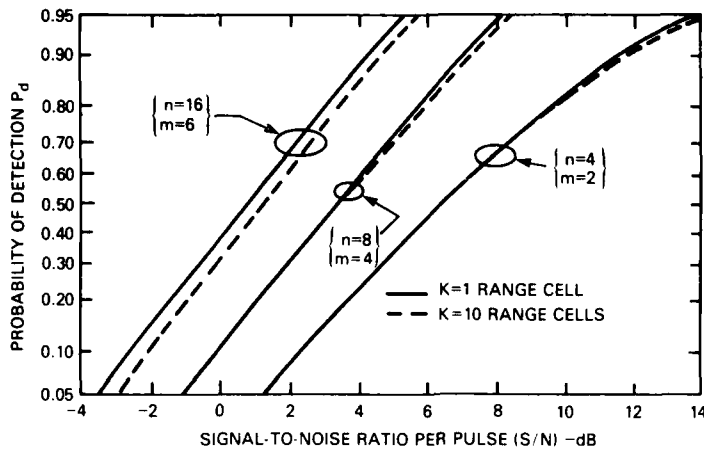
Fig. 5 — Comparison of performance for k = 1 and 10 using n = 16, 8, and 4, and m = m_{opt} . The fixed sample size selection criteria and the noncoherent integration were used for a probability of false alarm of 10^{-6} .
