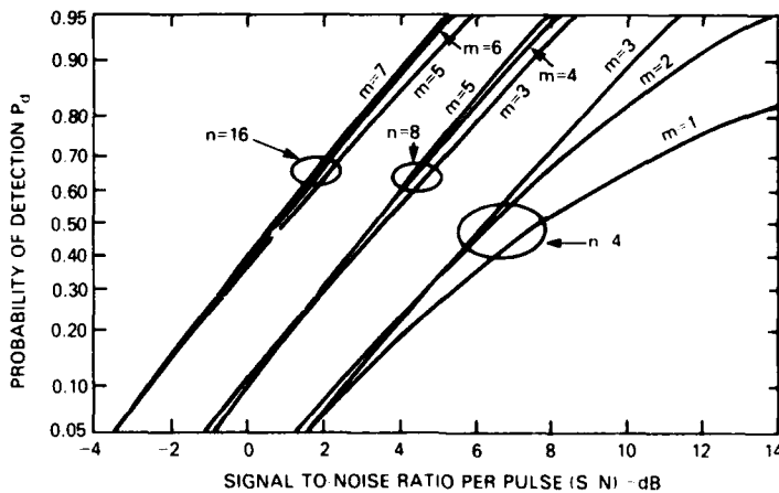
Fig. 4 — Comparison of performance for m = (m_{opt} - 1) , m_0 , and (m_{opt} + 1) , n = 16, 8, \text{ and } 4 . In all cases, the fixed sample size selection criteria and the noncoherent integration were used for k = 1 range cells and a probability of false alarm of 10^{-6} .
