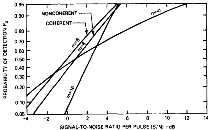
Fig. 1 — Performance characteristics for n = 16 pulses, k = 1 range cells, probability of false alarm of 10^{-6} for the cases of (1) random frequency selection m = 16, (2) fixed frequency selection using coherent integration m = 0, (3) fixed sample size using coherent integration m = m_{opt} = 6, and (4) fixed sample size using noncoherent integration m = m_{opt} = 6.
