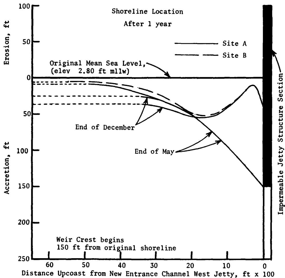
Figure 69. Computer simulation model indication of fillet formation on updrift side of west jetty at proposed new navigation entrance channel locations to Bolsa Chica Bay, California, at the end of May and December after 1 year of operation with a 150-ft sandtight landward section
