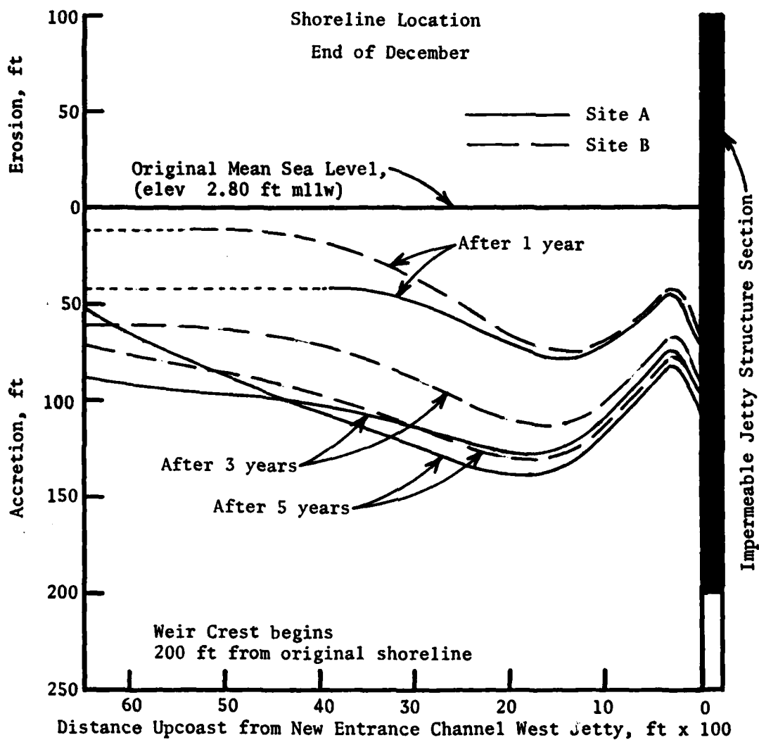
Figure 63. Computer simulation model indication of fillet formation on updrift side of west jetty at proposed new navigation entrance channel locations to Bolsa Chica Bay, California, at the end of December after 1, 3, and 5 years of operation with a 200-ft sandtight landward section
