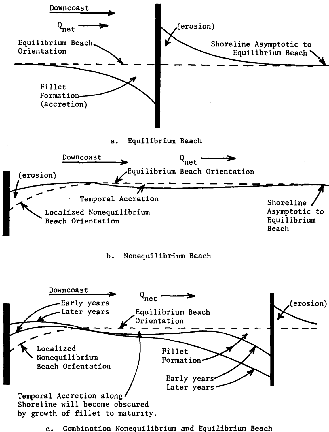
Figure 49. Schematic of shore processes near structures for equilibrium, nonequilibrium, and combination beach orientations
