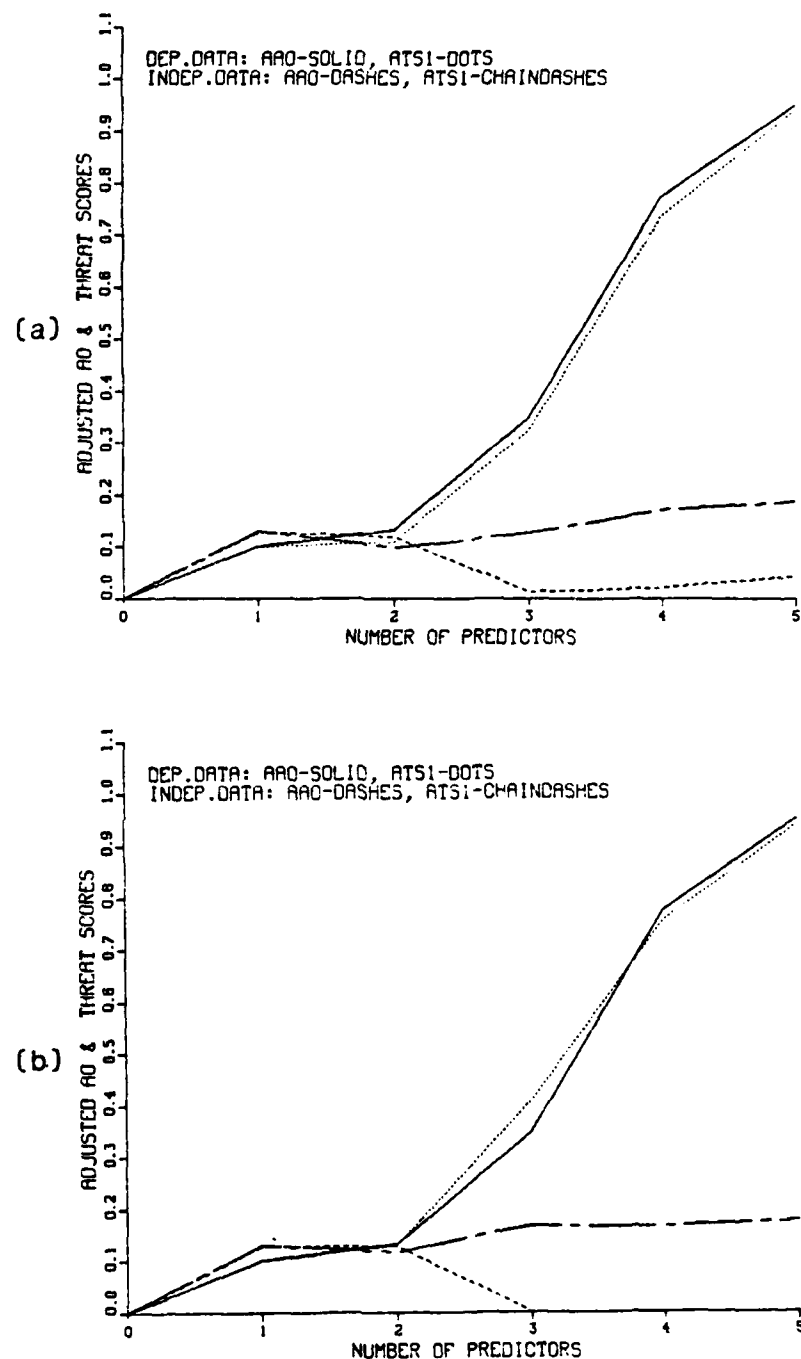
Fig. 10. Contingency table statistics AA0 and ATSl for both dependent and independent North Atlantic Ocean area 3W, 15 May-15 July 1983, data, without linear-regression equations as predictors, as a function of the number of predictors in the model for strategies (a) MAXPROB1 and (b) MAXPROB2. Predictors are SMF, D850, RH, UBLW and ENTRN, each divided into eight EPI's. Negative values are not plotted.
