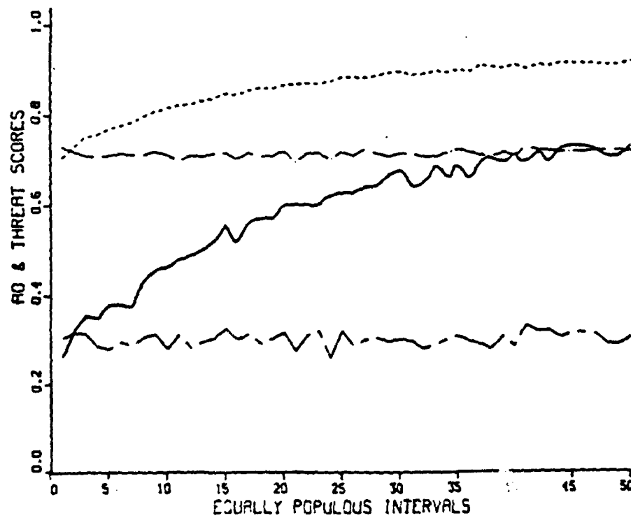
Fig. 3c. Same as Fig. 3a, except for four predictors (SMF(6), RH(3), DUDP(4) and VOR525).
