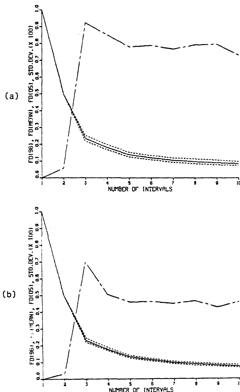
Fig. 4. The behavior of functional dependence (FD) as determined from 100 randomly generated data sets (Preisendorfer, 1983c) for EPI's of two through ten for (a) the North Atlantic Ocean area 3W, 15 May-15 July 1983, dependent data (1526 observations) and (b) the North Pacific Ocean, July 1979, dependent data (3682 observations). Plotted are FD(96) (upper dashed), FD(05), (lower dashed), mean FD (solid) and standard deviation (x 100) (chaindashes)
