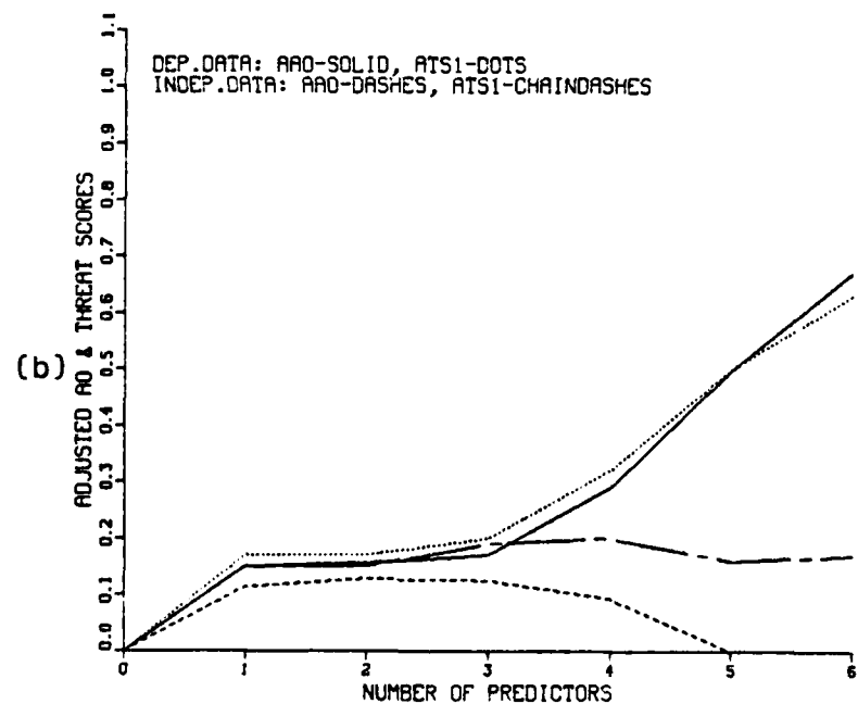
Fig. 6. Contingency table statistics AA0 and ATS1 for both dependent and independent North Pacific Ocean, July 1979, data as a function of the number of predictors in the model for strategies (a) MAXPROB1 and (b) MAXPROB2. Predictors are EHF, DDWW, H510, THF and CLIMO, each divided into five EPI's. Negative values are not plotted.
