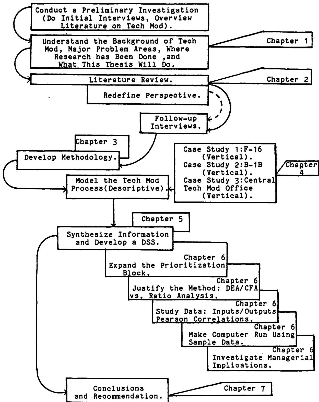
Figure 3.1. Research Methodology
