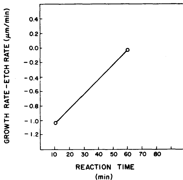
Figure 4. Net Growth Rates as a Function of Reaction Time. Hydrogen chloride partial pressure in the mixing zone, 1.9 \times 10^{-3} atm; HCl (source) partial pressure, 2.3 \times 10^{-3} atm; AsH 3 partial pressure, 1.0 \times 10^{-2} atm; total H 2 flow rate, 980 cc/min. Source alloy composition, 88.2 mole percent In and 11.8 mole percent Ga. Substrate temp = 675°C; mixing temp = 850°C; and source temp = 800°C
