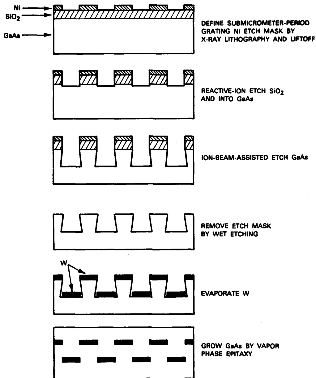
Figure 4-1. Self-aligned dual-grating GaAs permeable-base transistor fabrication sequence.
