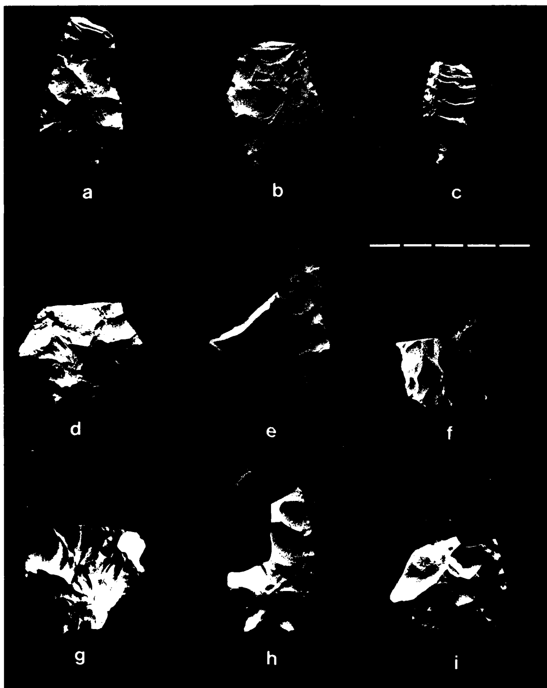
Figure 10.32. Blade fracture: a-c, impact; d, transverse; e, oblique; f-g, irregular; h-i, thermal. Scale in cm.
