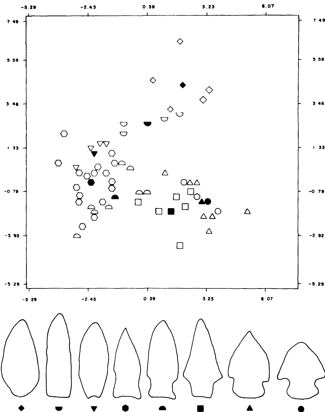
Figure 11.2. Discriminant plots of measured point types. Solid figures denote group centroids.
