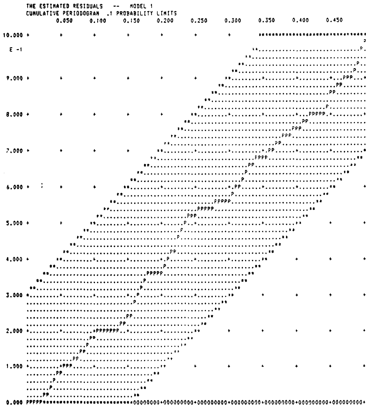
Figure 33. Cumulative Periodogram - Transfer Function Residuals
