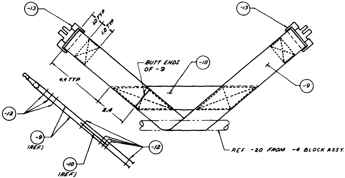
-7 LAP BELT STRAP ASSY. (1 REQD)
