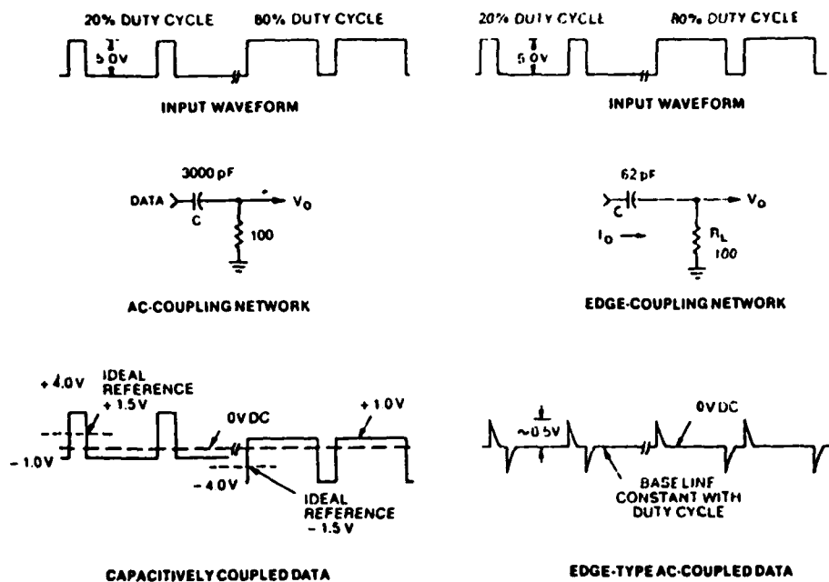
Figure 9(a). Tolerance of duty cycle variations
