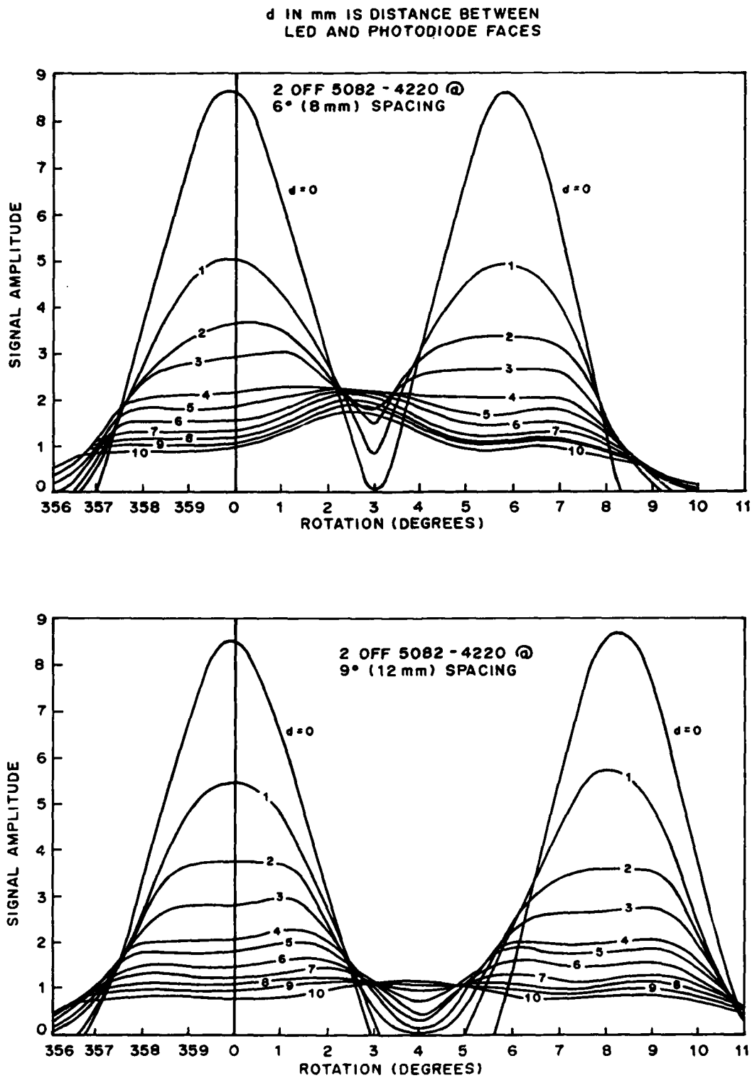
Figure 2. Effect of increasing separation between one IRED and two photodiodes
