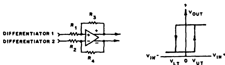
Figure 9(c). Differential comparator as amplitude detector with hysteresis
