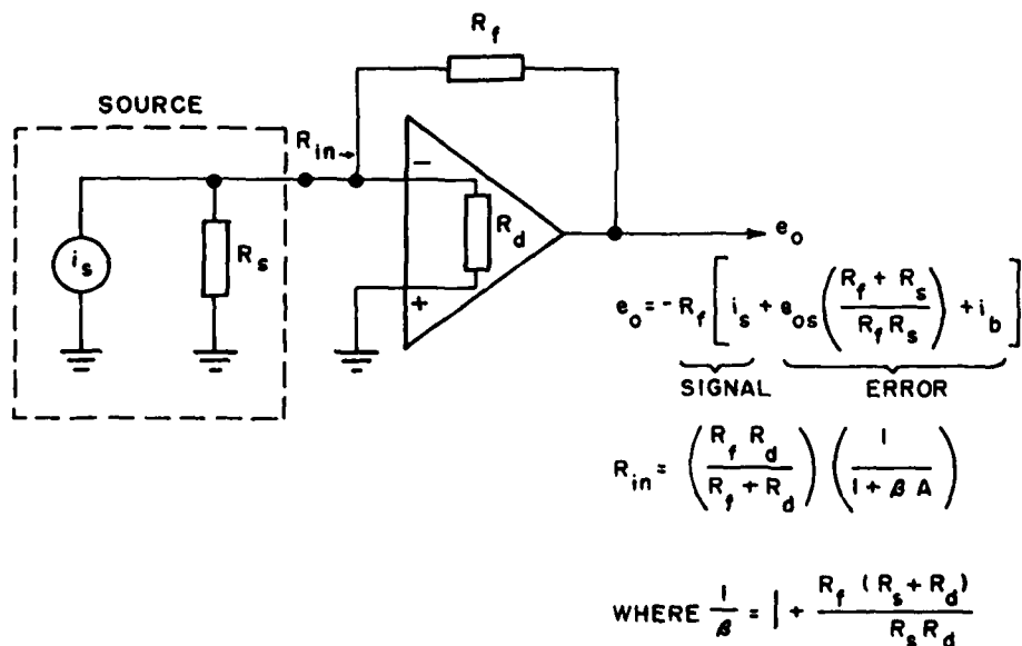
Figure 8(b). High input impedance amplifier
