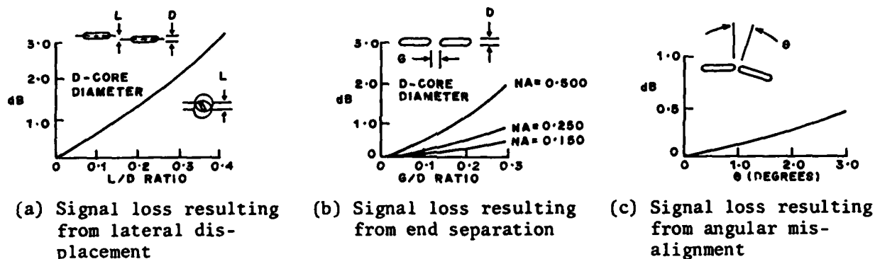
Figure 6. Light losses due to alignment problems
