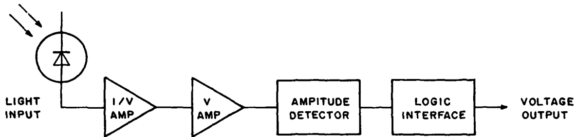
Figure 8(a). Block diagram of receiver
