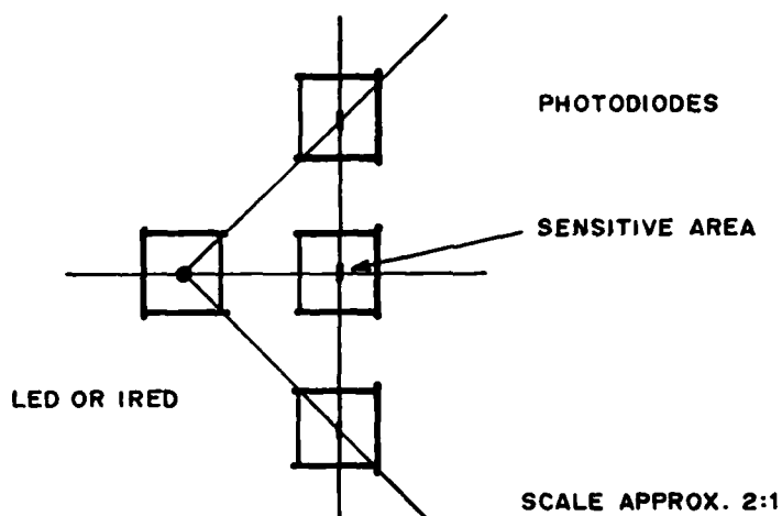
Figure 1. Simplified LED to photodiode relationship
