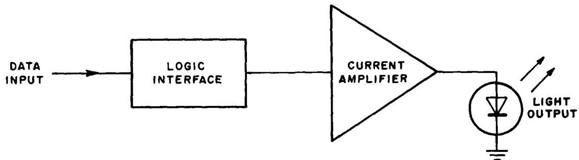
Figure 7(a). Block diagram of transmitter
