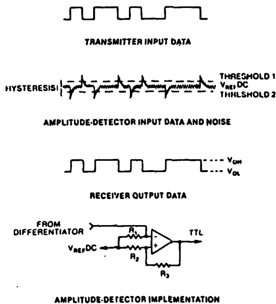
Figure 9(b). Amplitude detector thresholds
