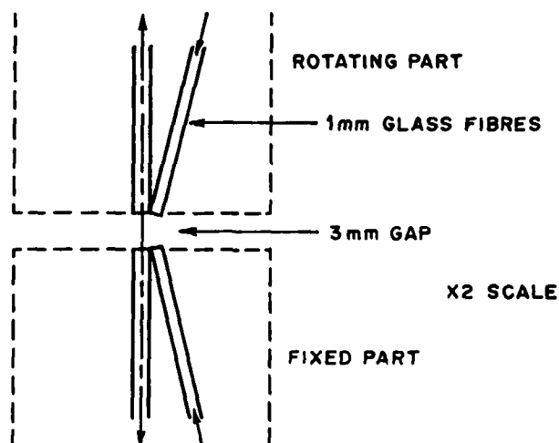
Figure 12. Optical-fibre rotating coupling
