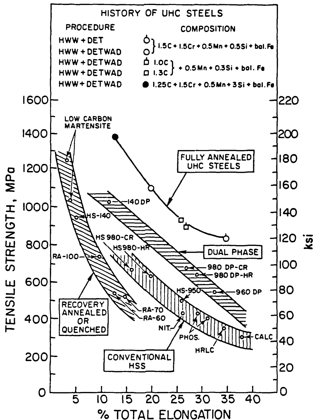
Figure 6. The tensile strength and percent elongation to fracture of UHC steels at room temperature is compared with mild steels, high strength steels and dual phase steels.
