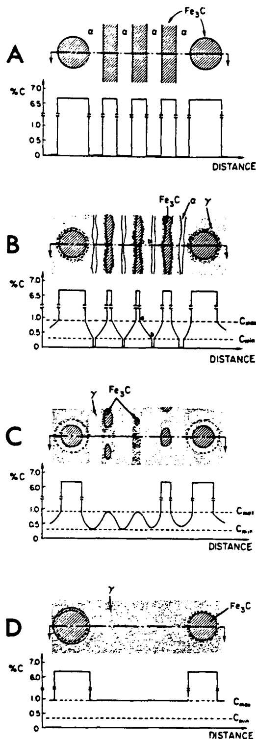
Figure 4. Schematic illustrations of the stages during austenitizing of a UHC steel after Hot and Warm Working (HWW). A carbon concentration profile for each stage is also presented. A, initial HWW structure consisting of spheroidized proeutectoid cementite and pearlite. B, incompletely austenitized structure consisting of austenite with a non-uniform carbon concentration, untransformed ferrite and cementite. C, a microstructure just after complete austenitizing, consisting of austenite with non-uniform carbon concentration and (proeutectoid) cementite particles. D, microstructure after long-time austenitizing consisting of austenite with a uniform carbon concentration and large particle proeutectoid cementite.
