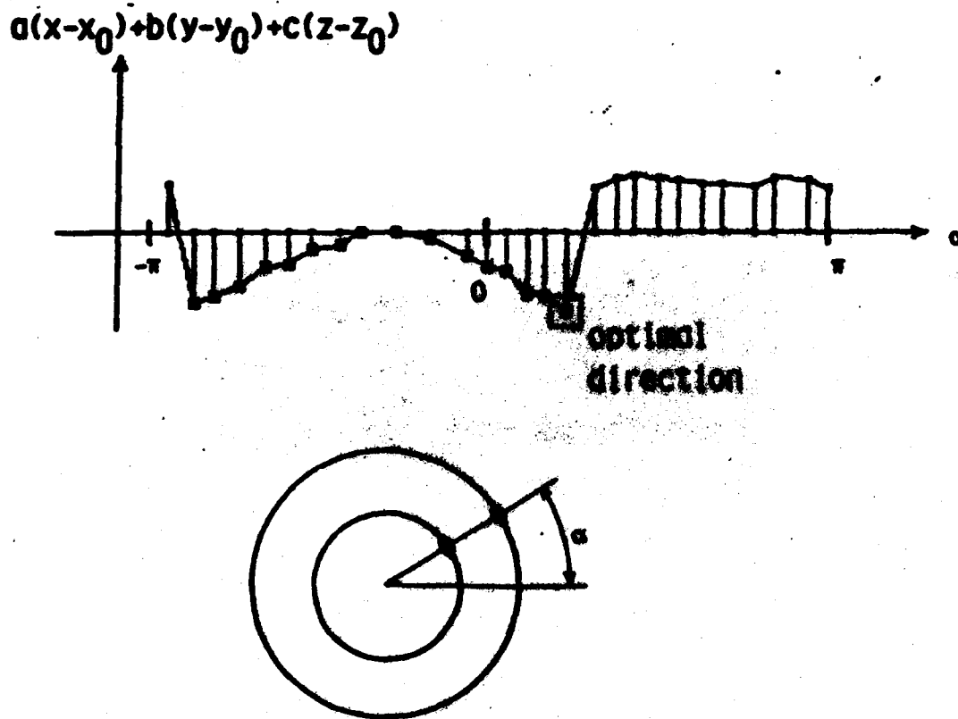
Figure 21. Profile of highest points over the rectangular area of the gripper work space, plotted as a function of rotation around the center of the doughnut
