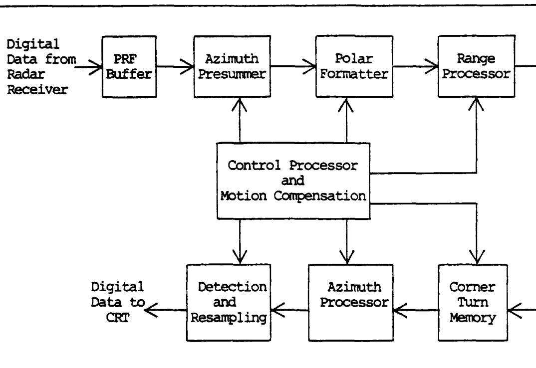
Figure 3. SAR Image Processing Functional Design (5:31)
