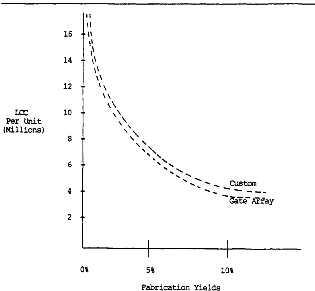
Figure 8. LCC of SAR Processor as a Function of Overall Fabrication Yields
